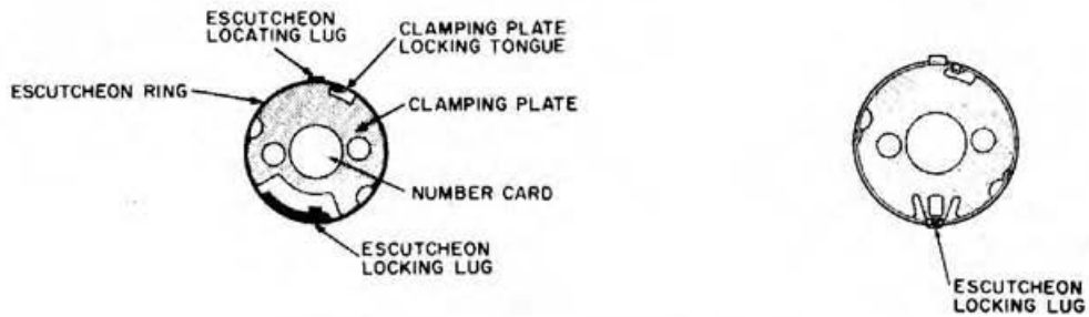
Figure 6. Escutcheon Disassembly.
