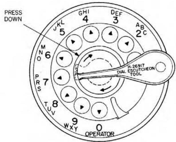
Figure 5b. Installation.
