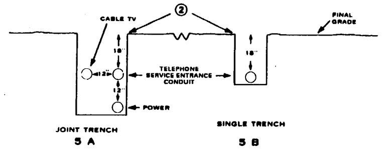
FIG 3 TYPICAL TRENCH CROSS SECTION
