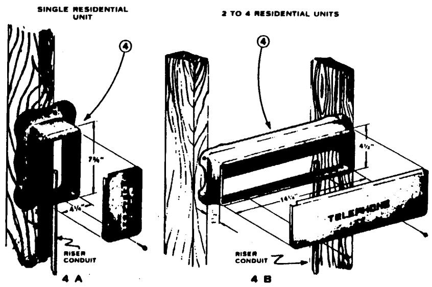
FIG 2 WEATHER PROOF ENCLOSURE
