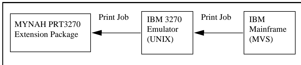
Figure 13-1. MYNAH PRT3270 Interactions
