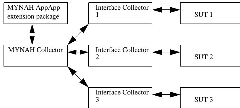
Figure 11-1. MYNAH General AppApp Interactions
