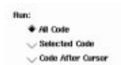
Figure 3-9. Radio Buttons
