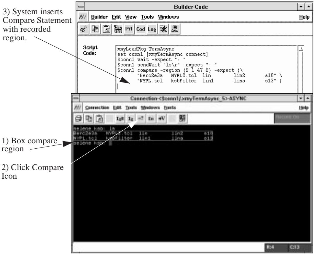
Figure 12-30. Capturing Compare Regions and Inserting Them in the Code View.
