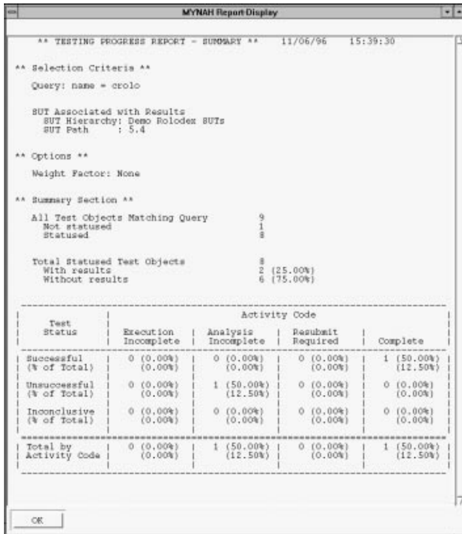
Figure 14-11. Testing Progress Report Window Output
