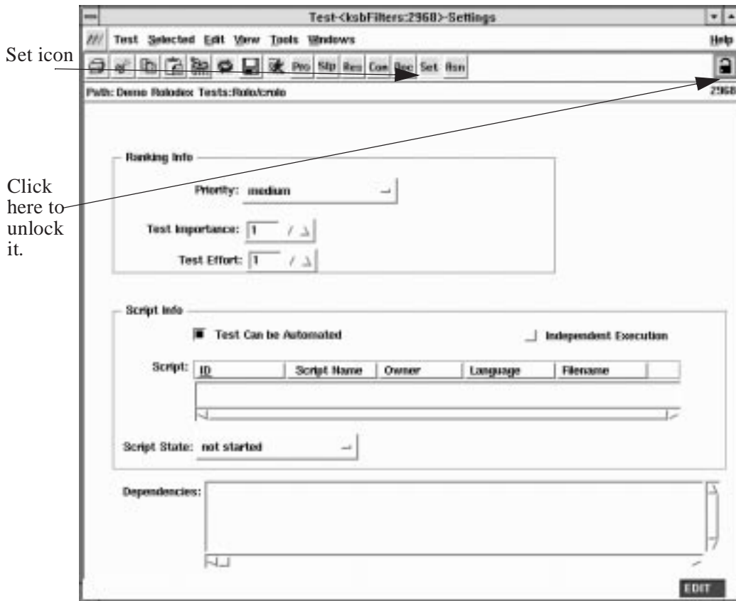
Figure 2-39. ksbFilters Test Setting View
