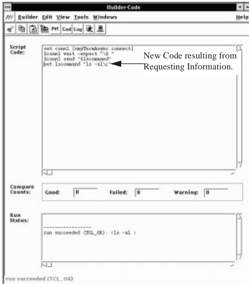
Figure 12-36. Code View with Expression
