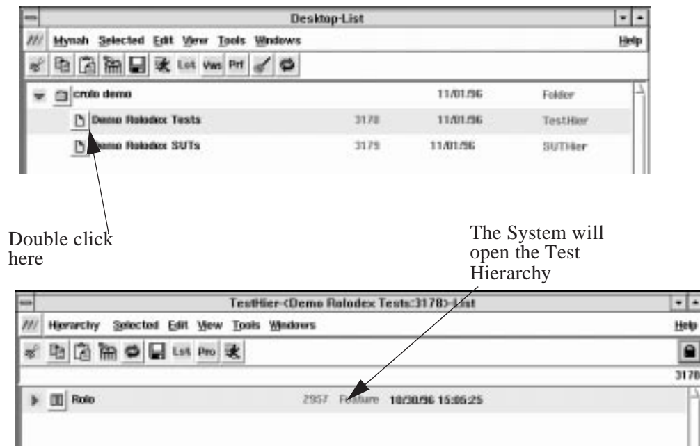
Figure 2-13. Opening a Test Hierarchy
