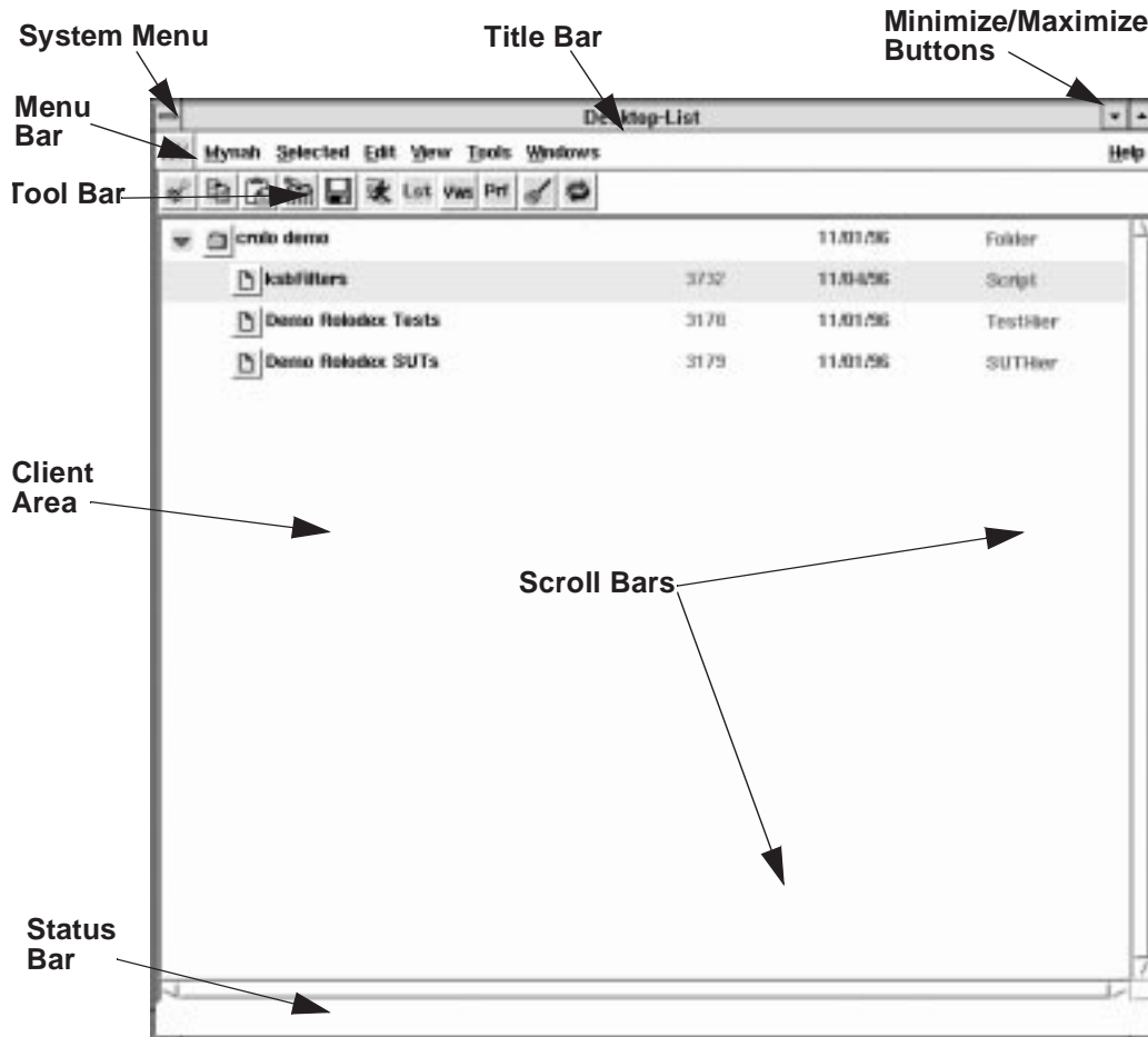
Figure 3-2. MYNAH Desktop (List View)
