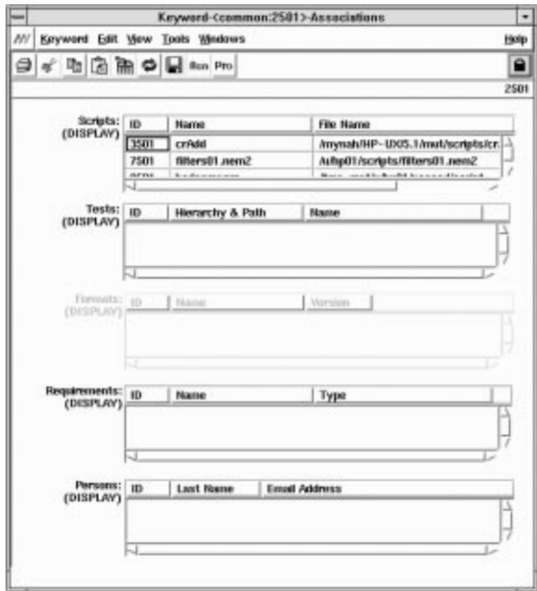
Figure 11-5. Example Associations View
