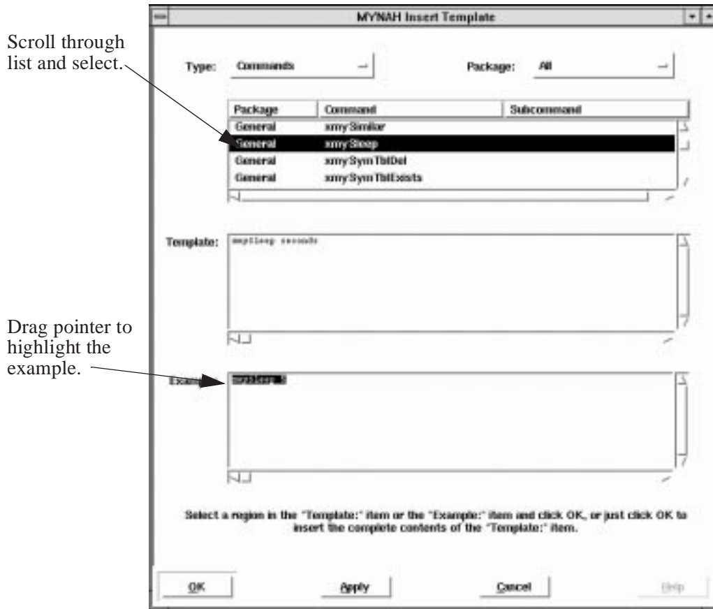
Figure 2-29. Selected Template and Example
