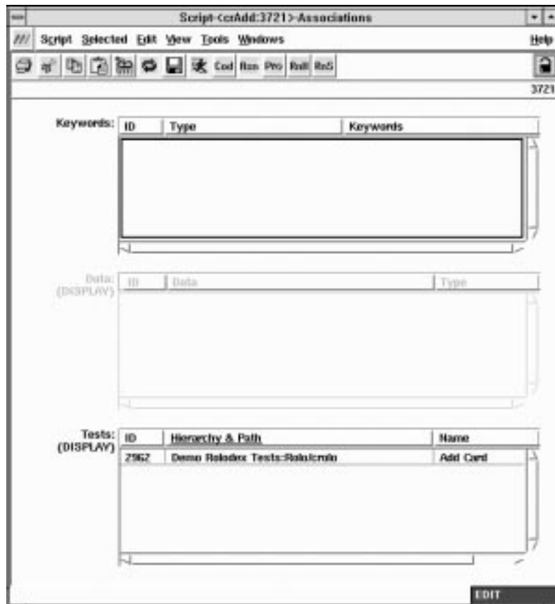
Figure 10-3. Script Object Association View.
