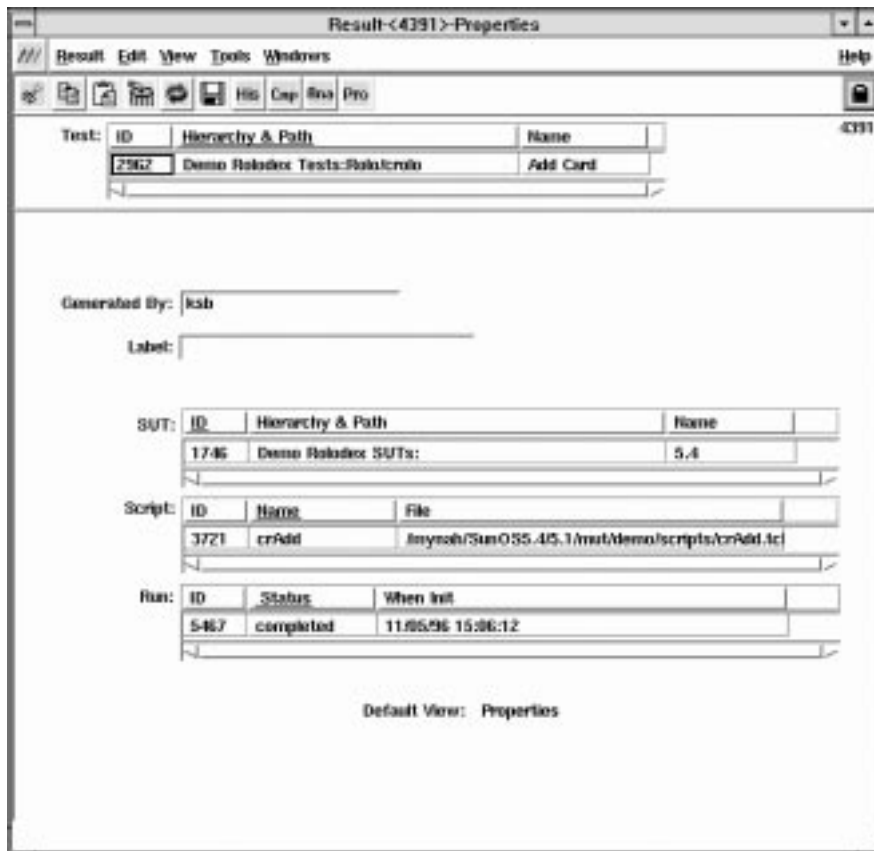
Figure 14-1. Result Object Properties View.
