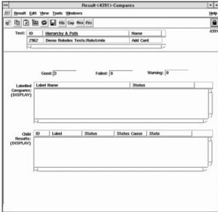
Figure 14-2. Compares View.
