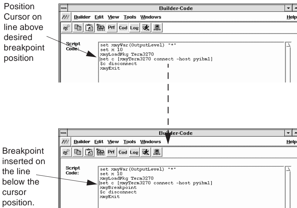
Figure 12-18. Inserting Breakpoints
