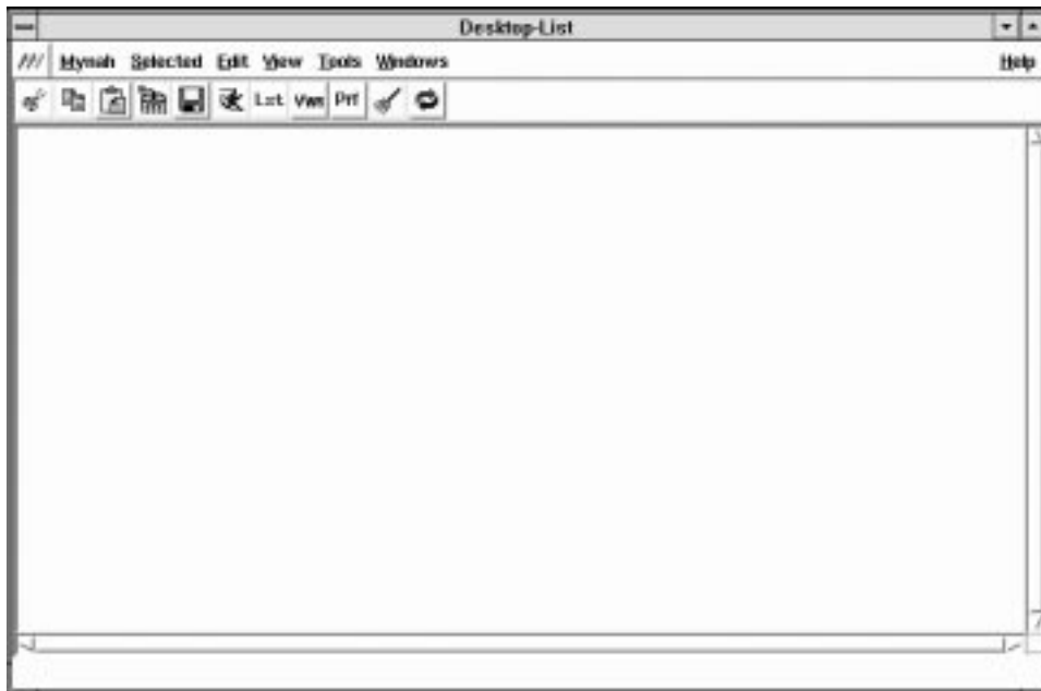
Figure 2-2. MYNAH Desktop
