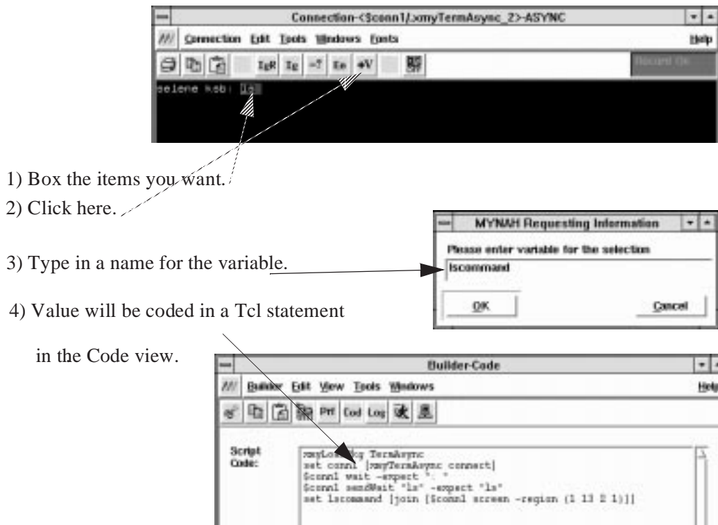
Figure 12-33. Saving a Value From a Screen Example
