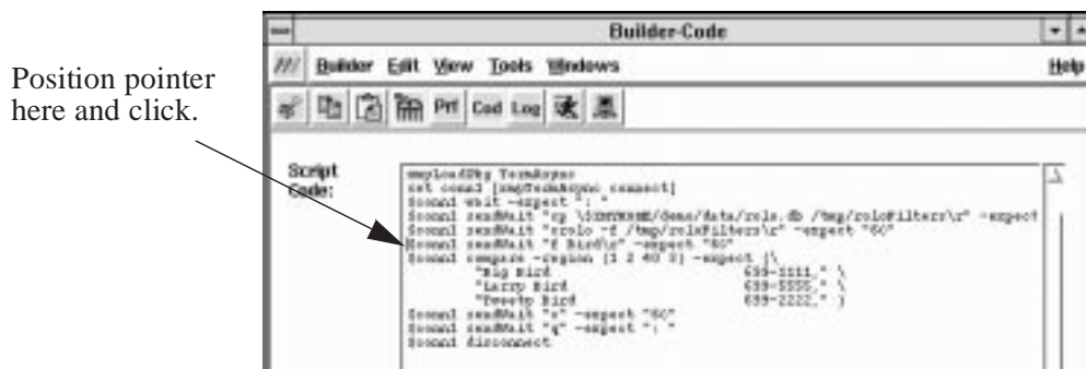
Figure 2-27. Positioning the Pointer to Insert a Tcl Statement
