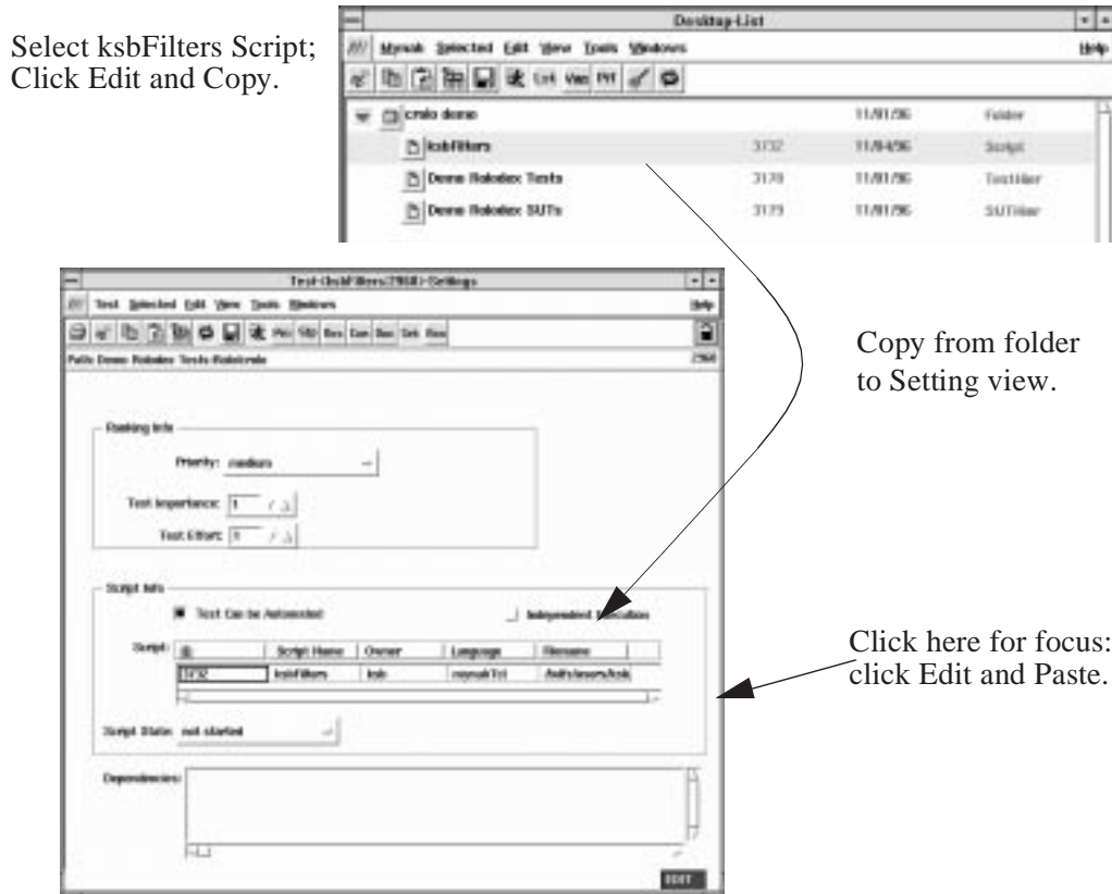
Figure 2-40. Identifying a Script to a Test
