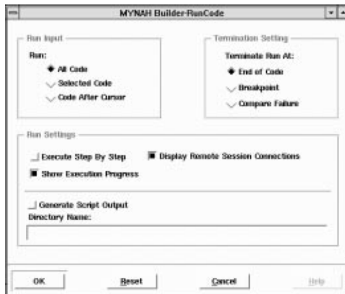
Figure 12-19. Run Code Dialog
