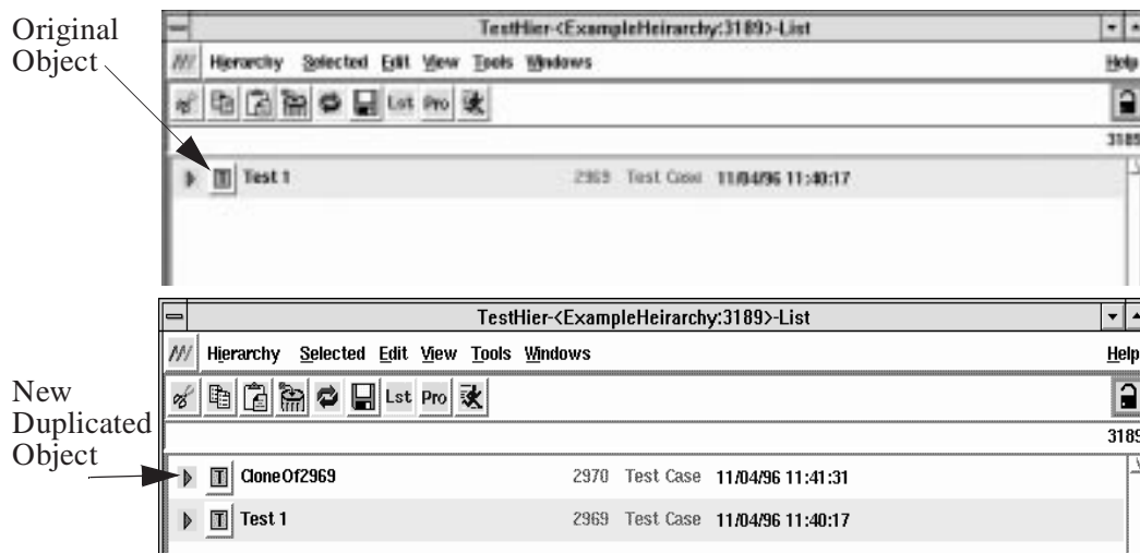
Figure 4-11. Duplicating Objects
