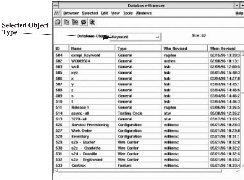
Figure 2-5. Database Browser
