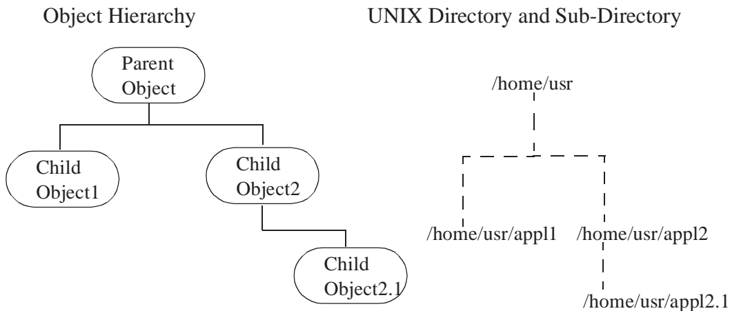
Figure 4-1. Hierarchy Idea
