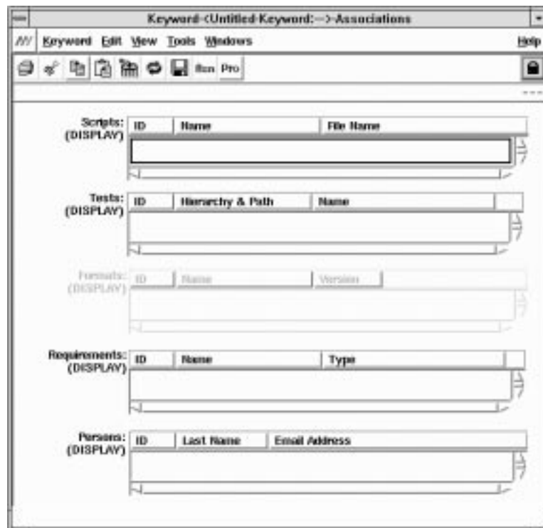
Figure 11-4. Associations View
