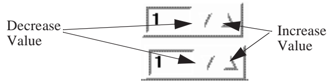
Figure 3-7. Spin Buttons
