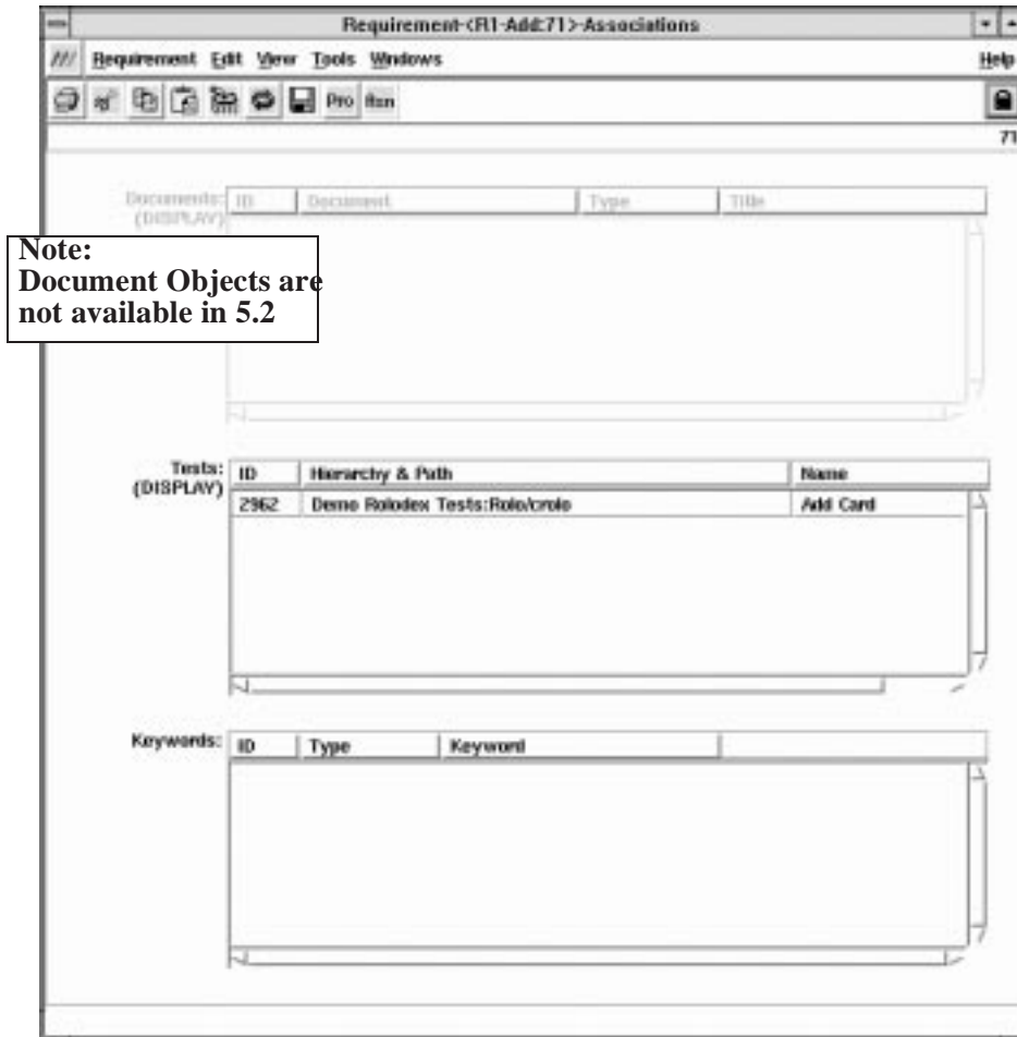
Figure 6-4. Associations View.
