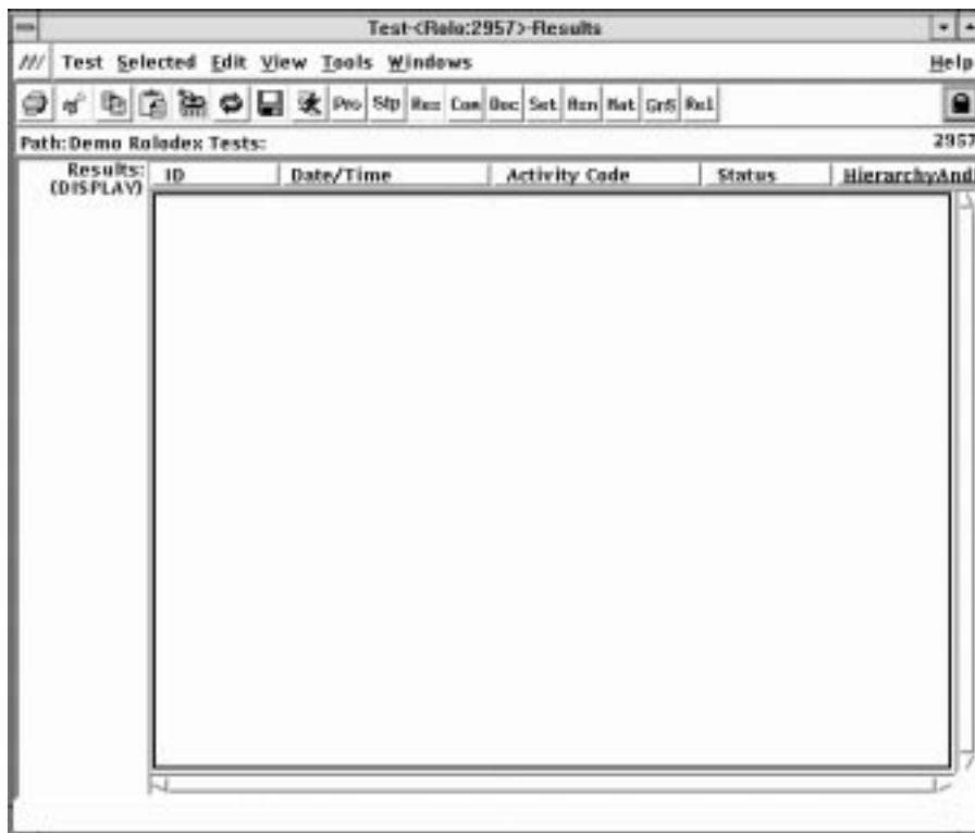
Figure 8-29. Results View
