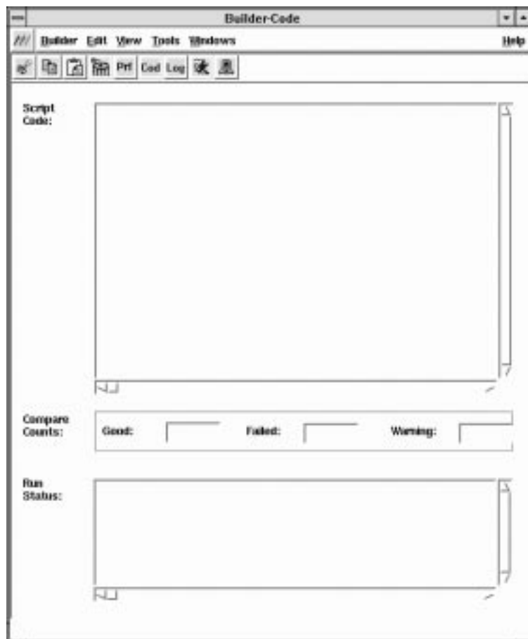
Figure 12-7. Code View
