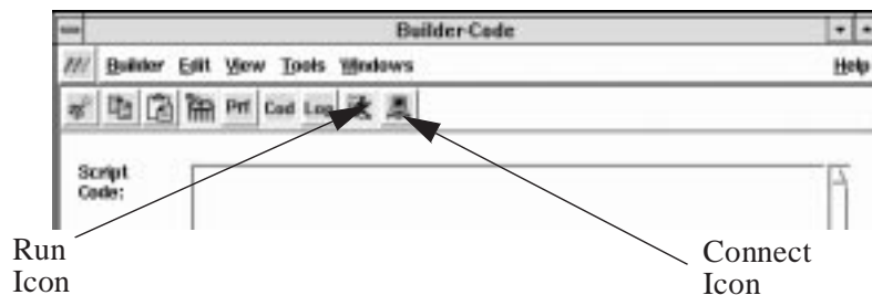
Figure 12-8. Dialog Icon
