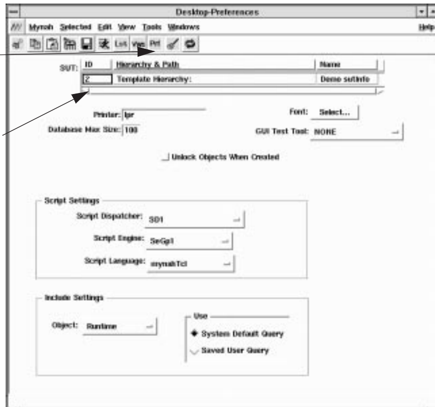
Figure 2-10. MYNAH Desktop-Preference
