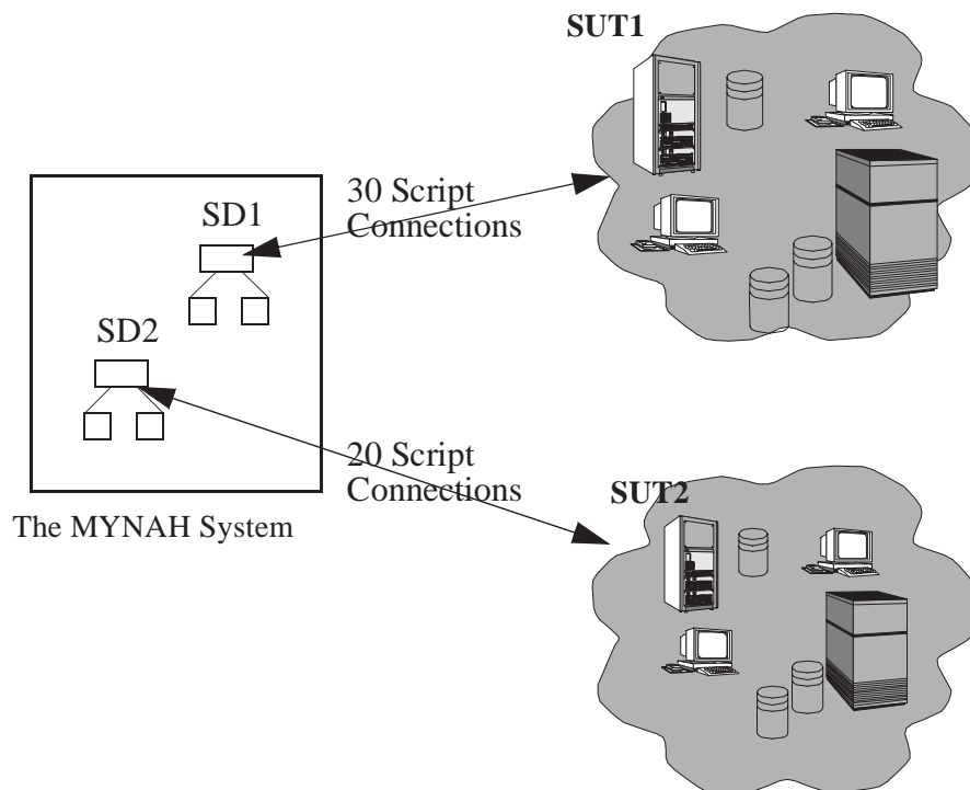
Figure 16-3. Testing Two SUTs Simultaneously with the BEE
