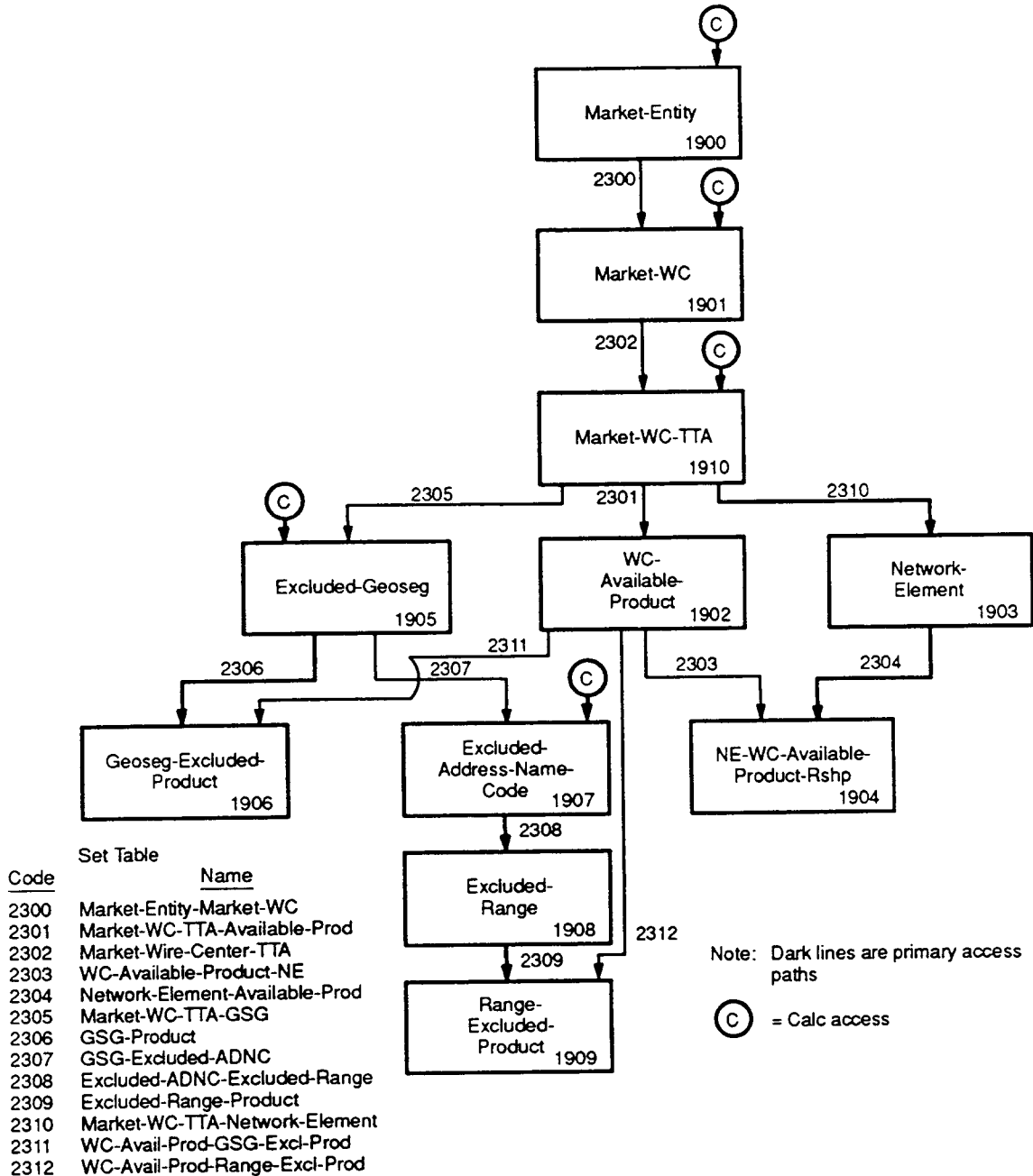
Figure 8-1. Schema Diagram of the MRKT-XXX Area
