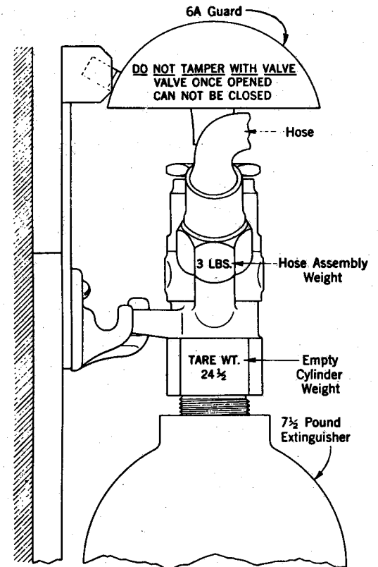
Fig. 3 - Handwheel Guard
