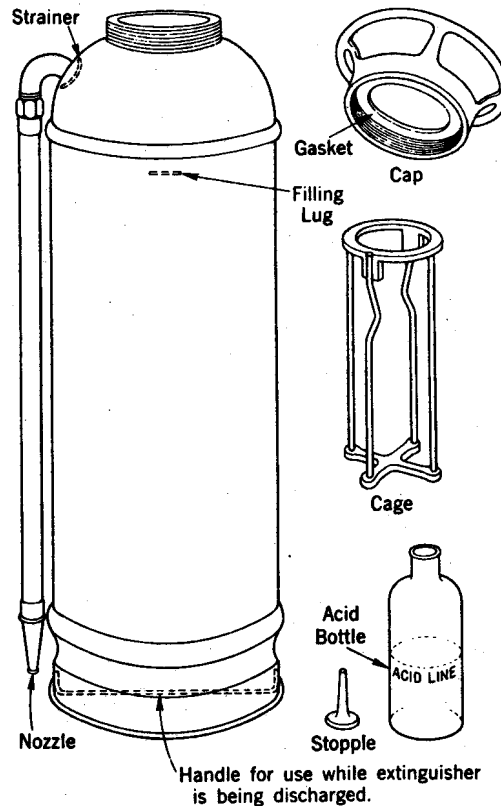
Fig. 6 - Soda Acid Extinguisher
