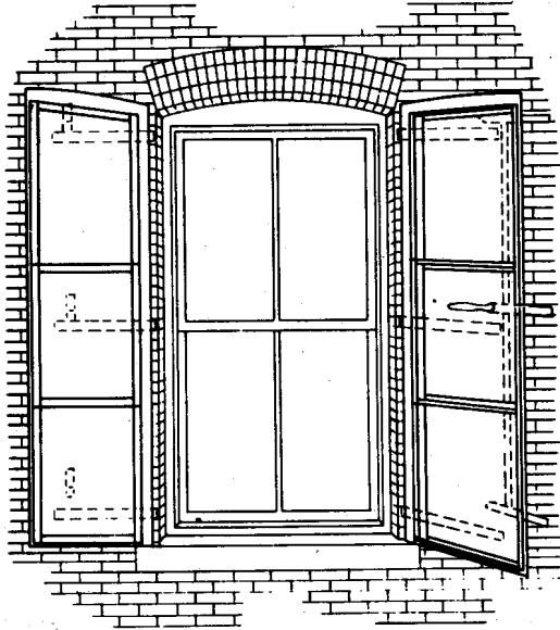
Fig. 9 - Manually Operated Fire Shutter - Open
