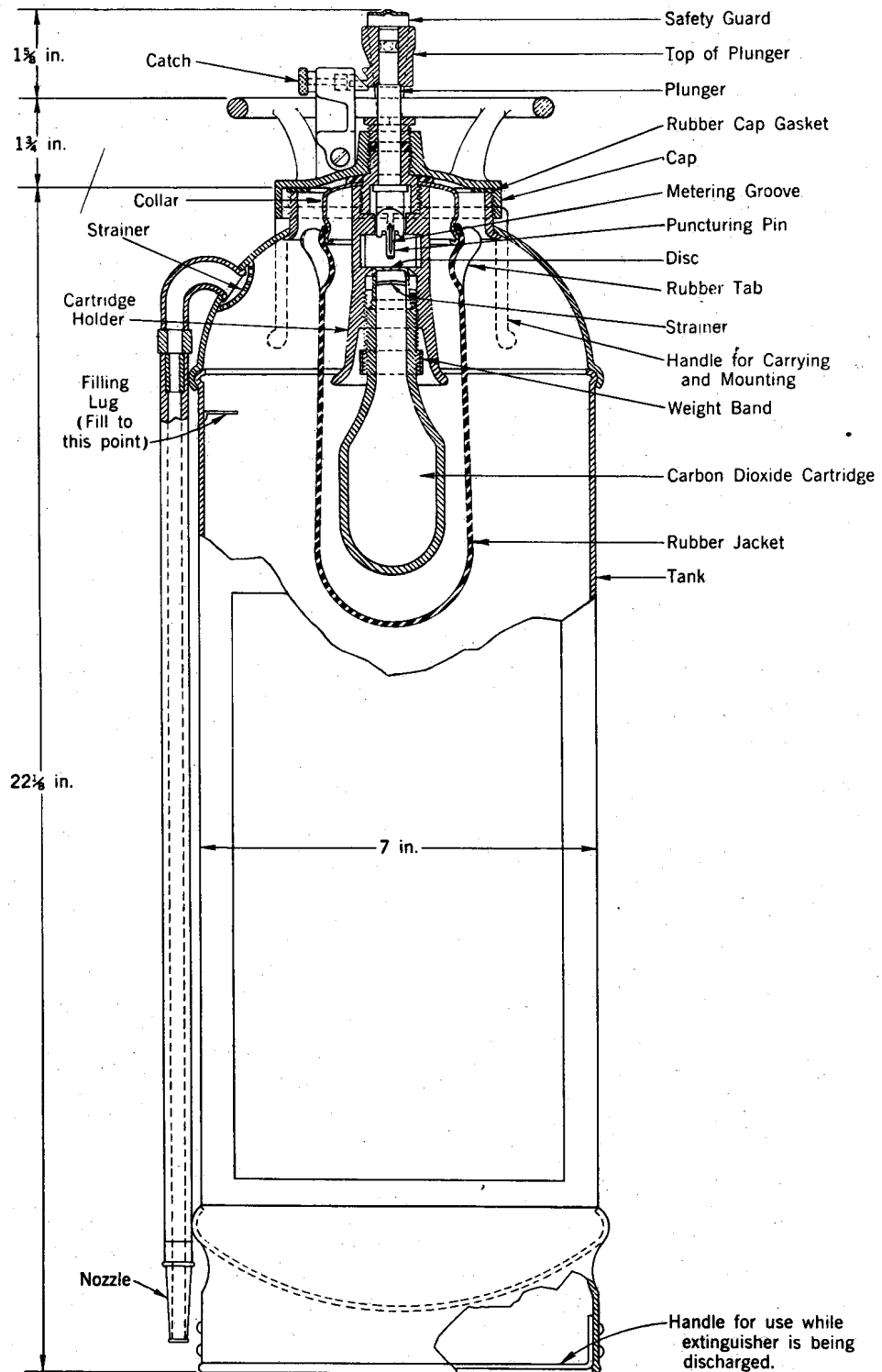
Fig. 4 - Water Extinguisher - Newer Design
