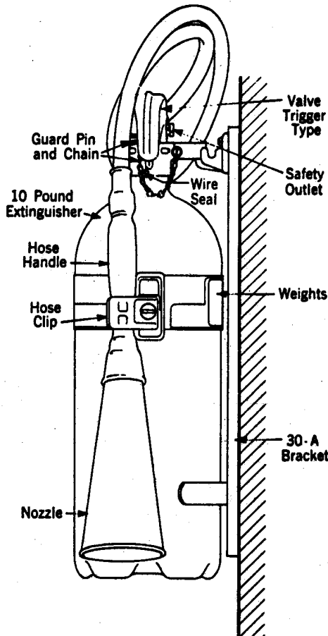
Fig. 1 - Carbon Dioxide Extinguisher - Newer Design
