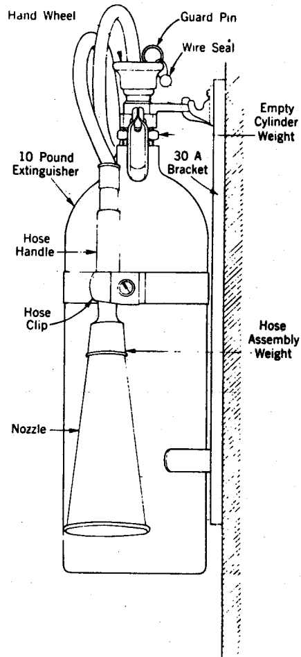
Fig. 2 - Carbon Dioxide Extinguisher - Former Design
