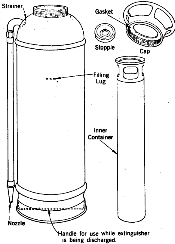
Fig. 5 - Foam Extinguisher
