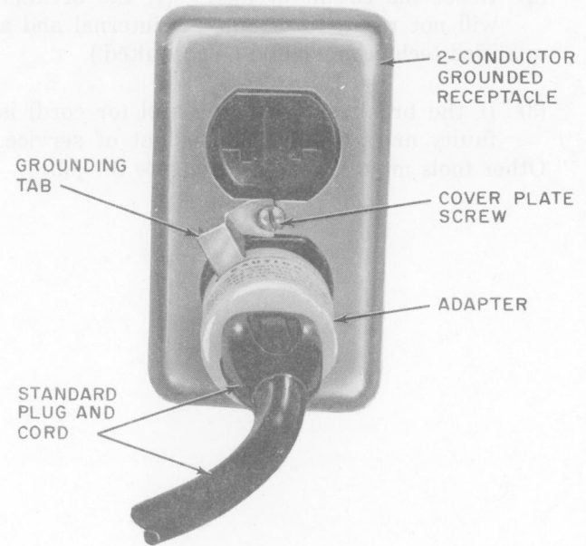
Fig. 10—Grounded 2-Conductor Receptacle
