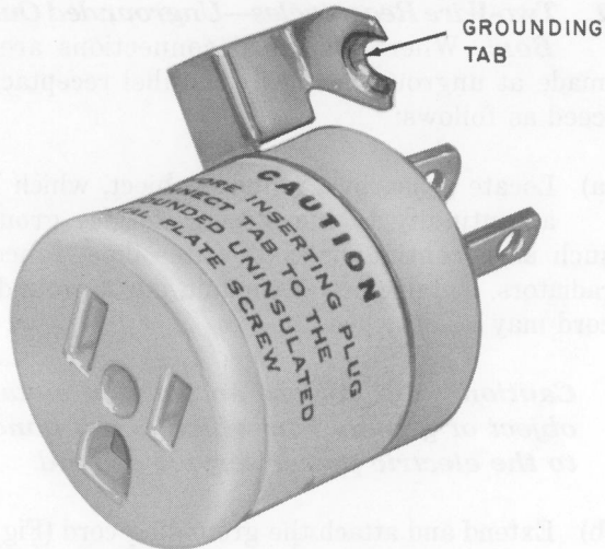
Fig. 2—Adapter
