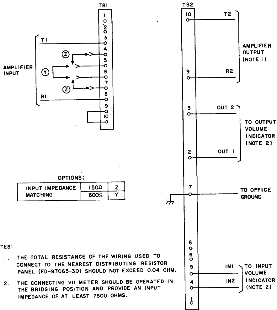
Fig. 2—KS-20425 L2 Amplifier System—Connections and Options
