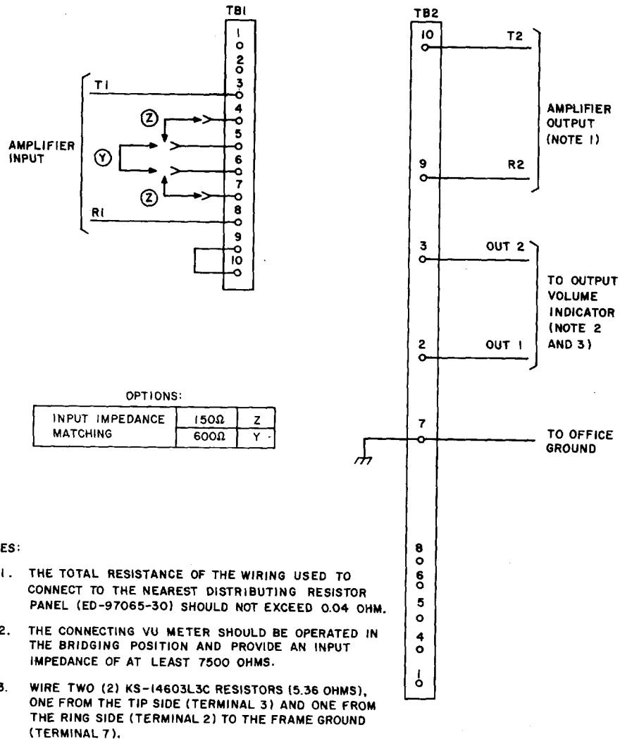
Fig. 1—KS-20425 L1 (Manufacture Discontinued) Amplifier System—Connections and Options
