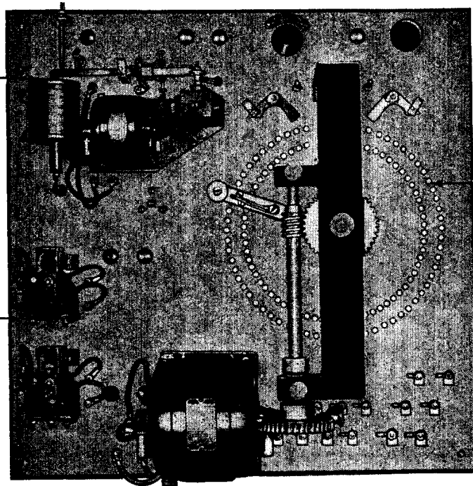
Fig. 3—D-C. Automatic Rotating Cam Type Voltage Regulator (KS-5117)
