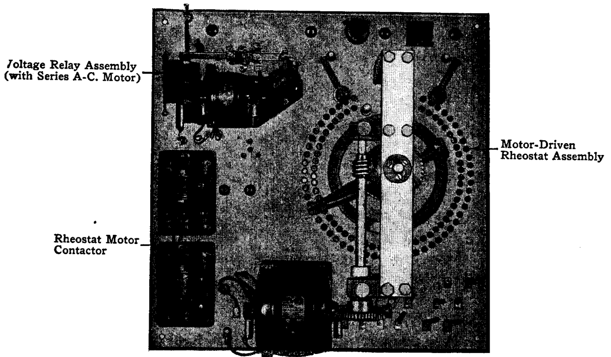
Fig. 5—A-C. Automatic Rotating Cam Type Voltage Regulator (KS-5016)
