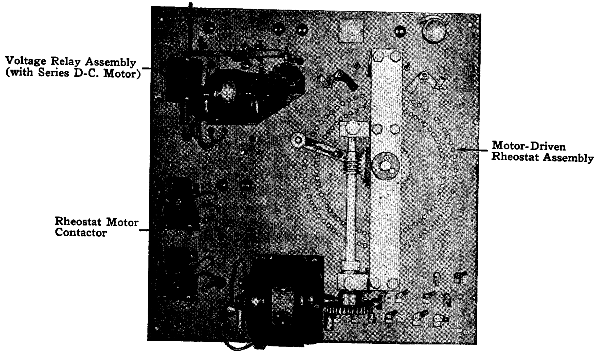
Fig. 4—D-C. Automatic Rotating Cam Type Voltage Regulator (KS-5016)
