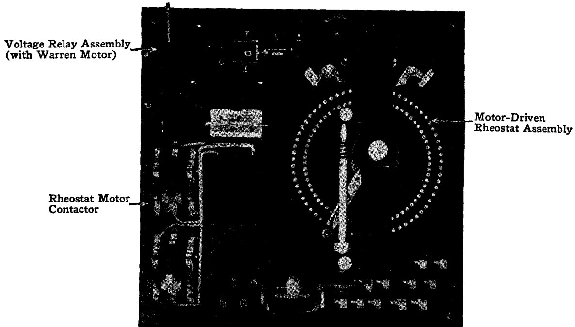
Fig. 1—A-C. Automatic Rotating Cam Type Voltage Regulator (KS-5117, Front View Shown)
