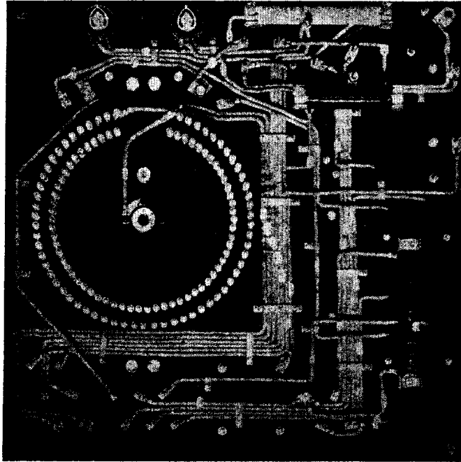
Fig. 2—A-C. Automatic Rotating Cam Type Voltage Regulator (KS-5117, Rear View Shown)
