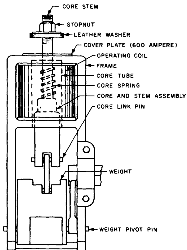
Fig. 3—Typical Operating Solenoid Assembly
