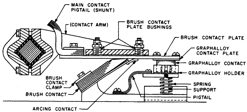
Fig. 10—Main Contact Structure of 600-Ampere Contactors
