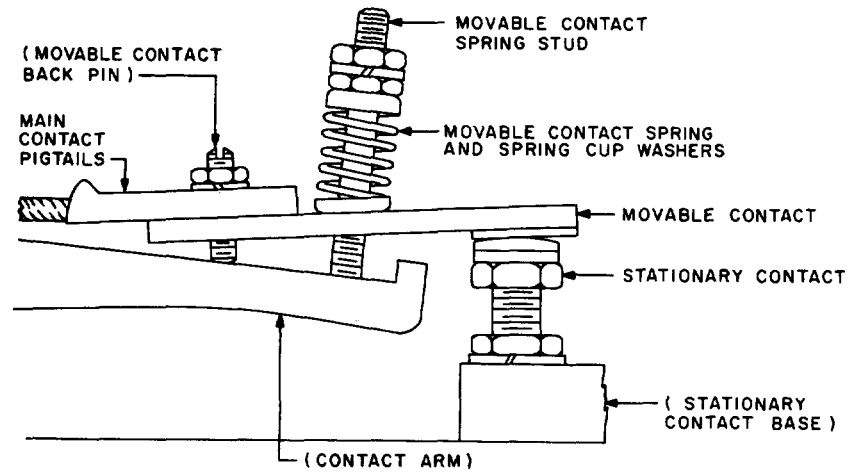
Fig. 7—Main Contact Structure (Butt Type) of 75- and 100-Ampere Contactors
