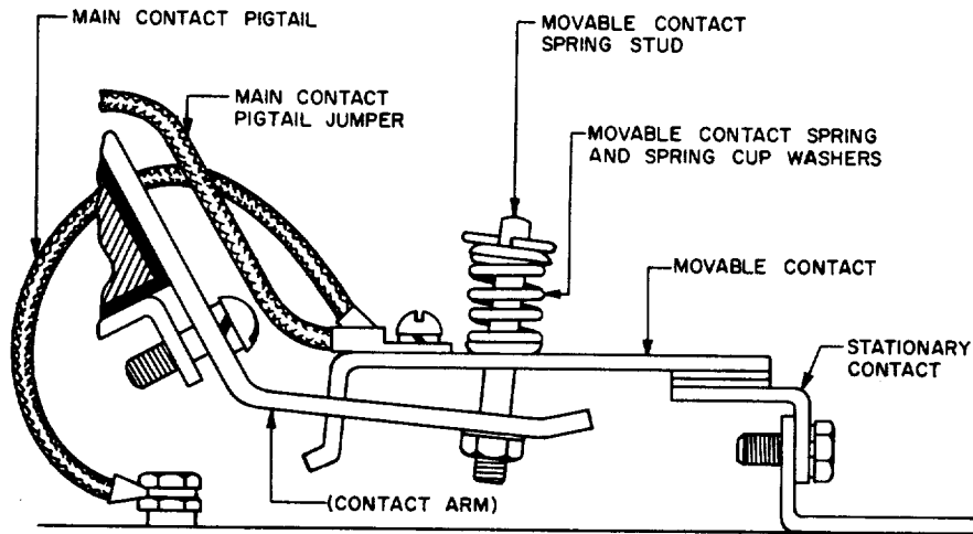
Fig. 6—Main Contact Structure (Butt Type) of 30-Ampere Contactors
