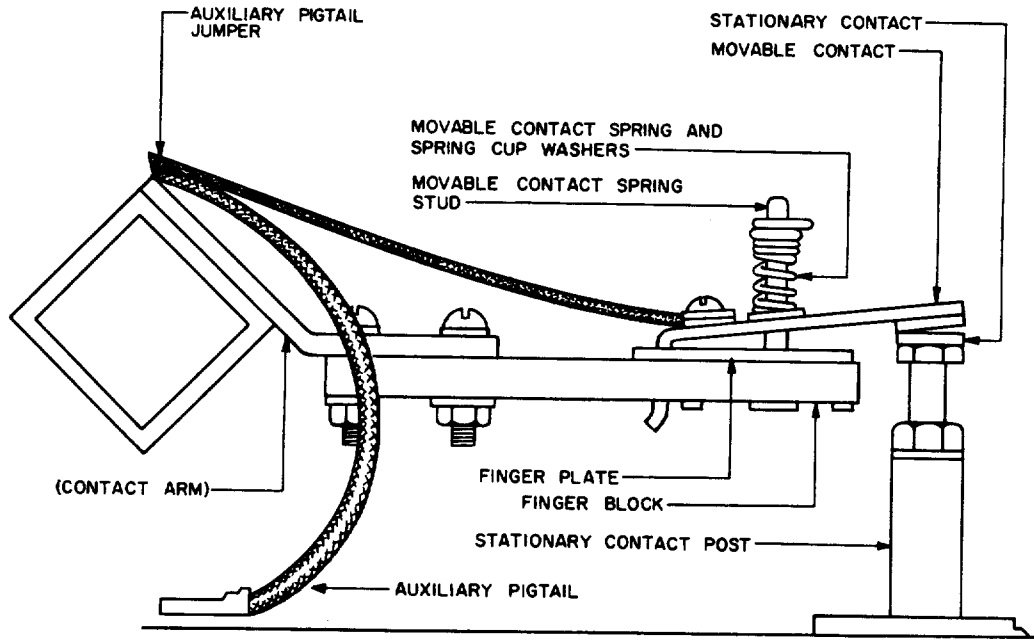
Fig. 5—Auxiliary Contact Structure (Butt Type) of 200-, 300-, 400-, and 600-Ampere Contactors
