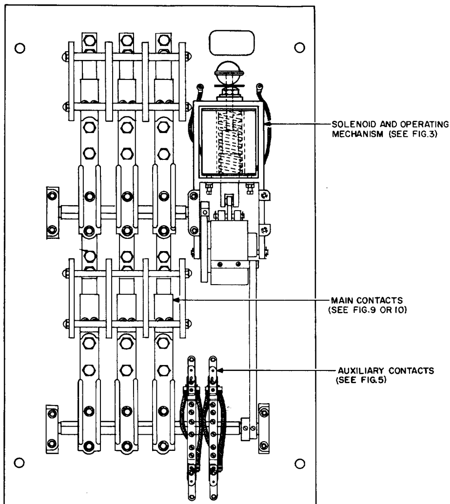
Fig. 2—Typical KS-15514 and KS-15934, 200-, 300-, 400-, and 600-Ampere Contactors
