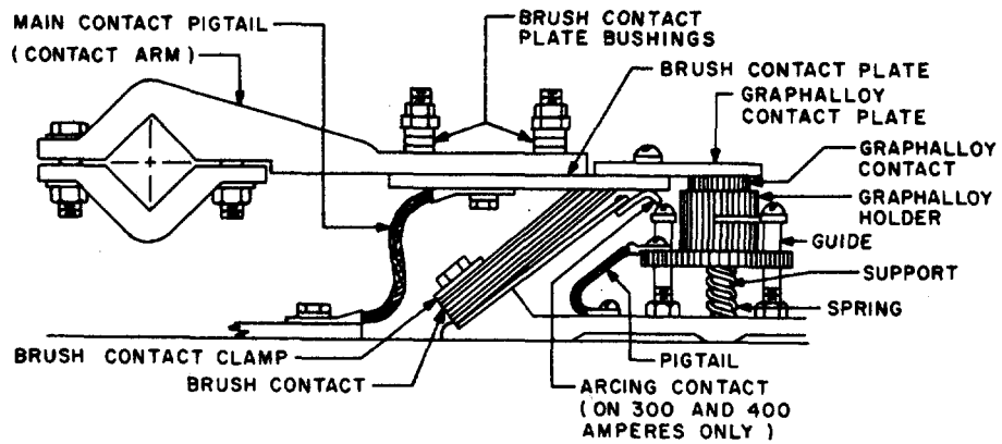
Fig. 9—Main Contact Structure of 200-, 300-, and 400-Ampere Contactors
