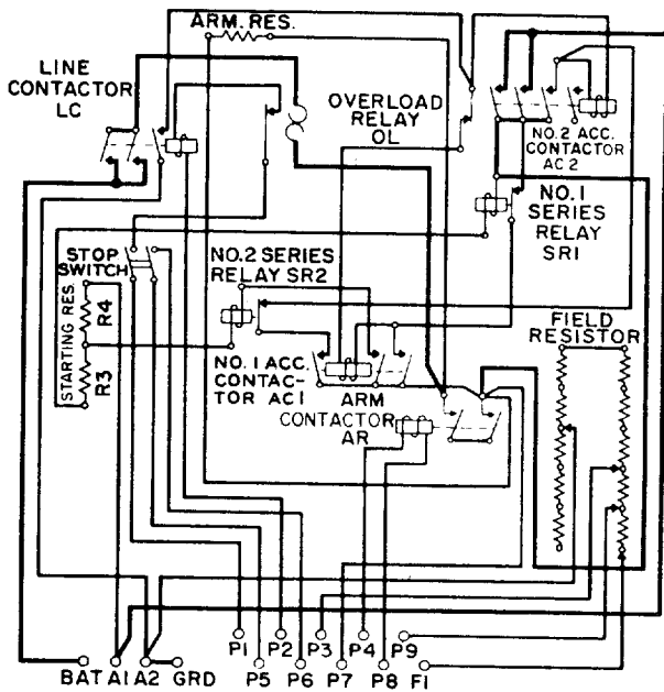
Fig. 3 – Schematic for KS-15582 L4
