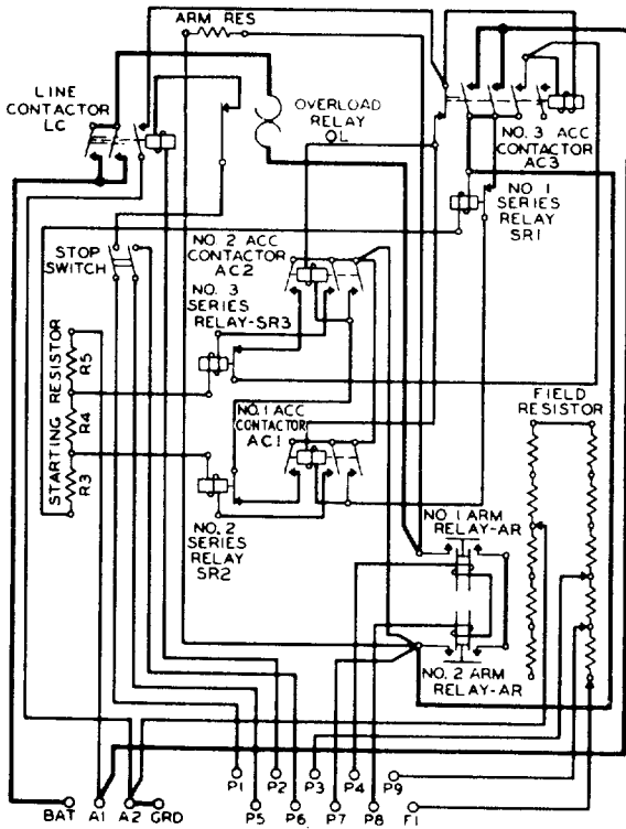
Fig. 2 – Schematic for KS-15582 L2 and L3
