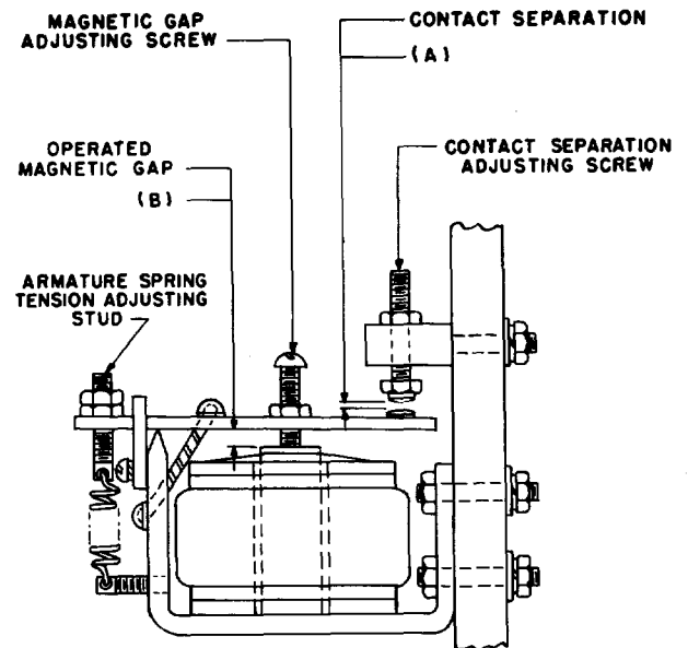
Fig. 7 — SR Relay (shown in operated position)
