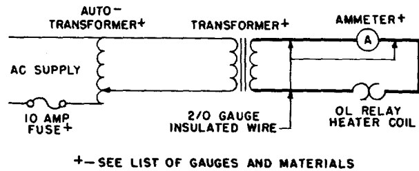
Fig. 8 – Circuit for Checking Operate Current of OL Relay
