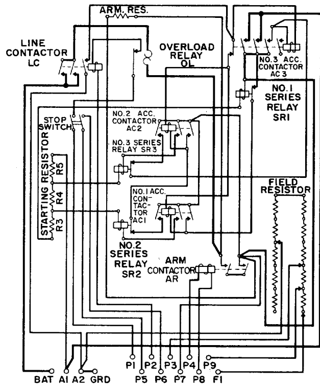
Fig. 4 – Schematic for KS-15582 L5 and L6
