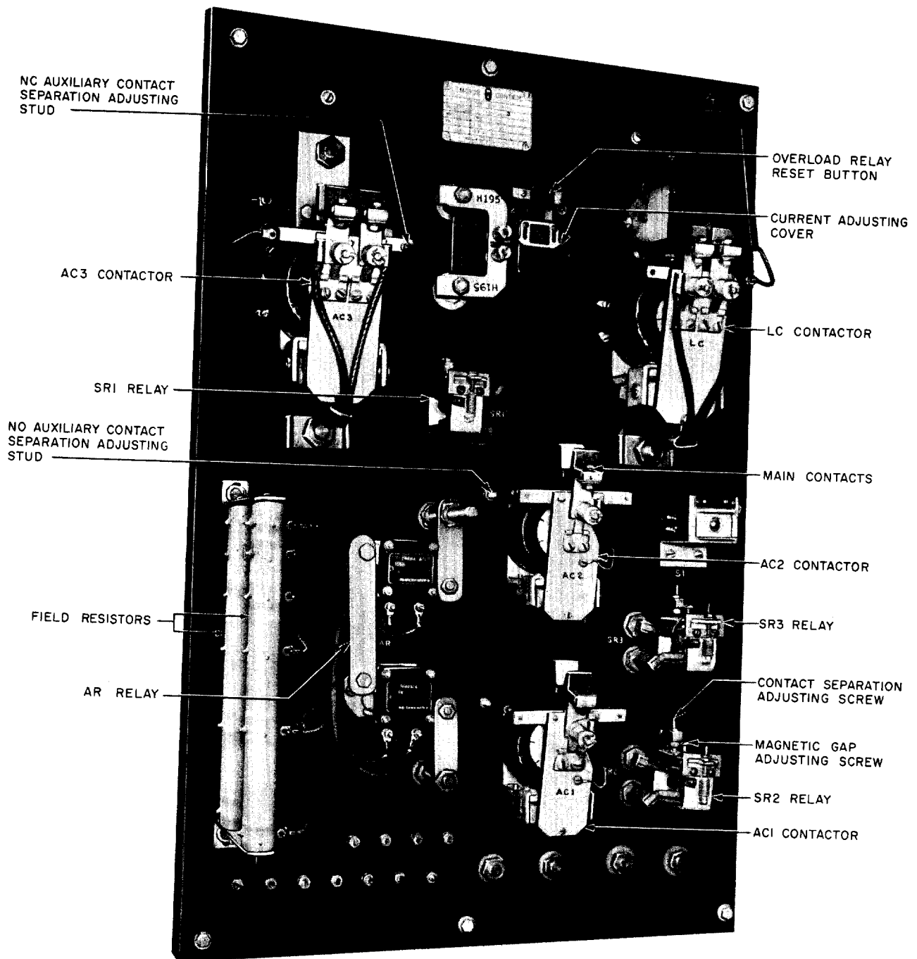
Fig. 5 - KS-15582 L2 Starter
