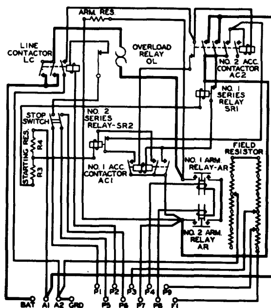
Fig. 1 - Schematic for KS-15582 L1
