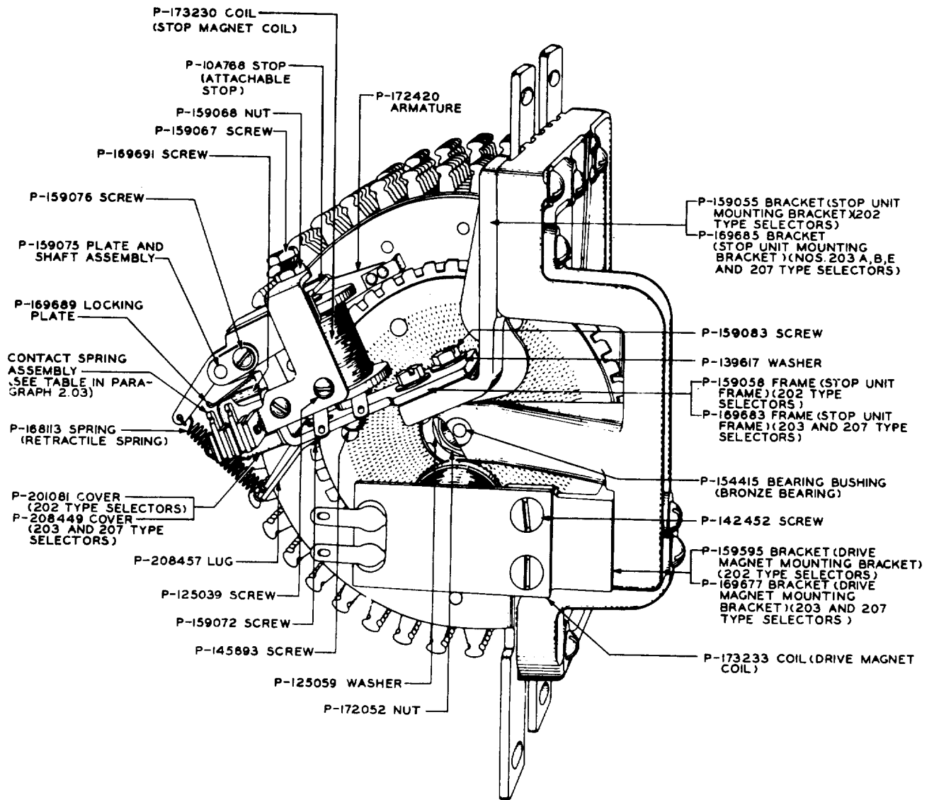
Fig. 2 - Side View Showing General Design of 202 Type, Nos. 203A, B, E and 207 Type Selectors Together with Associated Banks
