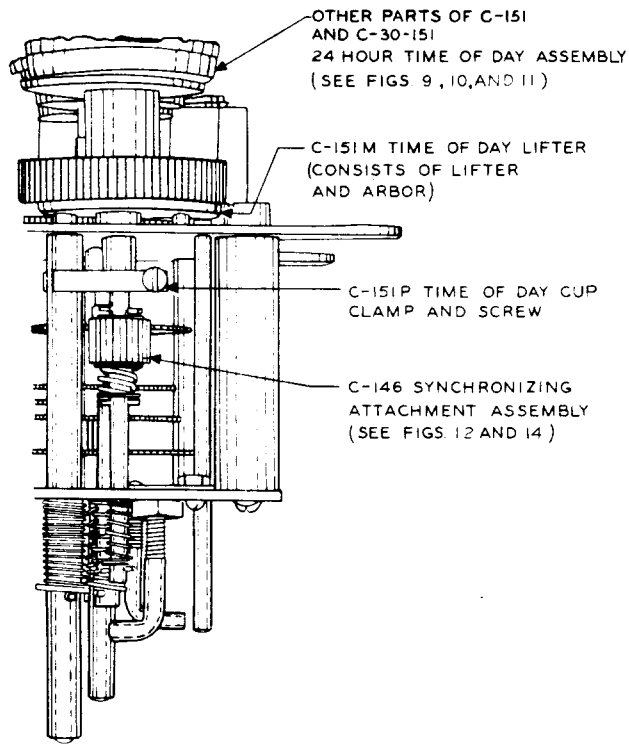
Fig. 15 - Clamping Arrangement for 24-Hour Time-of-Day Assembly
