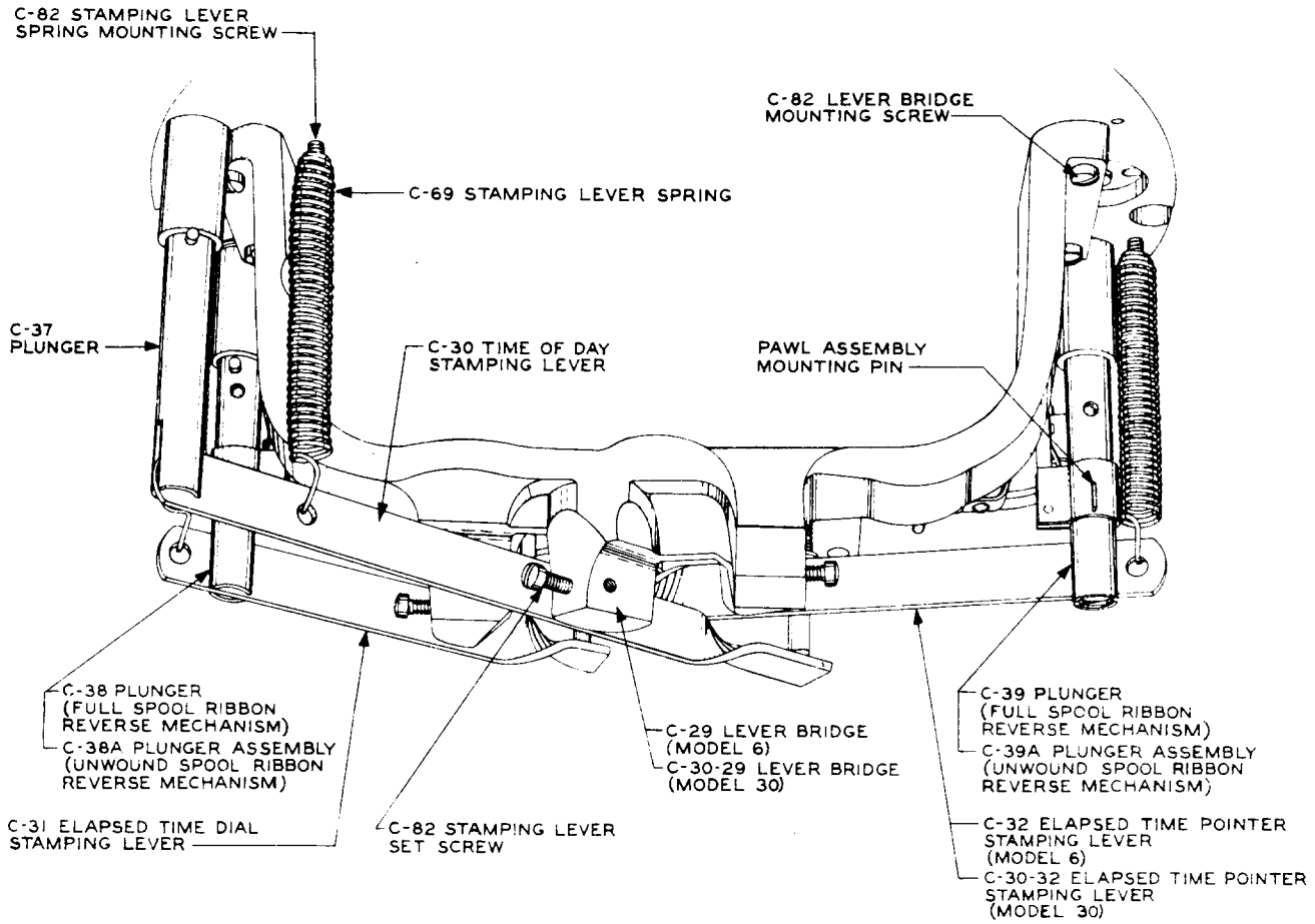
Fig. 18 – Stamping Mechanism — Models 6 and 30 Calculagraphs
