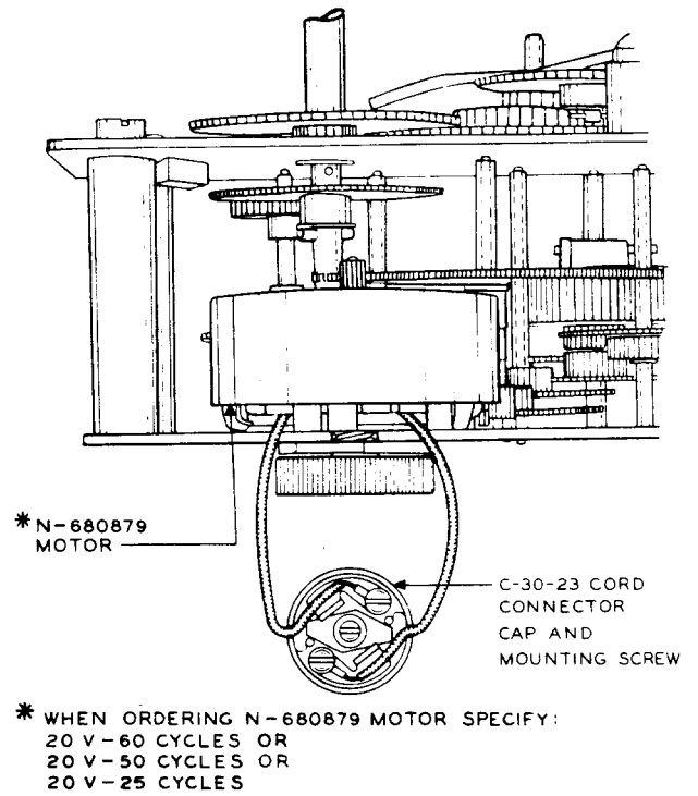
Fig. 16 - Motor Mechanism - Model 30 Calculagraph (Motor With Aluminum Cap Rotor)
