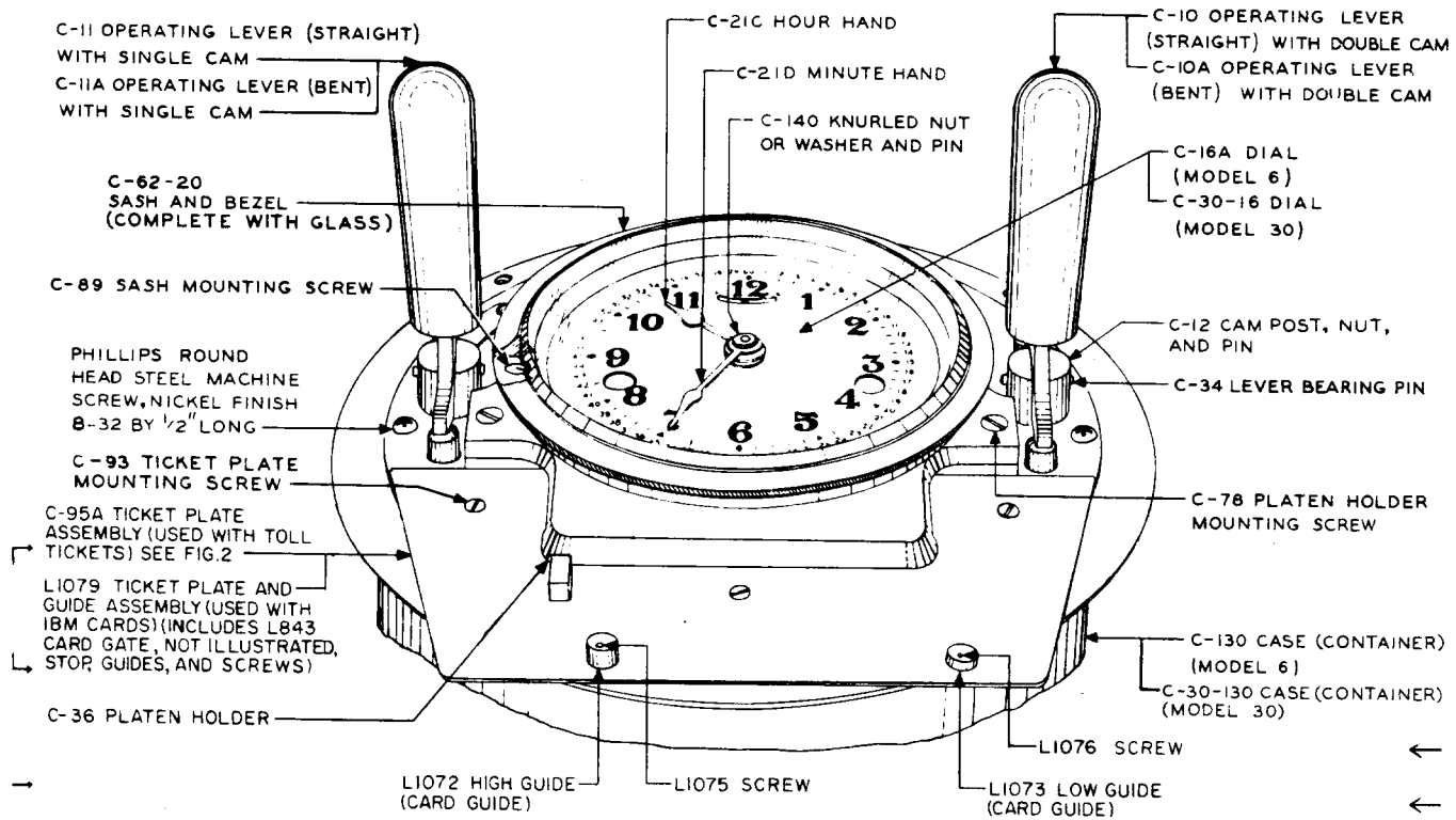
Fig. 1 - Top View of Calculagraph
