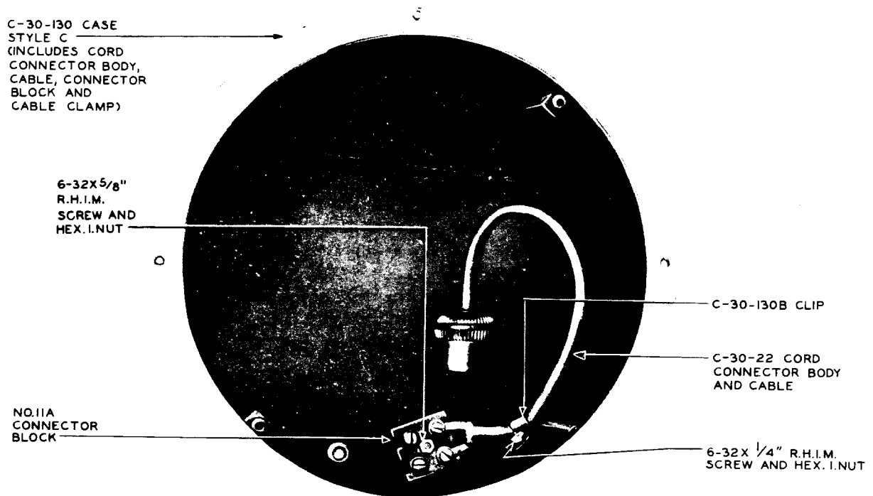
Fig. 20 — Case and Associated Parts — Model 30 Calculagraph
