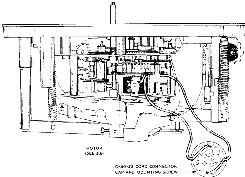
Fig. 17 - Motor Mechanism - Model 30 Calculagraph (Motor With Copper Bar Rotor)
