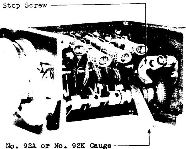
Fig. 5 - Checking Stop Screw Position
