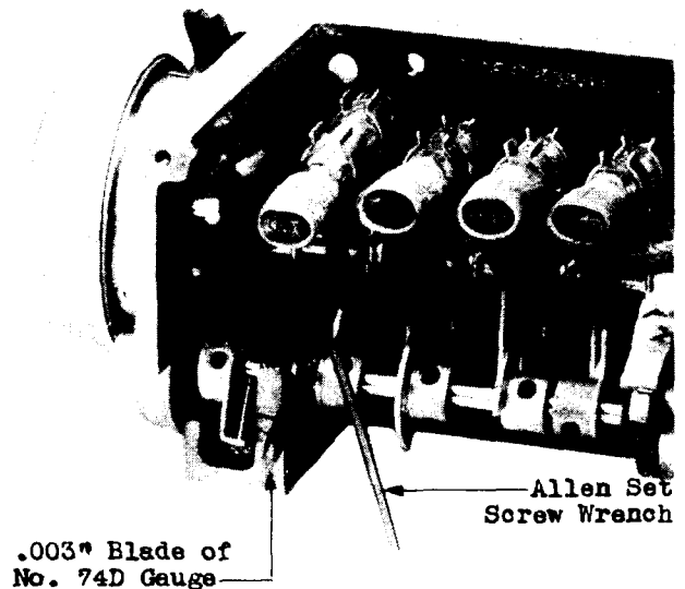
Fig. 6 - Adjusting End Play of Cam Shaft
