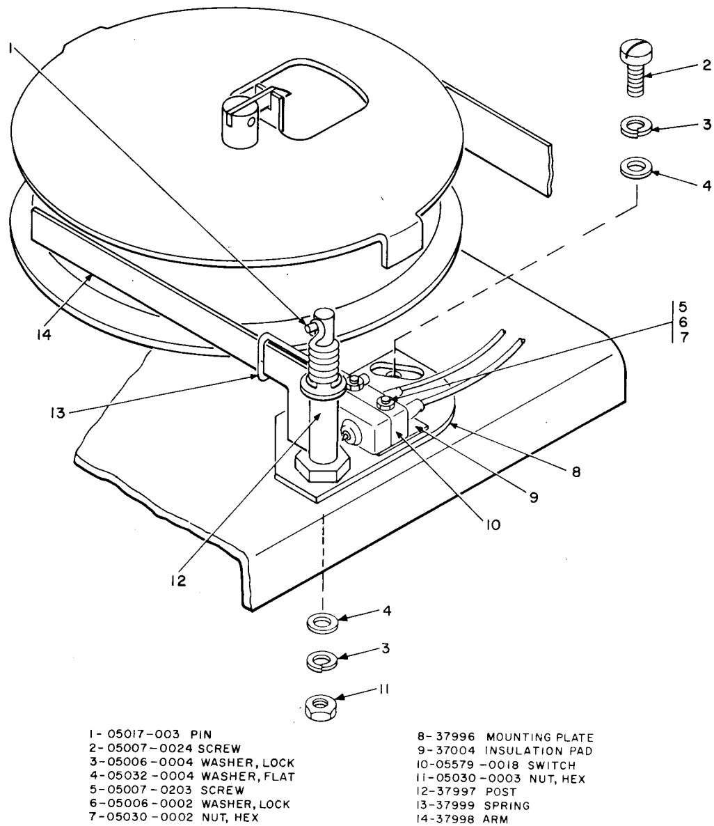
Fig. 6—KS-19717 L11 Low Tape Alarm
