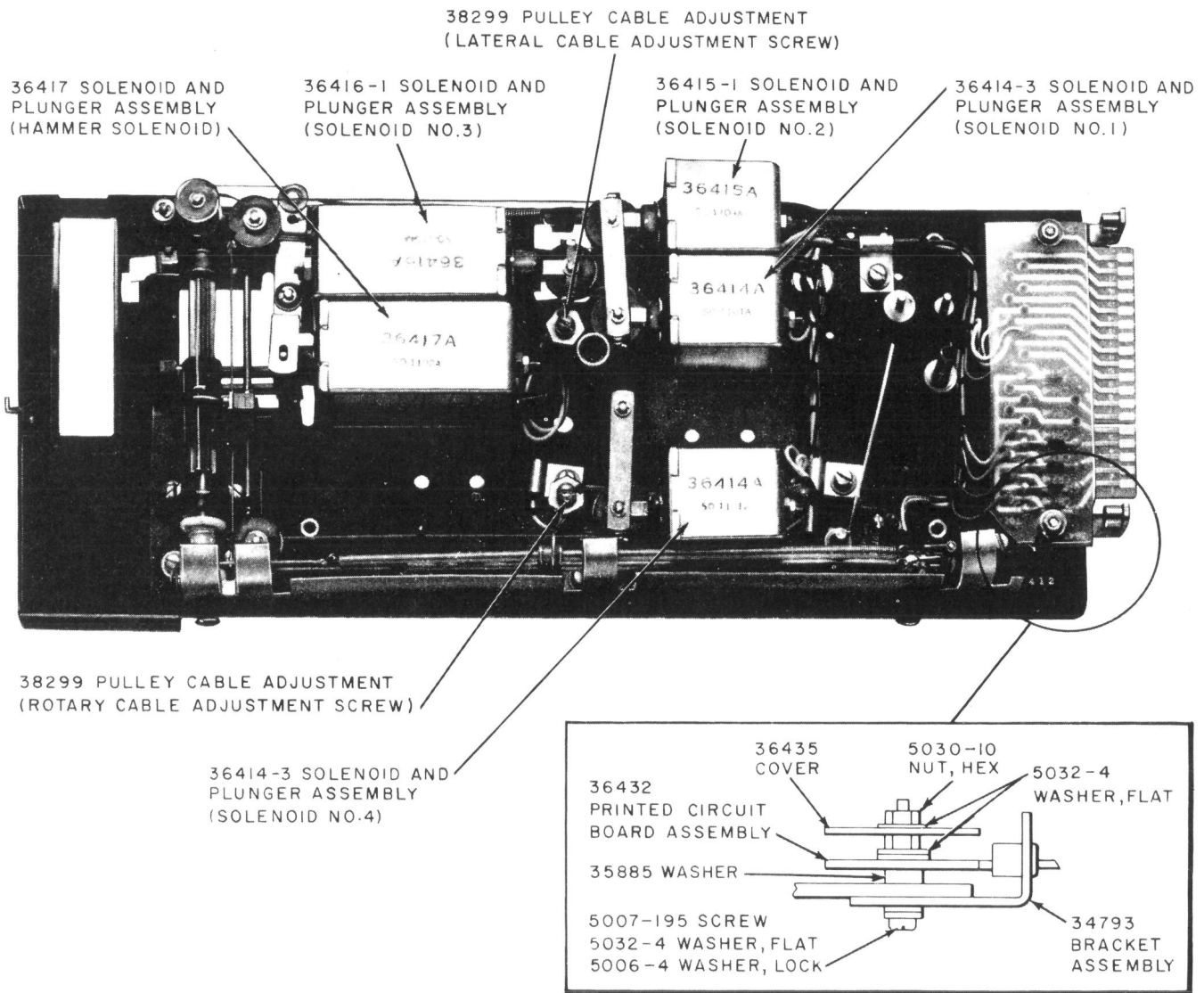
Fig. 3—KS-19717 L5 Tape Printer Showing Circuit Board
