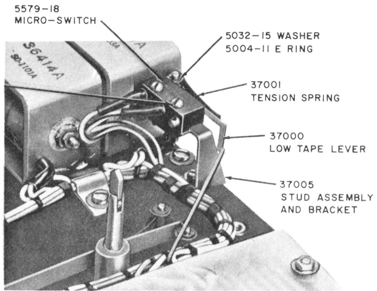
Fig. 4—KS-19717 L10 Low Tape Alarm
