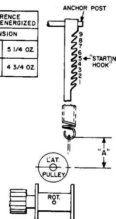
Fig. 8—Rotary and Lateral Return Spring Attachment and Adjustment
