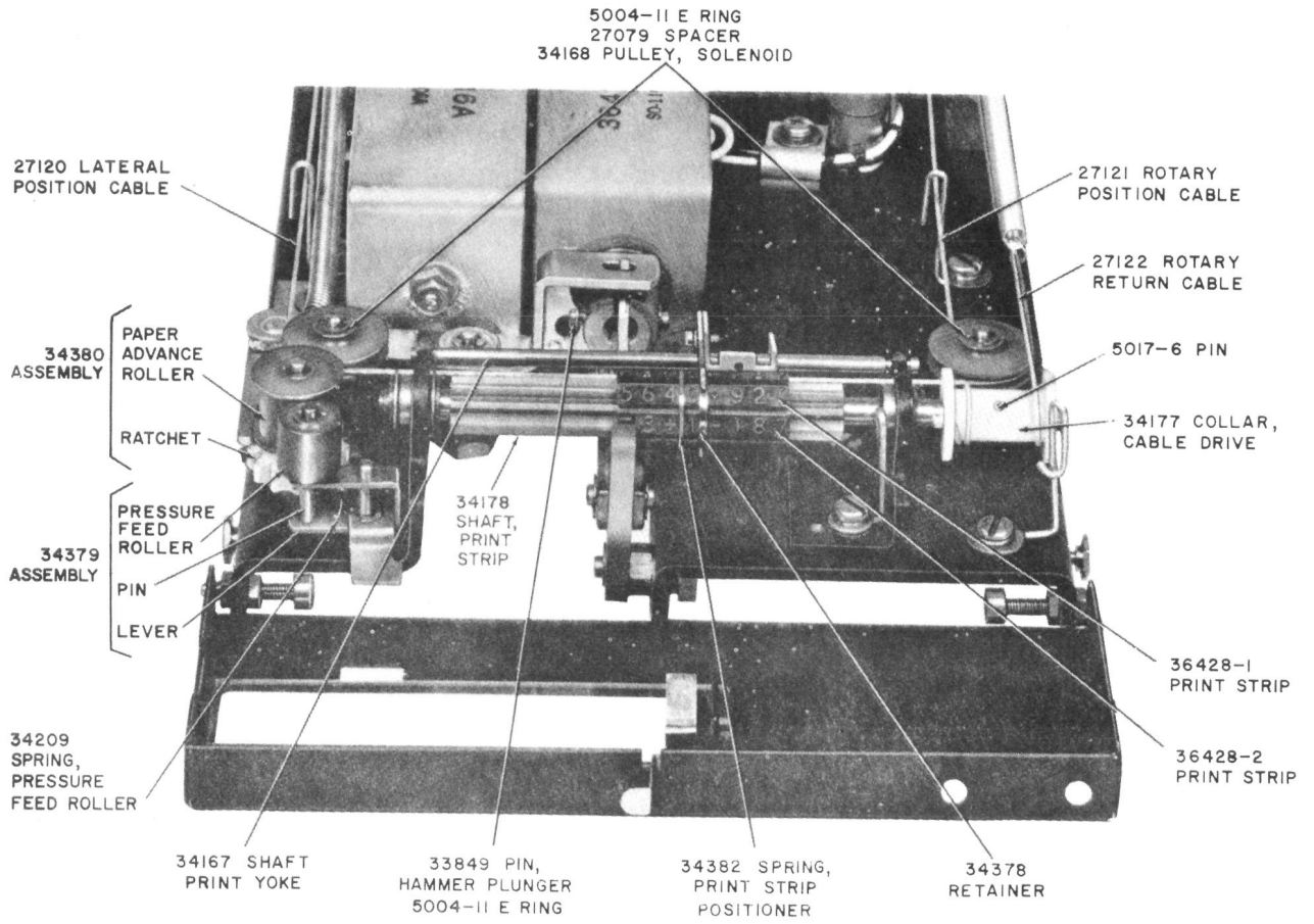
Fig. 2—KS-19717 L5 Tape Printer Showing Print Segments
