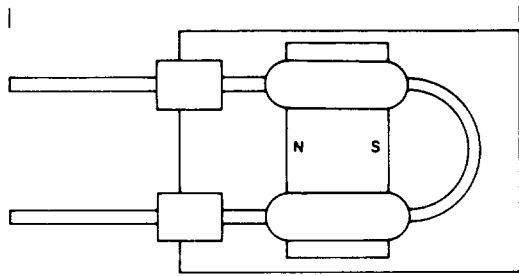
Fig. 17—Block Magnets
