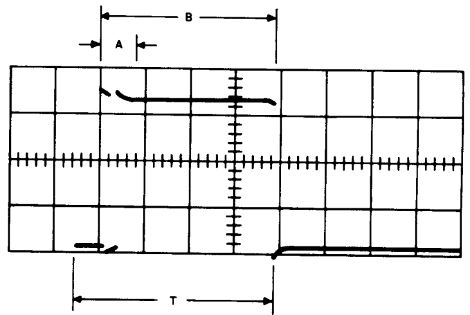
Fig. 23—Timing Chart (S1 to OFF)
