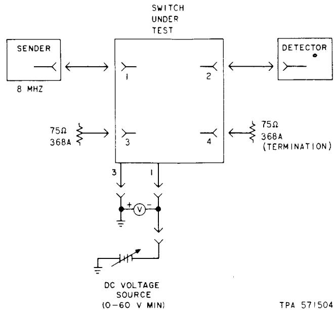
Fig. 19—Insertion and Isolation Loss/Test Circuit
