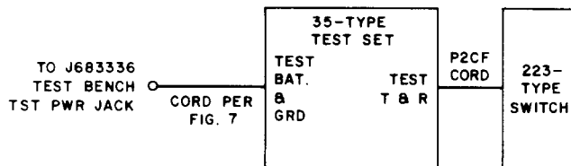
35-TYPE TEST SET PREPARATION FOR TEST
