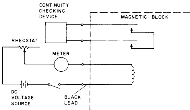
Fig. 18—Indicating Circuit
