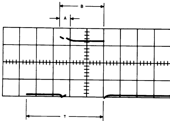
Fig. 22—Timing Chart (S1 to ON)
