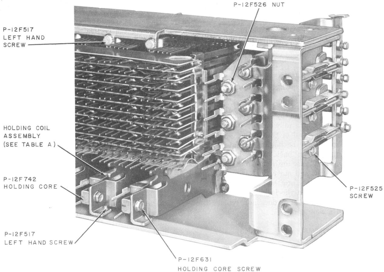
Fig. 3—Partial Rear View of Switch
