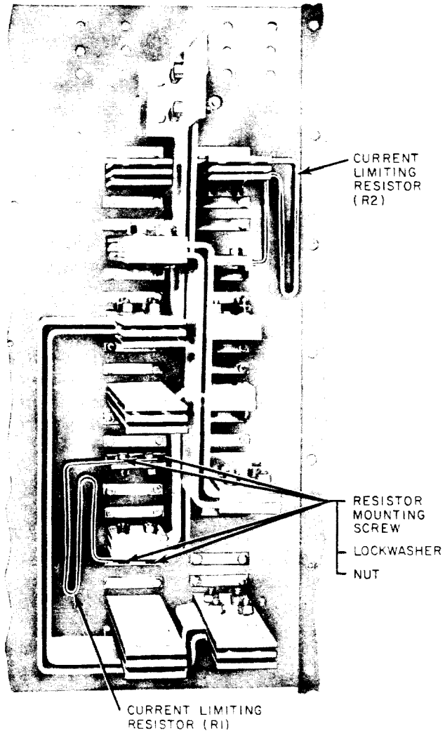
Fig. 4—KS-15847 Type Switch (partial rear view)
