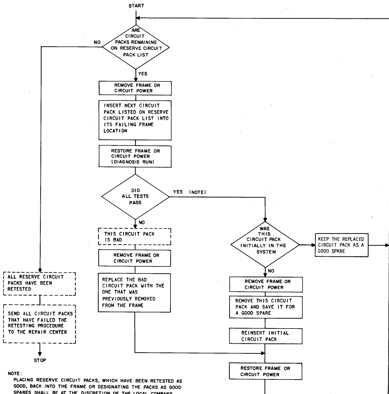
Fig. 12—Procedure for Retesting Reserve Circuit Packs
