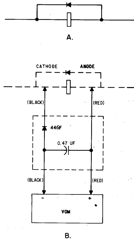
Fig. 9—Diode Test Hookup Procedure 1
