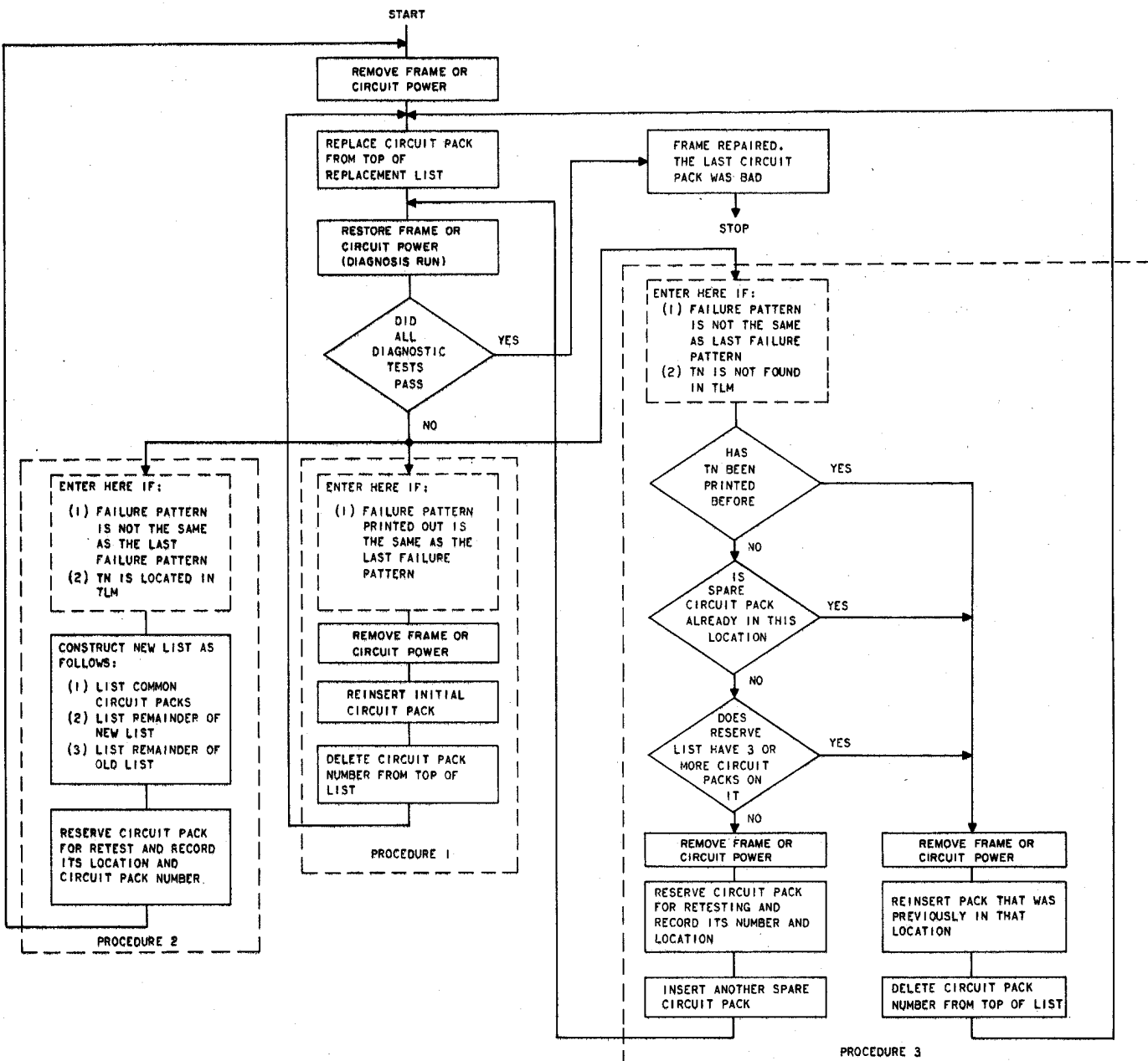
Fig. 11—Procedure for Replacing Faulty Circuit Packs
