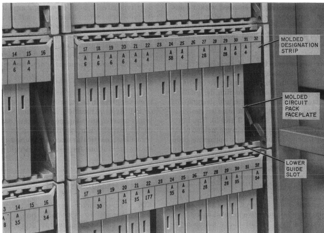
Fig. 4—Molded Circuit Faceplate and Front of Apparatus Mounting With Hinged Description Strip in Normal Position
