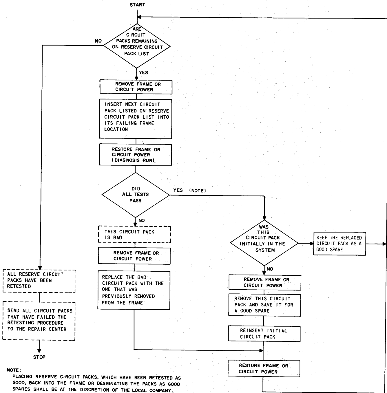
Fig. 13—Procedure for Retesting Reserve Circuit Packs
