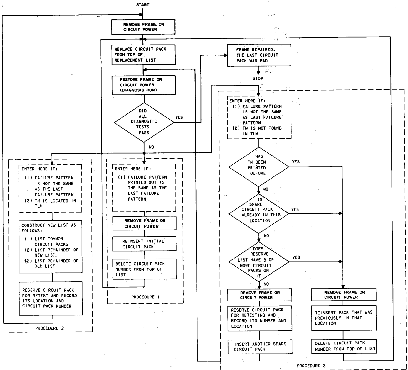
Fig. 12—Procedure for Replacing Faulty Circuit Packs
