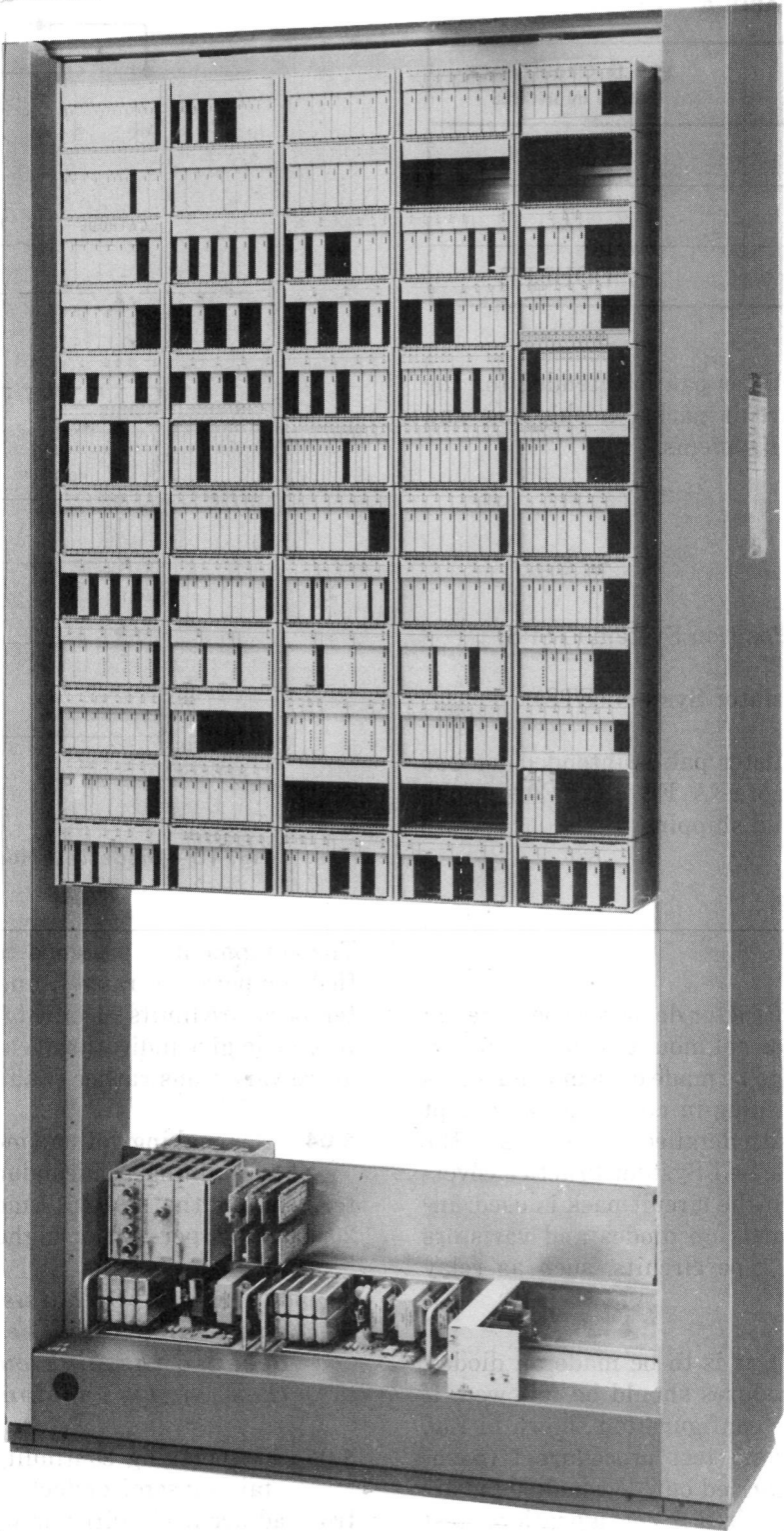
Fig. 9—Circuit Pack Storage Frame for No. 2, 2B, and 3 ESS Offices
