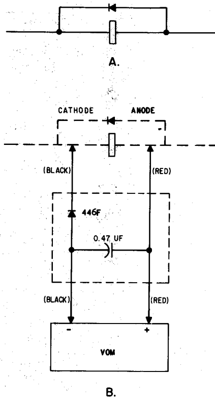
Fig. 10—Diode Test Hookup Procedure 1
