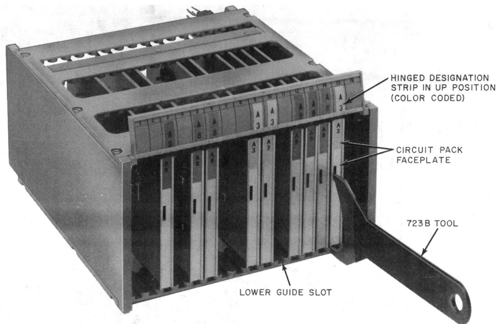
Fig. 5—Apparatus Mounting With Hinged Designation Strip in Raised Position
