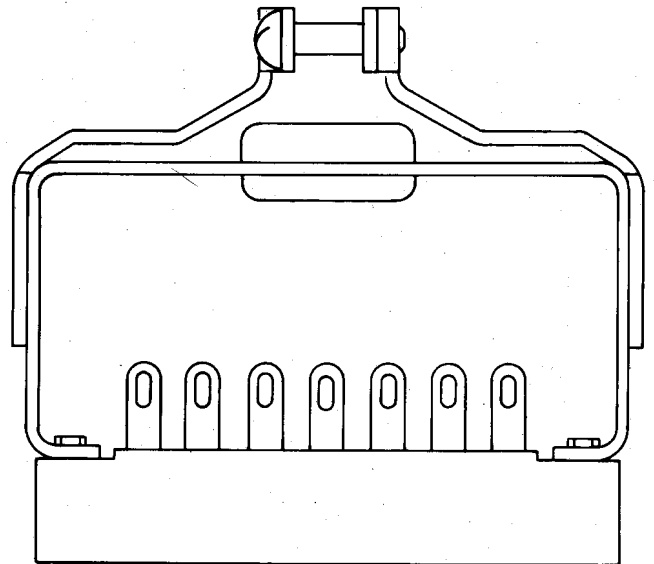
Fig. 15—KS-16323 Connector
