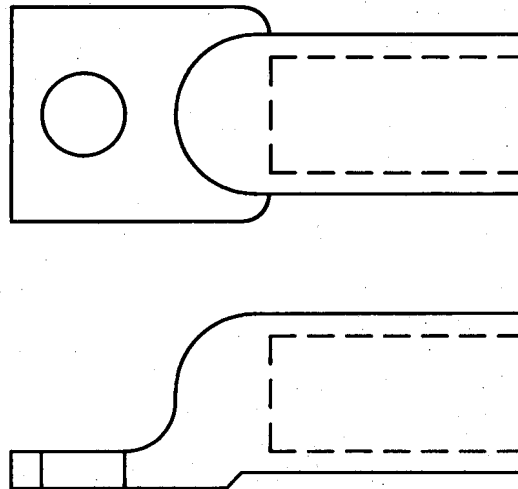
Fig. 12—KS-15977-Type Connector
