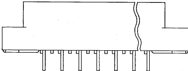
Fig. 13—KS-16182-Type Connector
