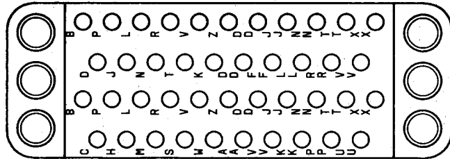
Fig. 10—KS-16409, L10 Connector
