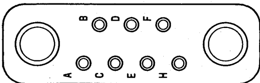
Fig. 8—KS-16409, L22 or L33 Connector
