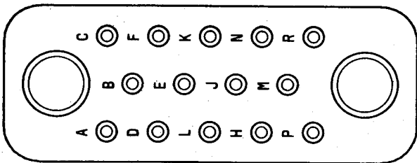
Fig. 1—KS-16409, L1, L21, L23, L39, L41, L45, or L50 Connector
