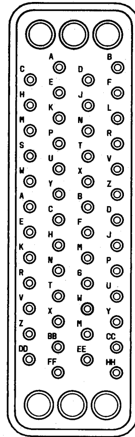
Fig. 6—KS-16409, L11, L12, L13, L14, L24, L25, L28, L43, or L47 Connector
