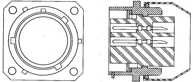
Fig. 8—KS-20461-Type Connector
