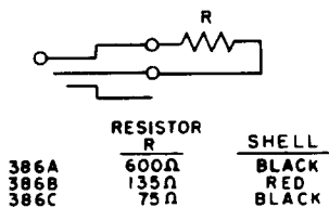
Fig. 10—386-Type Plug
