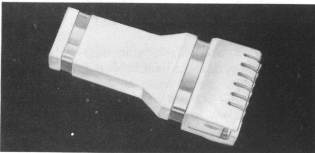
Fig. 2—459-Type Plug (6-Wire Switches)
