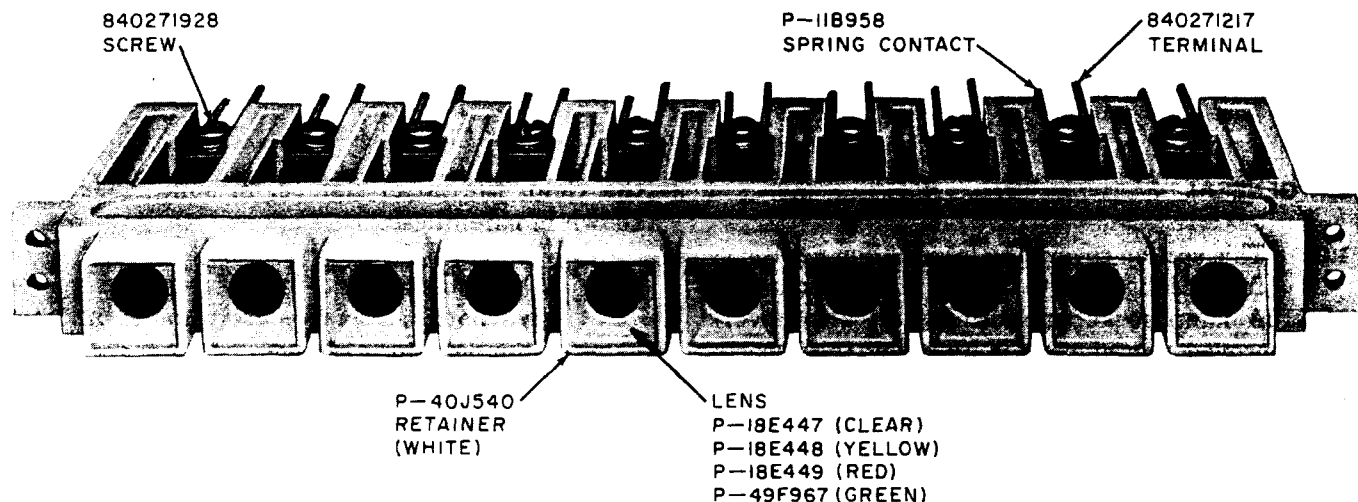
Fig. 1—310A Lamp Socket Mounting
