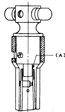
Fig. 5 - 406-type Key
