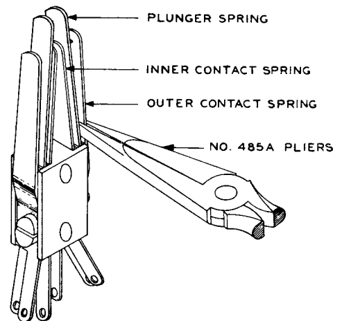
Fig. 21 - Method of Adjusting Contact Springs
