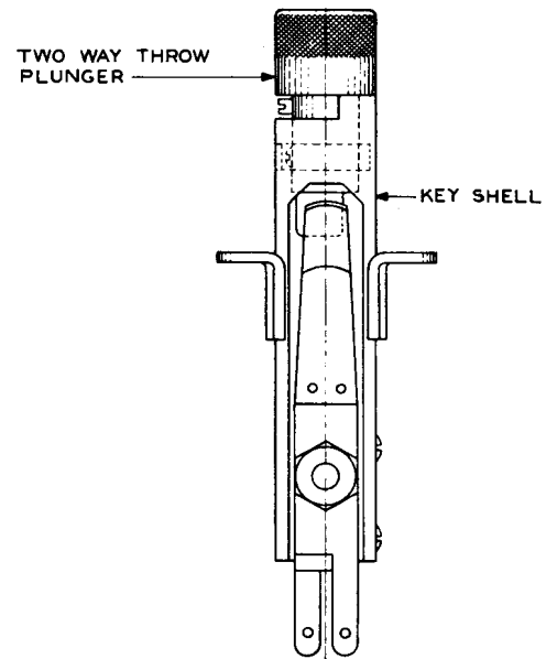
Fig. 4 - 498-type Key
