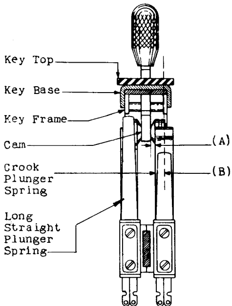
Fig. 11 - Relation of Plunger Springs to Cam and Key Frame
