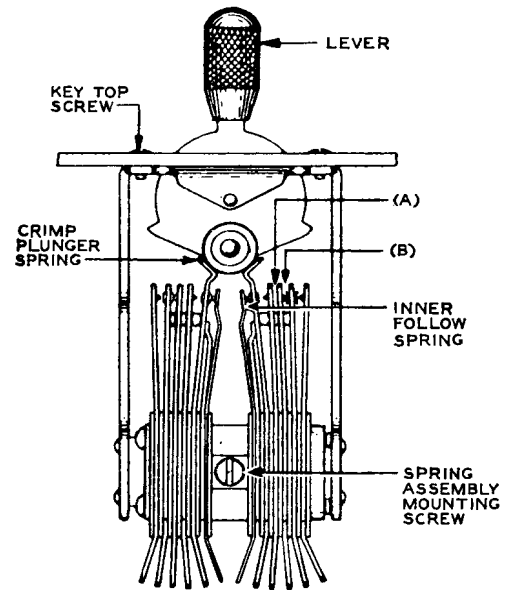
Fig. 16 - Spring Clearance
