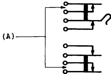
Fig. 15 - Contact Separation
