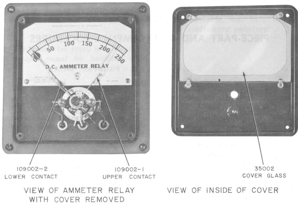
Fig. 2—KS-15802 Ammeter Relay
