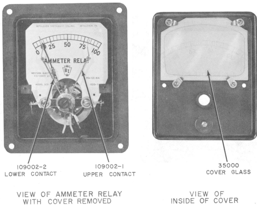
Fig. 3—KS-15803 Ammeter Relay
