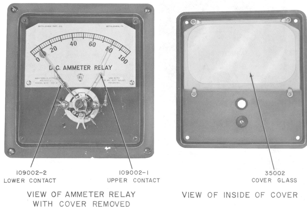
Fig. 1—KS-5662 Ammeter Relay
