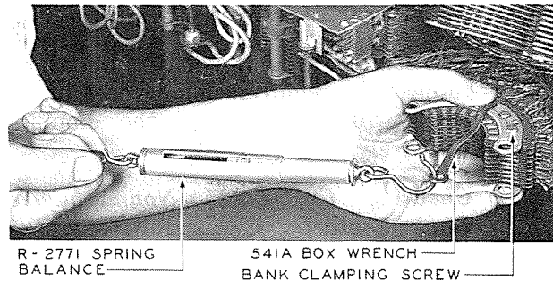
Fig. 4 – Method of Checking Tightness of Bank Clamping Screws on Mechanized Bank
