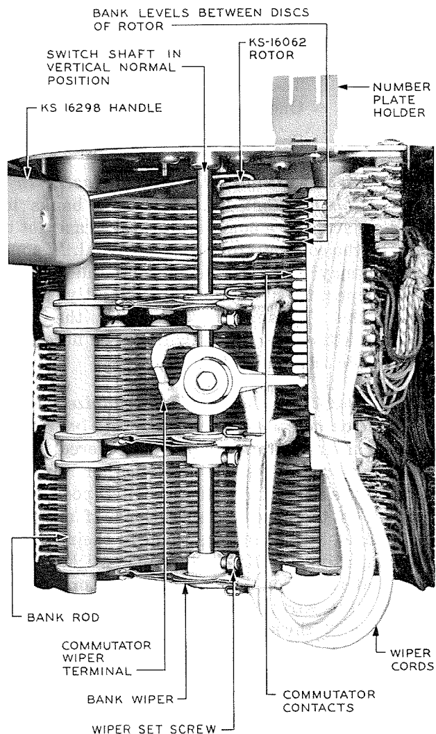
Fig. 2 — KS-16062 Rotor at Right End of Upper Half of Bank
