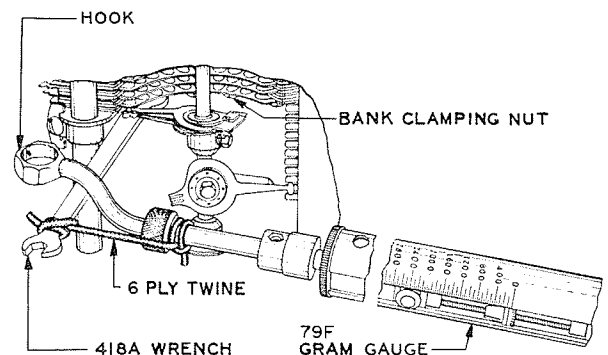
Fig. 5 – Method of Checking for Tightness of Bank Clamping Nuts on Nonmechanized Banks Using 418A Wrench and 79F Gram Gauge
