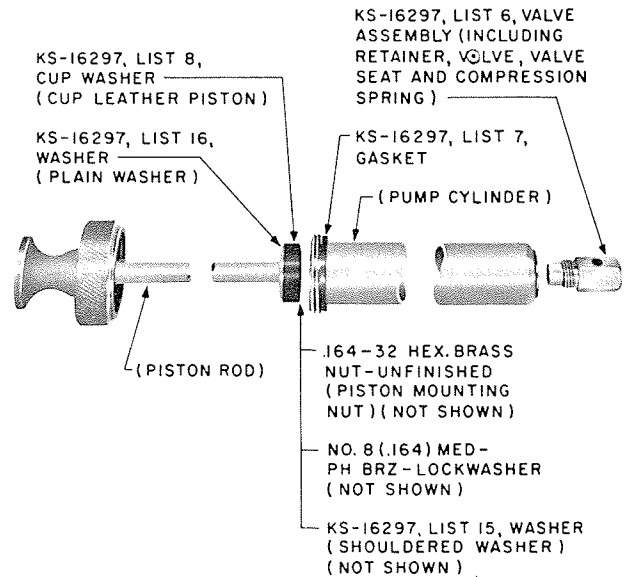
Fig. 14 – Replaceable Parts of KS-16297 L9 Pump Assembly
