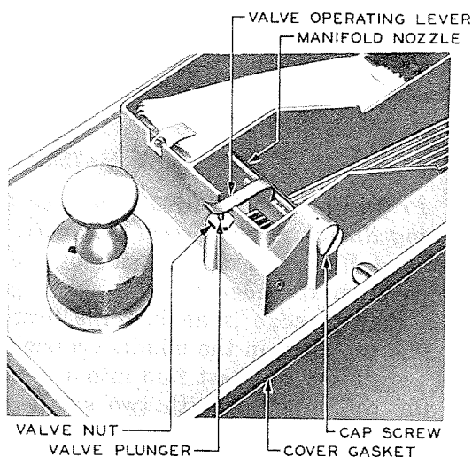
Fig. 7 – Partial View of KS-16297 L1 Flushing Unit Showing Manifold Nozzle and Associated Parts
