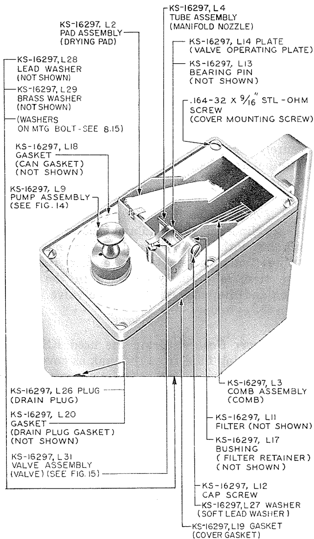
Fig. 13 – Replaceable Parts of KS-16297 L1 Flushing Unit
