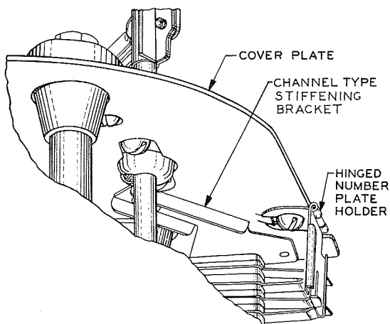
Fig. 1 — Channel-Type Stiffening Bracket on Coverplate
