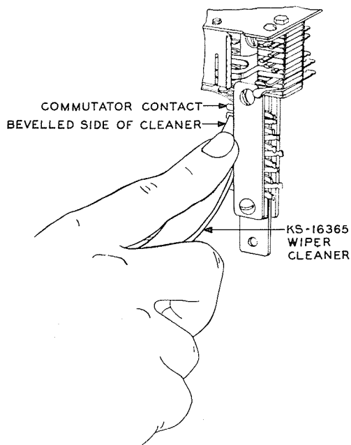
Fig. 3 – Method of Nonabrasively Cleaning Commutator Contacts
