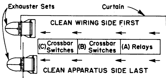
Fig. 1—Curtain Enclosed Frame With Exhaustor Sets in Place
