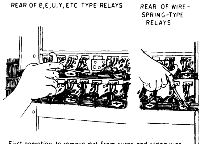
Fig. 4—Method of Directing Nozzle for Cleaning Rear of B-, E-, U-, Y-, etc., and Wire-Spring Type Relays
