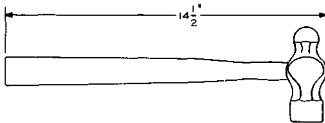
HAMMER, BALL PEEN, 1-POUND
