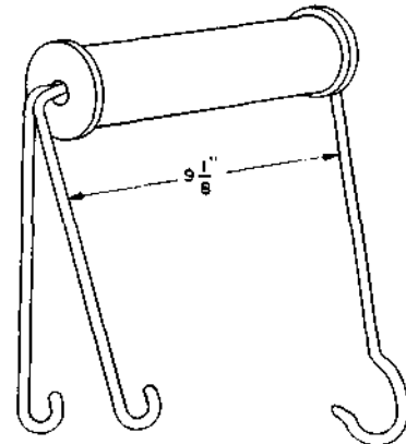
HANDLE, CARRYING, KS-5299
