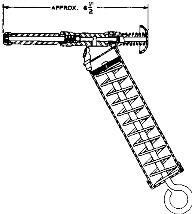
GUN, GREASE, LINCOLN ENGINEERING COMPANY, 5958
