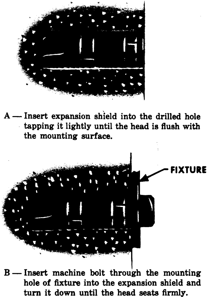
Fig. 2 — Installation
