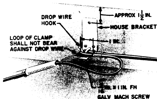
Fig. 2 — Drop Wire Hook and House Bracket (First Attachment)
