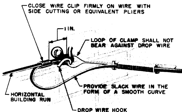
Fig. 1 — First Attachment — Drop Wire Hook
