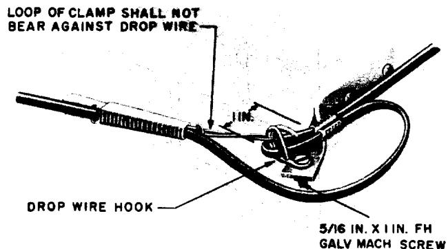
Fig. 4 — Drop Wire Hook and Corner Bracket (To Clear Corner of Building)
