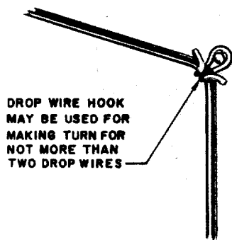
Fig. 3 — Drop Wire Hook (Intermediate Attachment)
