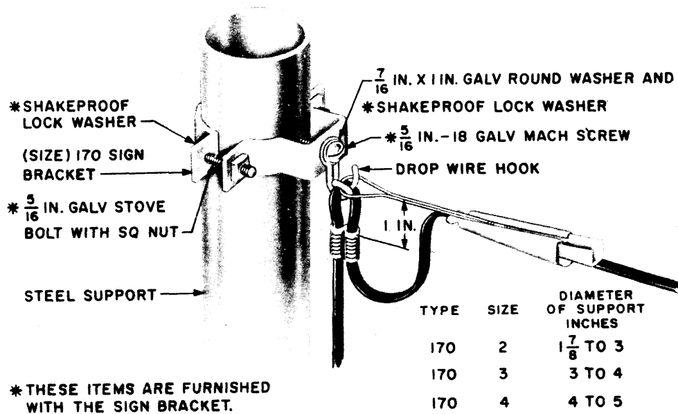
Fig. 1 — First Attachment, Sign Bracket, 170 Type
