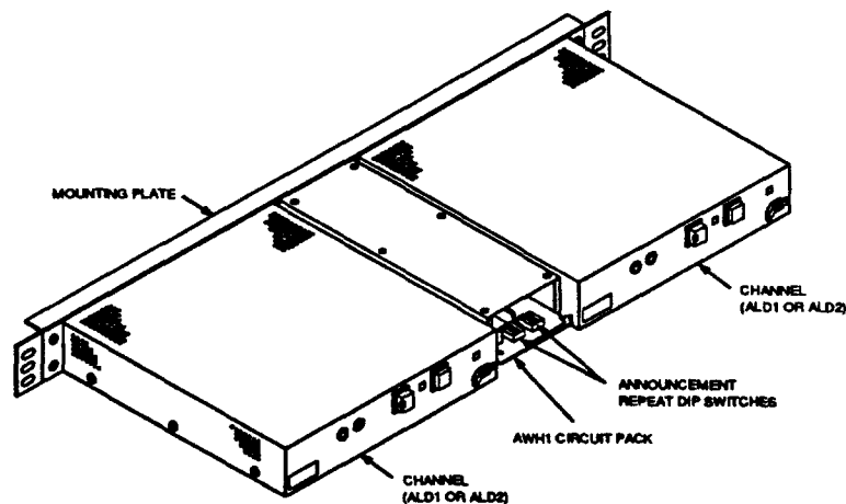
Figure 5. 14A Announcement System Equipped With Two Channels and AWH1 Circuit Pack for 2-Wire Telephone Line Connection
