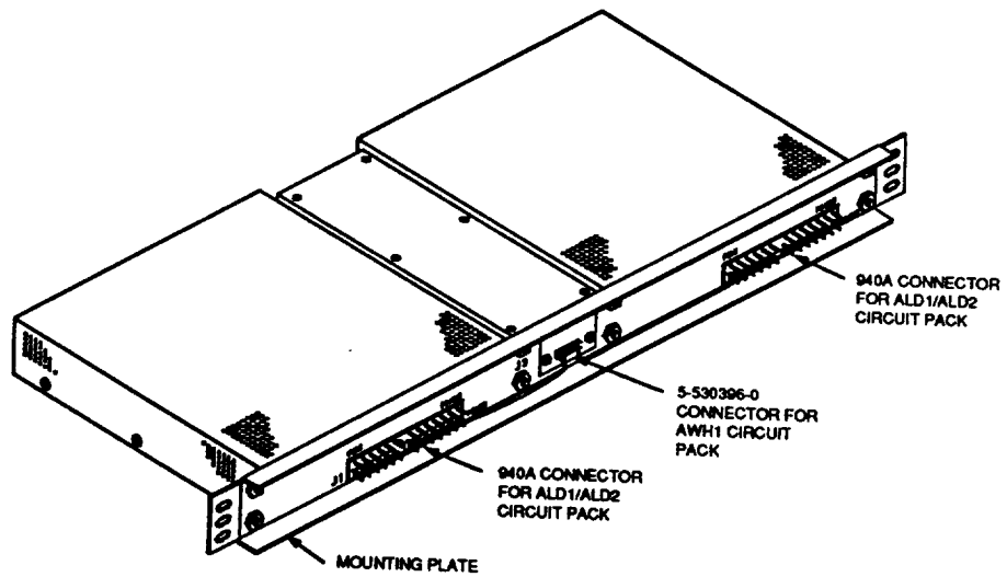
Figure 7. 14A Announcement System Rear Mounting Plate
