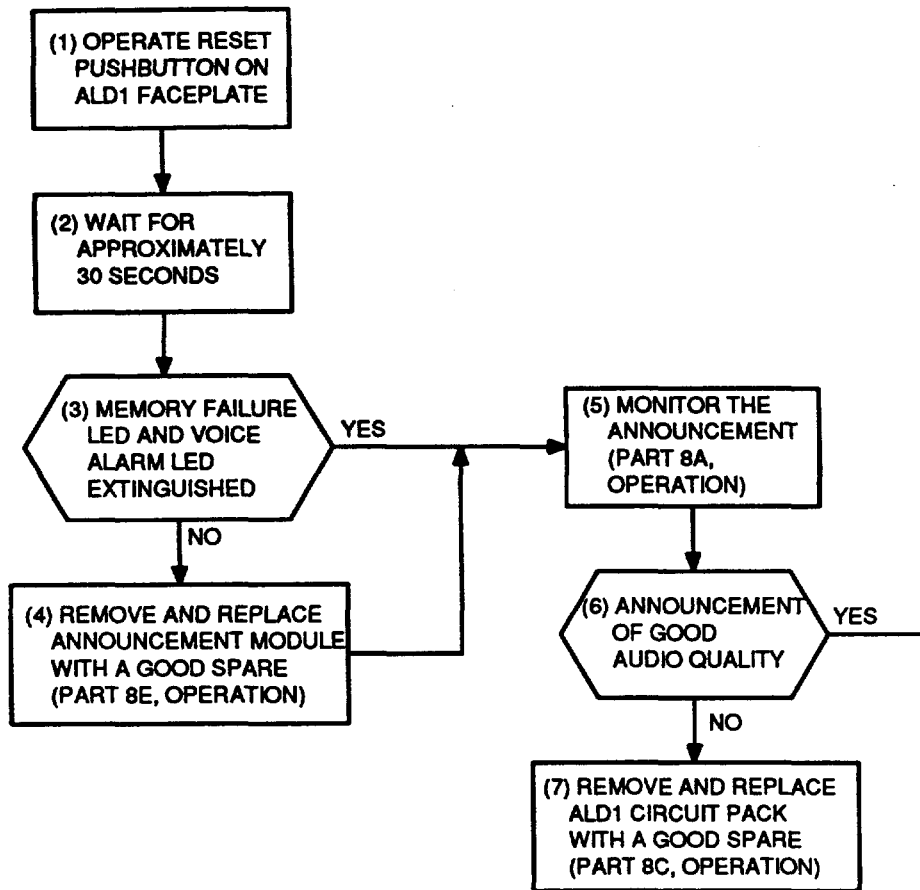
Figure 14. ALD1 Memory Failure LED and Voice Alarm LED Flowchart
