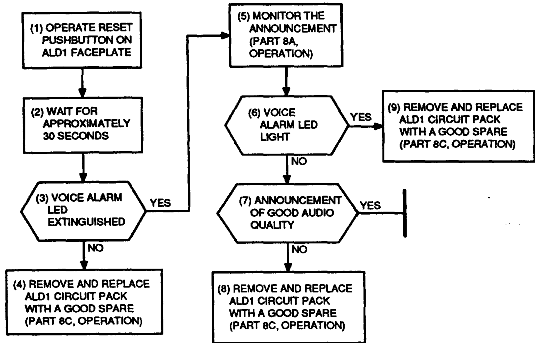
Figure 13. ALD1 Voice Alarm LED Flowchart
