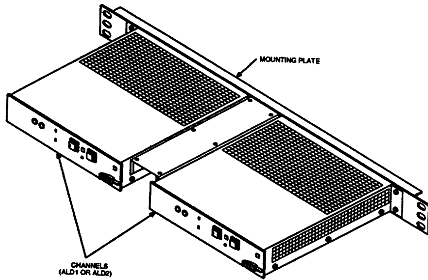
Figure 6. 14A Announcement System Equipped With Two Channels for Announcement Trunk Connection
