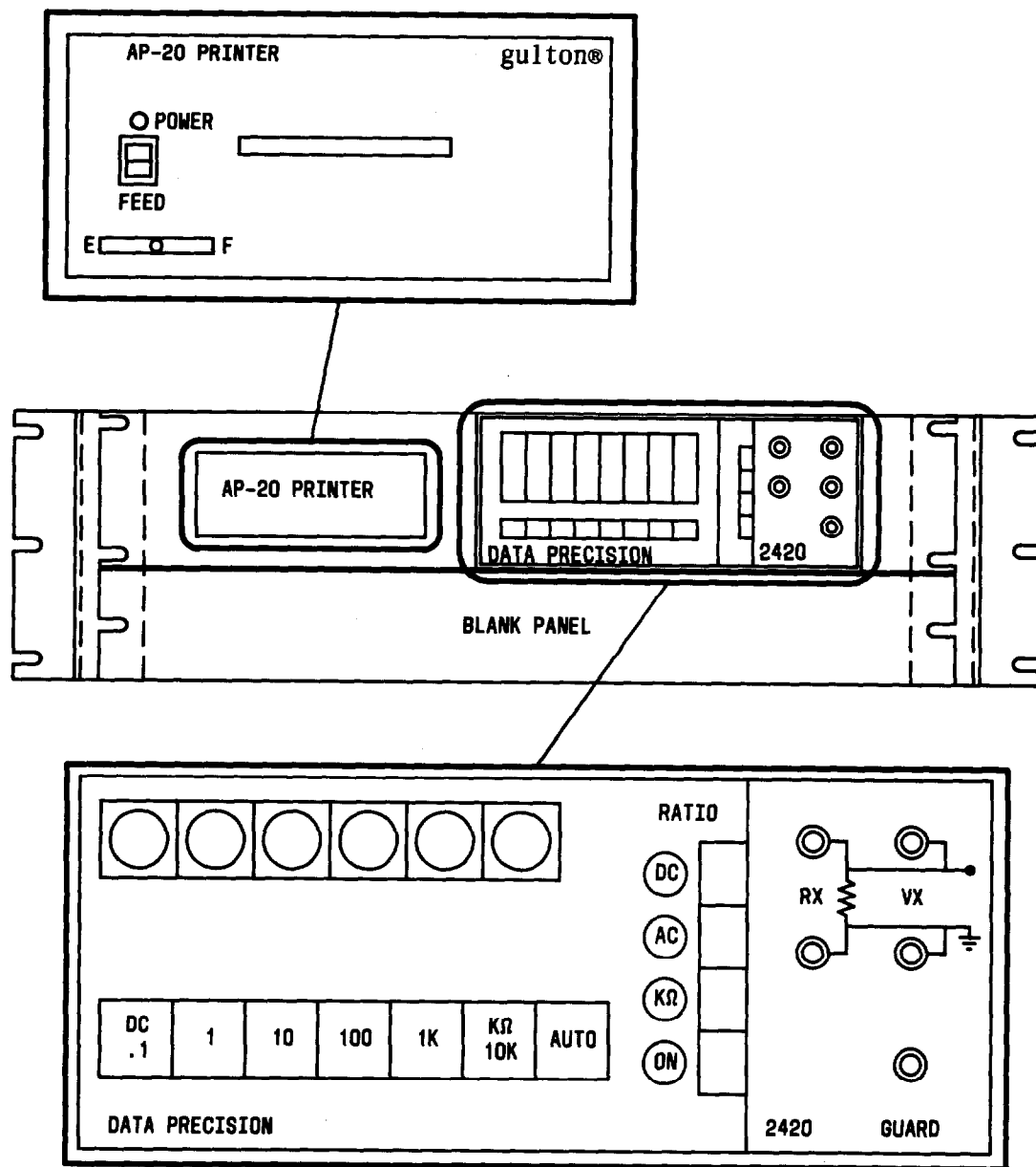
▶Fig. 6—Part of Central Control Panel Showing Digital Volt-Ohmmeter and Thermal Printer◀
