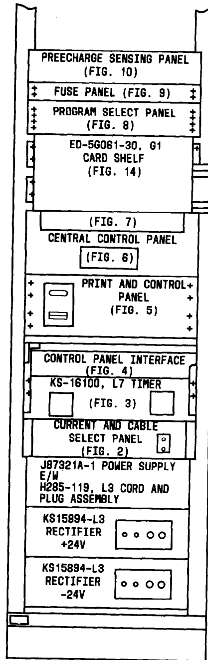
Fig. 1—Central Control Bay
