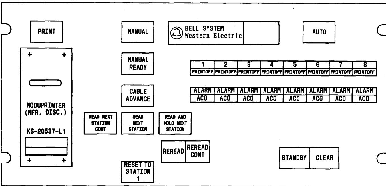
Fig. 5—Print and Control Panel
