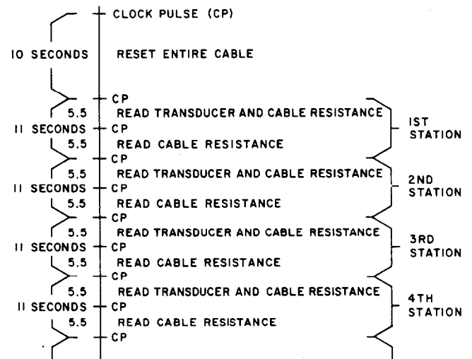
Fig. 12—Cable Pressure Measurement Time Sequence
