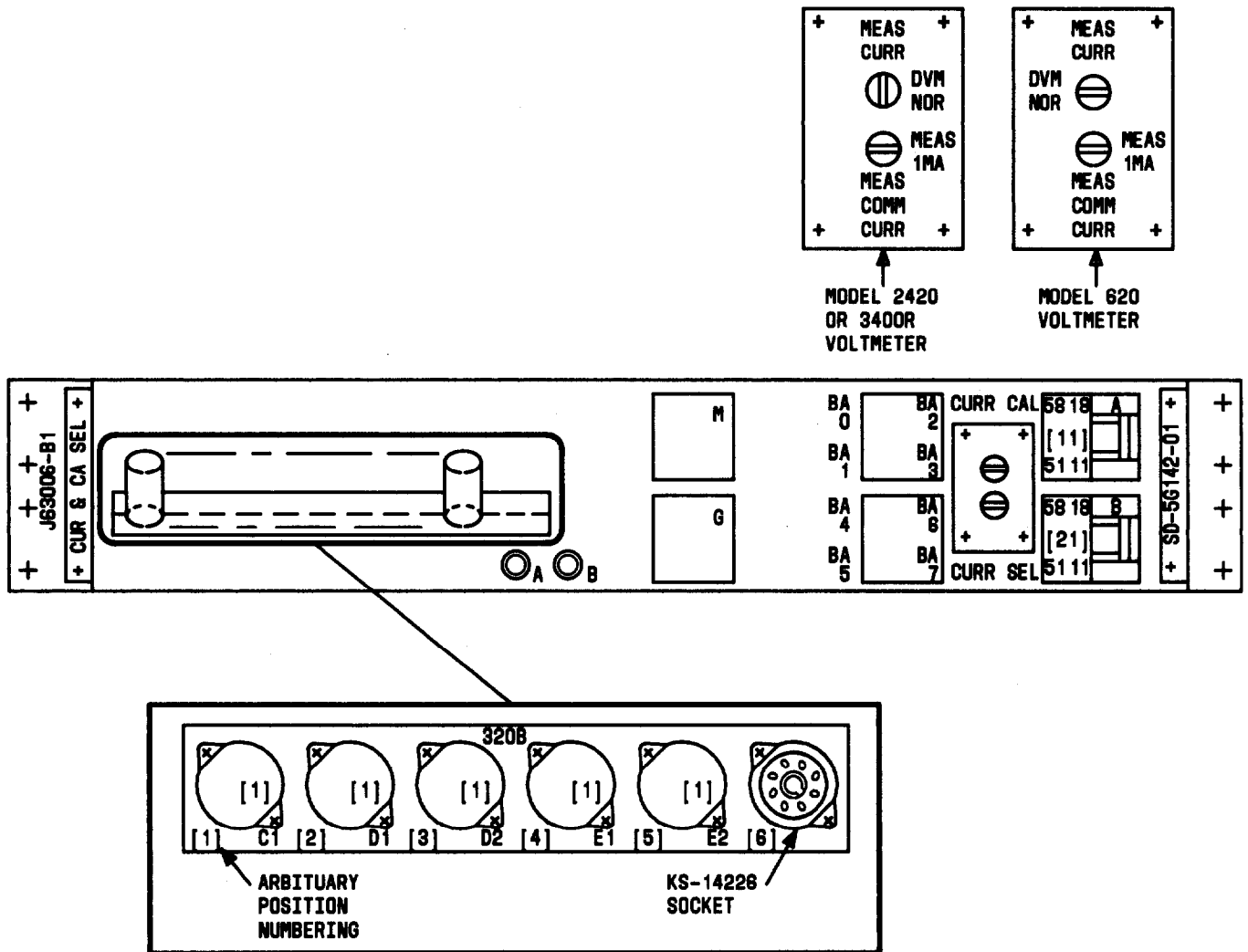
Fig. 2—Current and Cable Select Panel
