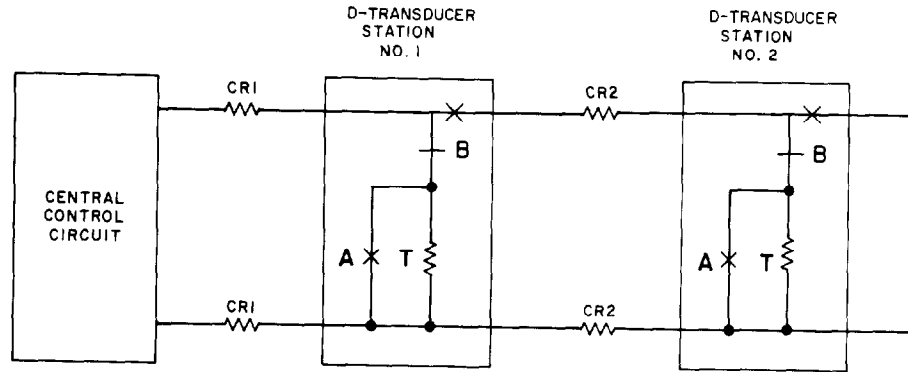
Fig. 11—D-Transducer Measurement
