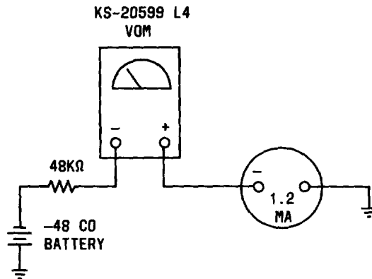
Fig. 1—Milliammeter Calibration Circuit—1.0 mA Connection
