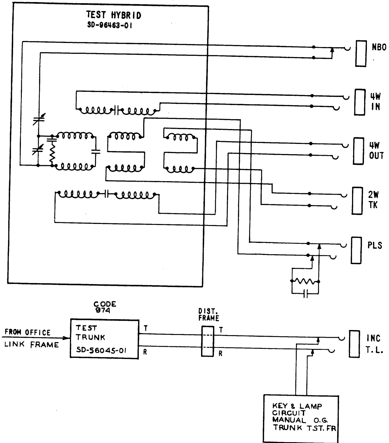
Figure 1 - Return Loss Test Equipment Arrangement at the Outgoing Trunk Test Jack Bay
