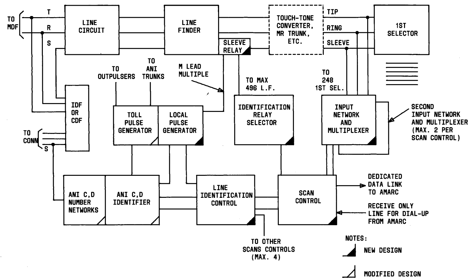
Fig. 3—Call Data Accumulator with Automatic Number Identification Types C and D (2.11, 4.06)
