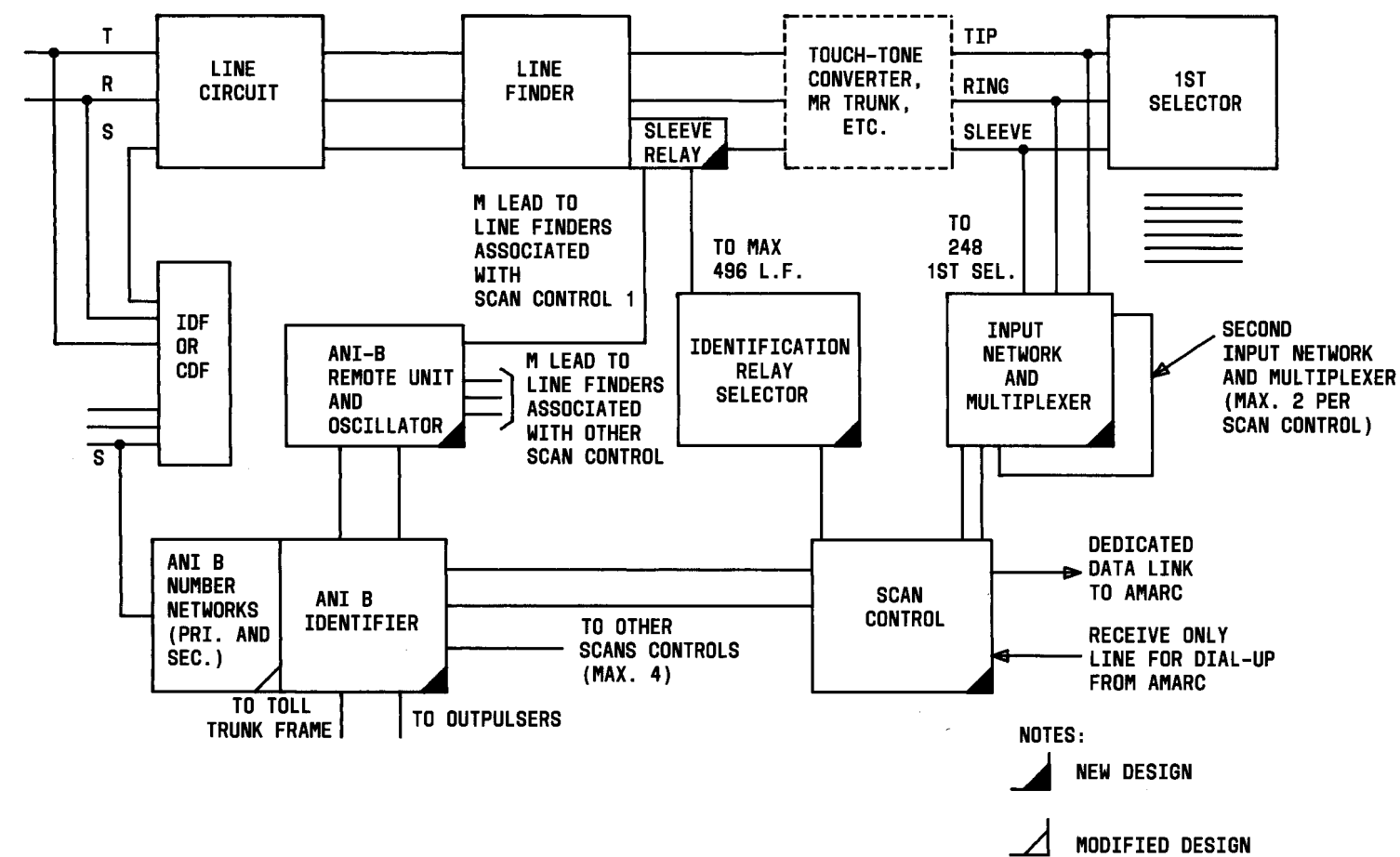
Fig. 2—Call Data Accumulator with Automatic Number Identification Type B (2.10, 4.06)
