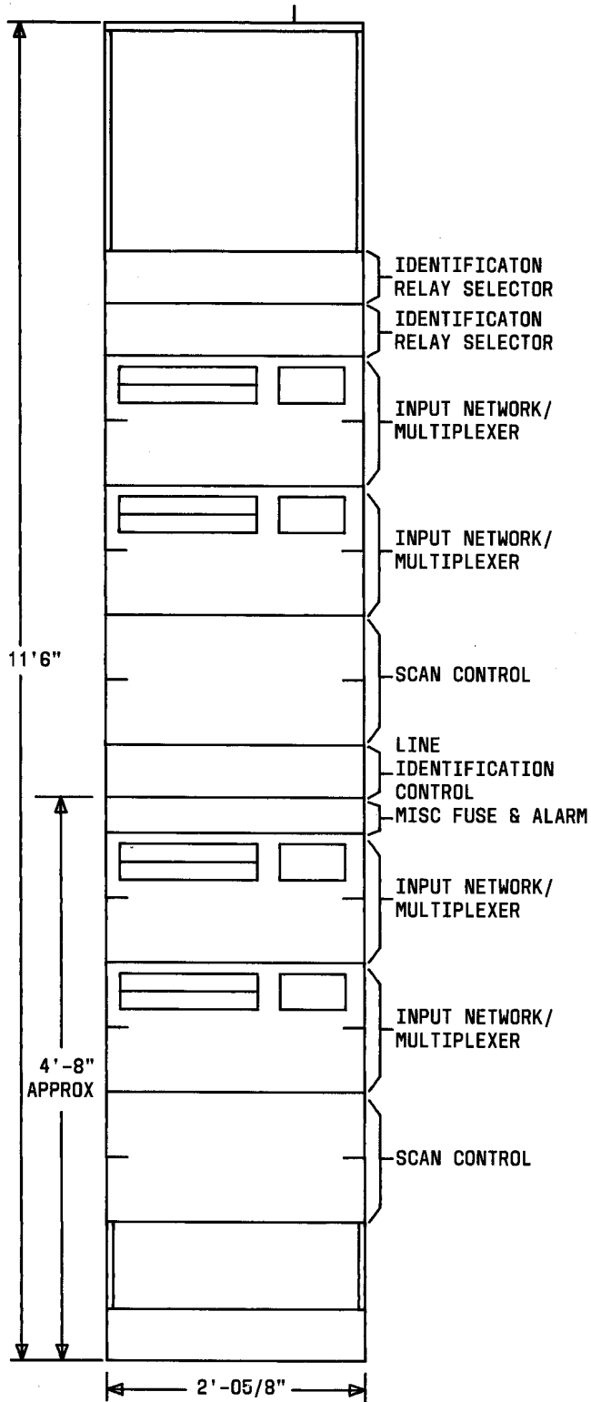
Fig. 1—Call Data Accumulator Typical Configuration (2.03)
