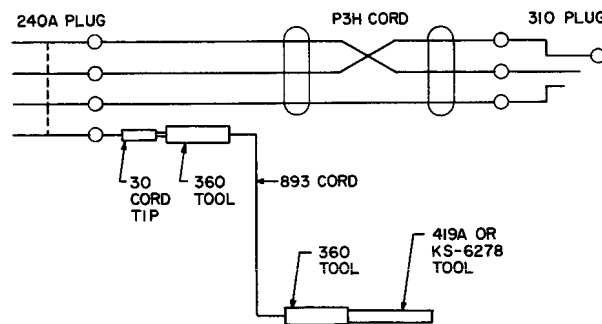
Fig. 1 — Testing Cord
