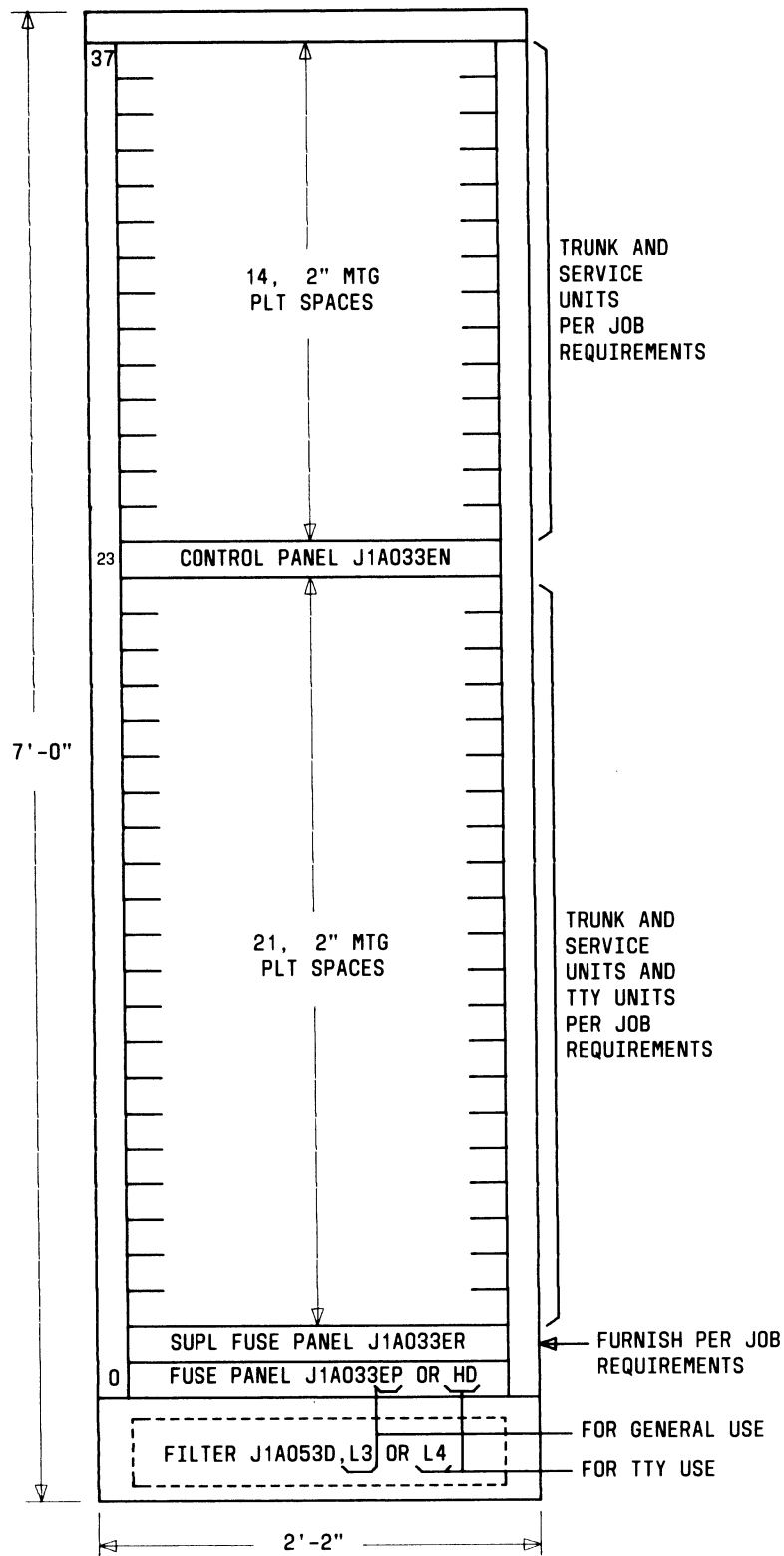
Fig. 5—Miscellaneous Trunk Frame
