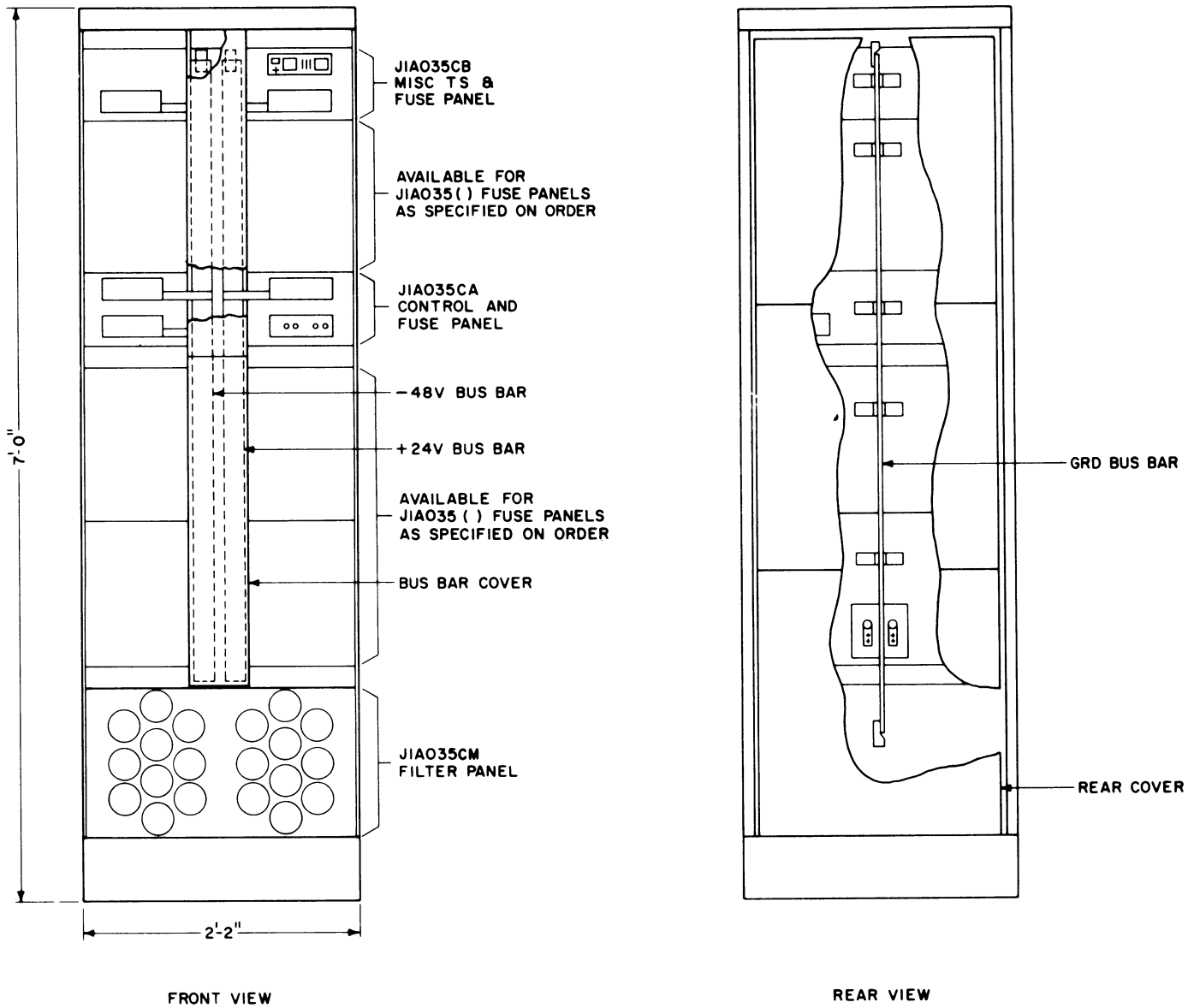
Fig. 4—Power Distributing Frame
