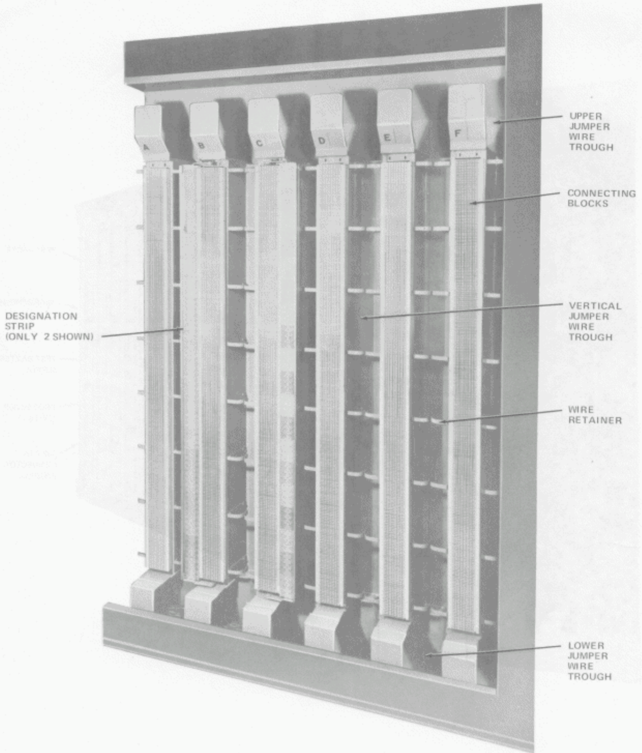
Fig. 3—Trunk Distributing Frame (or Intermediate Distributing Frame)
