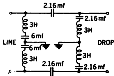
* Effect of side circuit composite sets on phantom circuits
