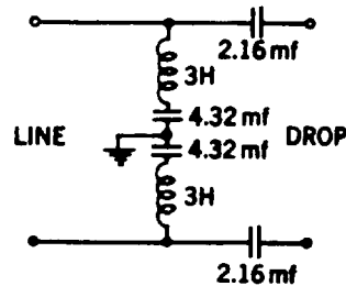
* Effect of side circuit composite sets on phantom circuits
