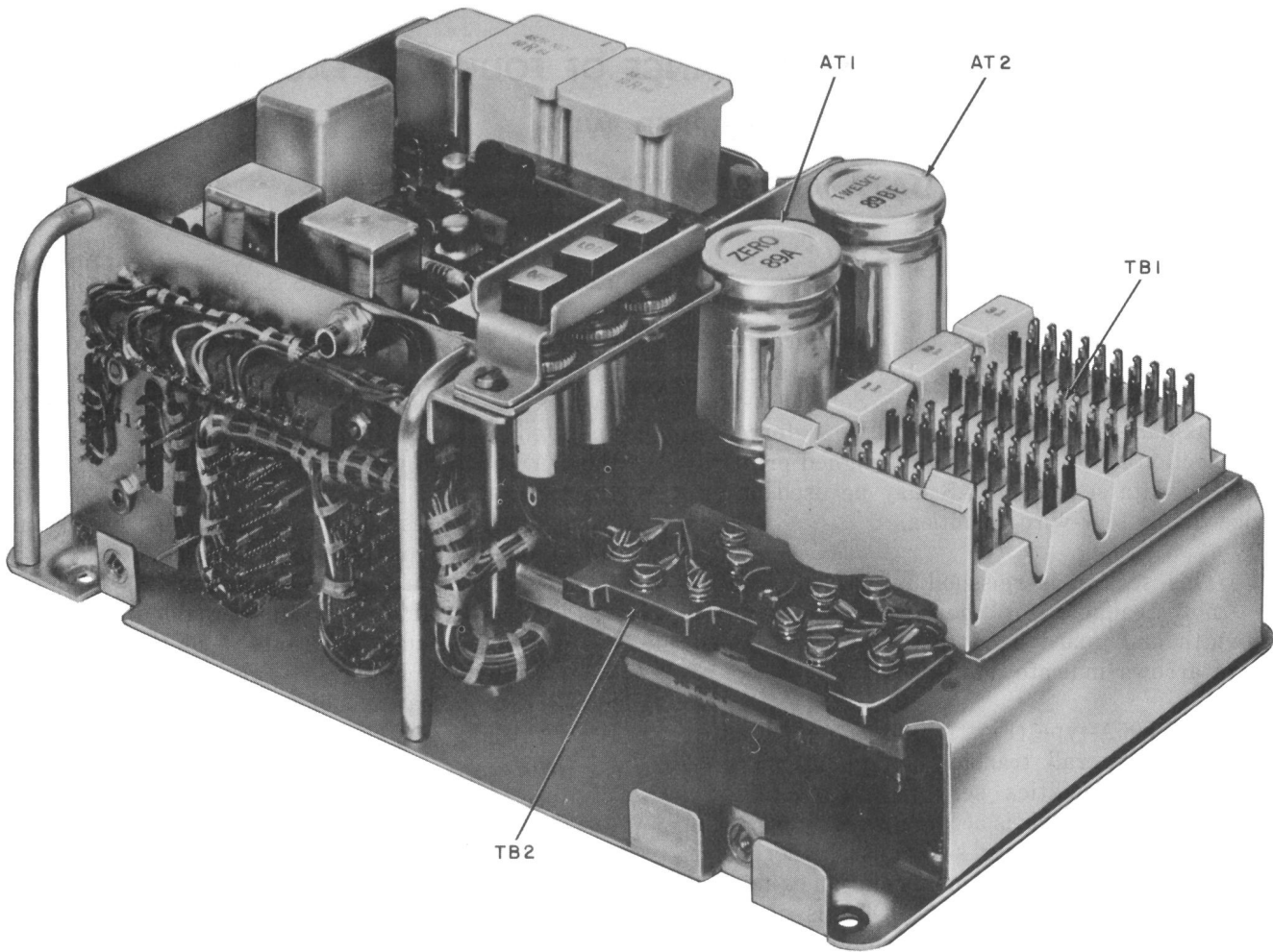
Fig. 1—Data Auxiliary Set 806A-Type—Cover Removed
