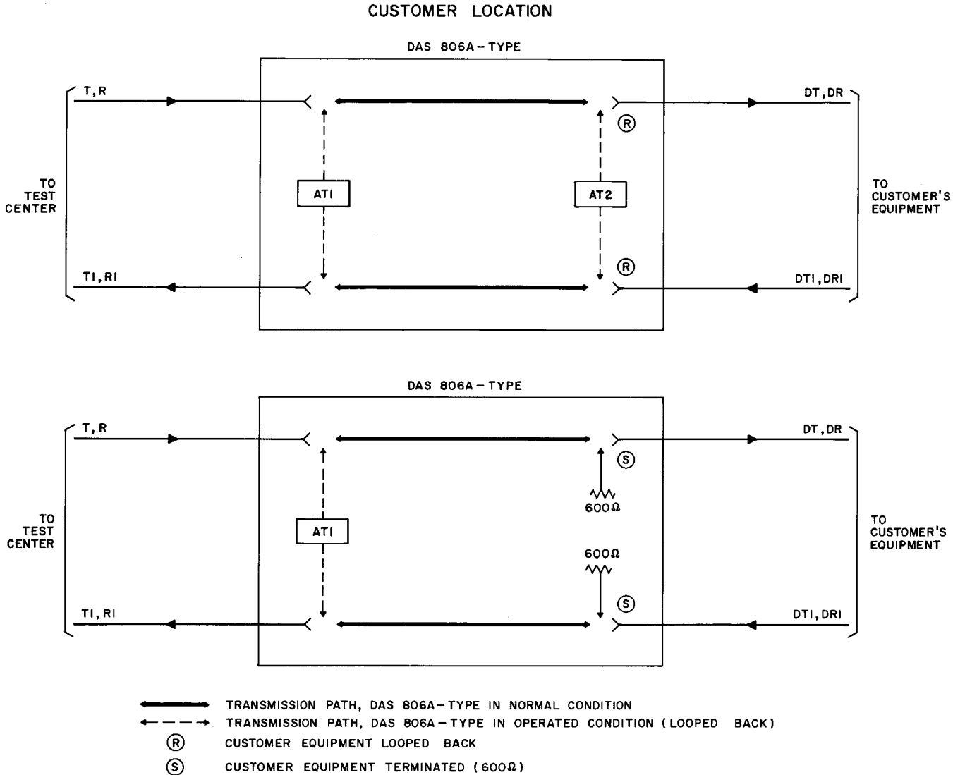
Fig. 2—Data Auxiliary Set 806A-Type—Transmission Options Under Control of Test Center
