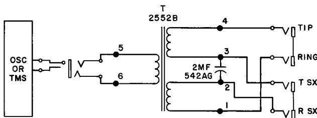
Fig. 3—Transformer Connections For Applying DAS 806A1 Operate Signal
