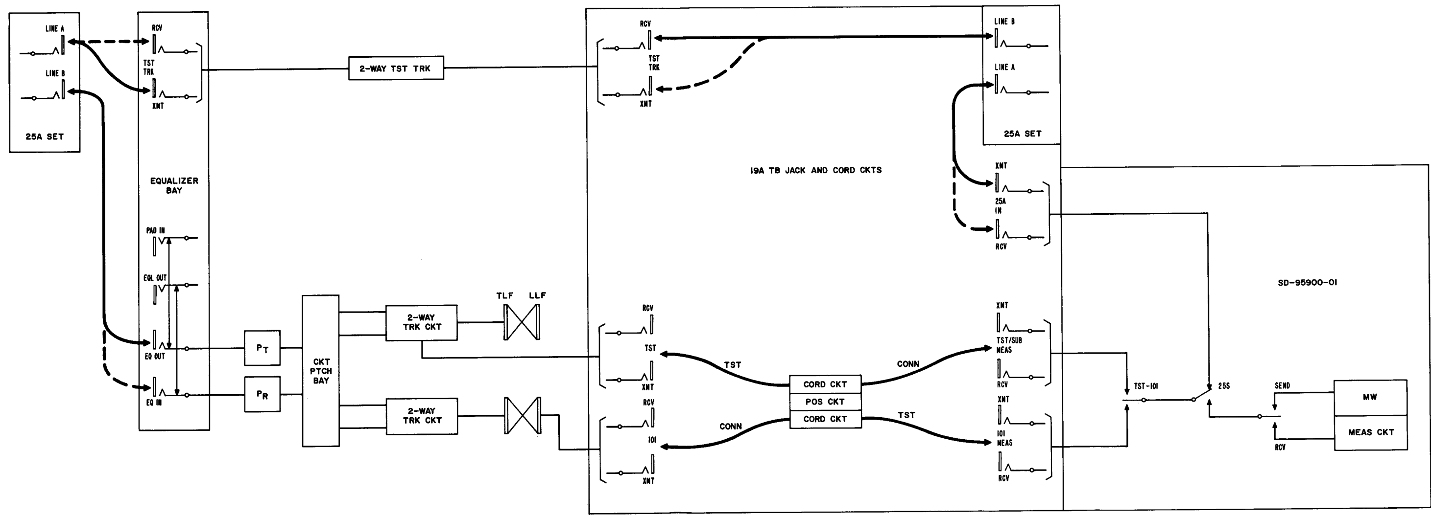
Fig. 2 — Typical Arrangement for Making Reference Measurements of Relative Envelope Delay and Frequency Response
