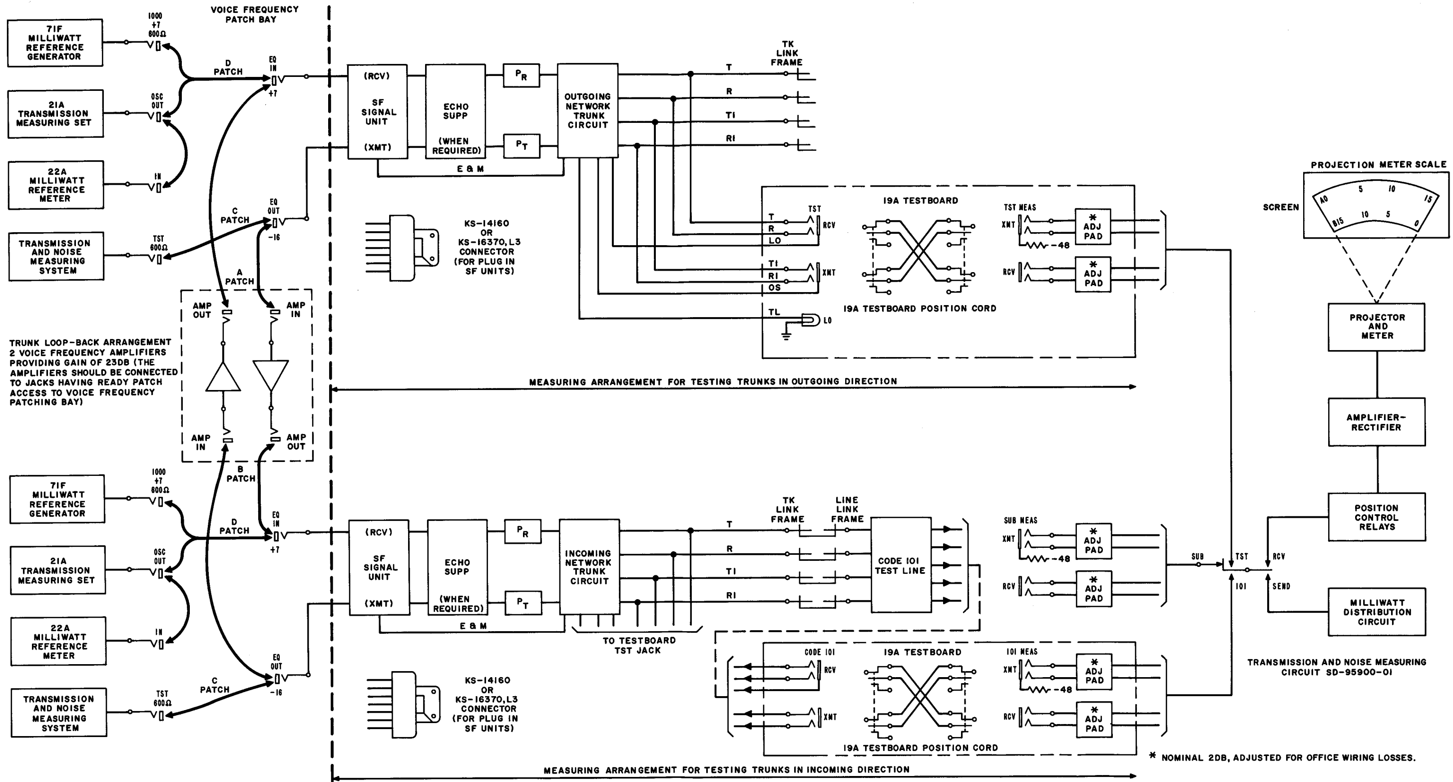
Fig. 1 — Measurement and Adjustment of Transmission Levels
