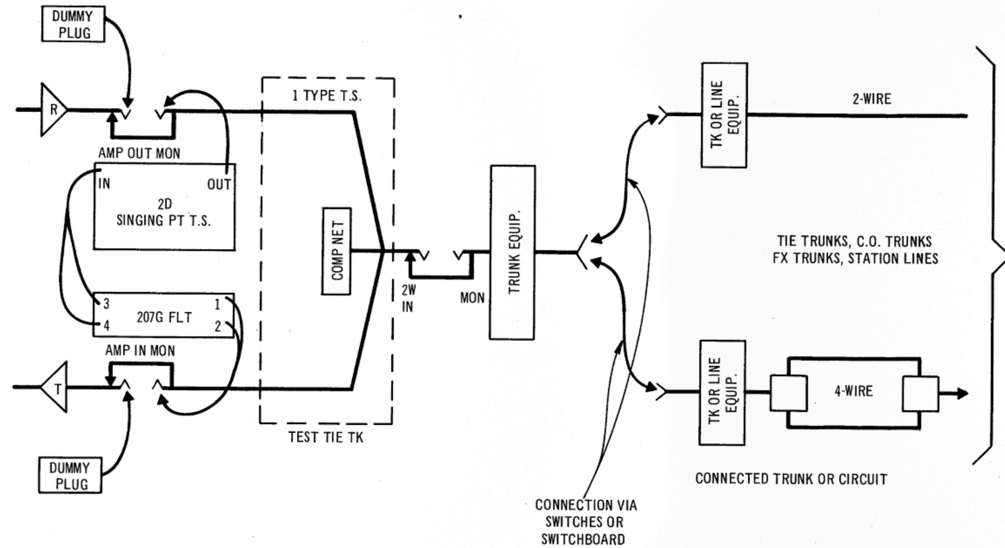
Fig. 7 - Terminal Balance Tests — Equipment Arrangement for Singing Point Test
