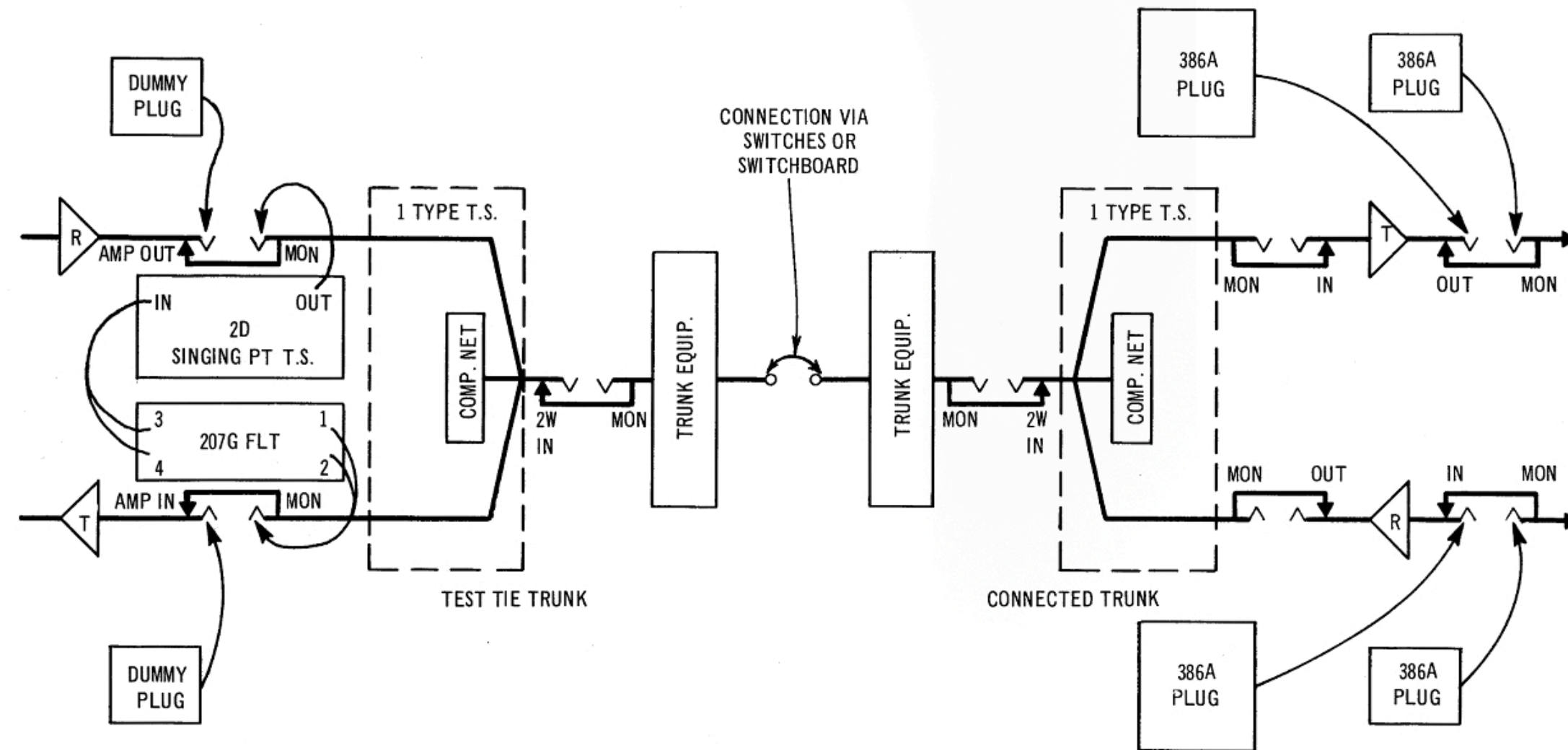
Fig. 4 - Through Balance Tests — Equipment Arrangement for Singing Point Measurement
