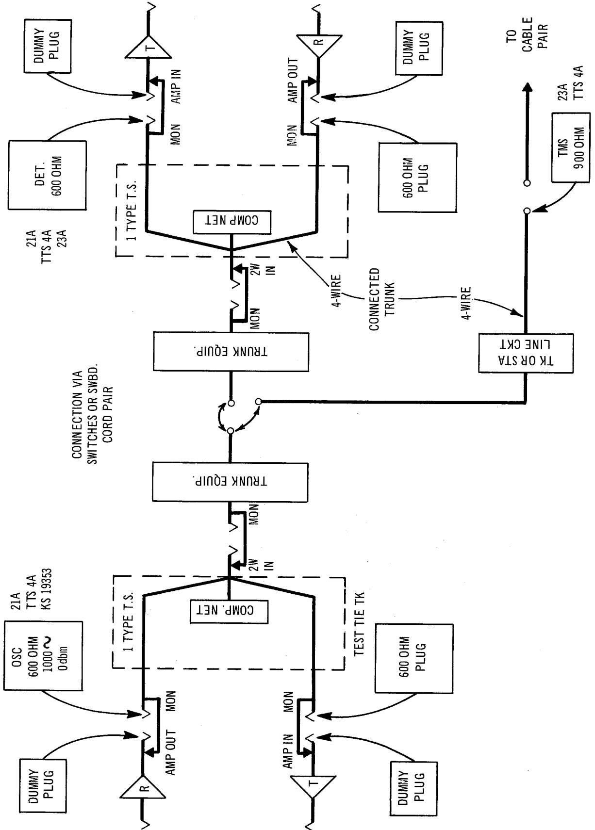
Fig. 1 -- Test Arrangement for Checking Transmission Loss of Balance Path
