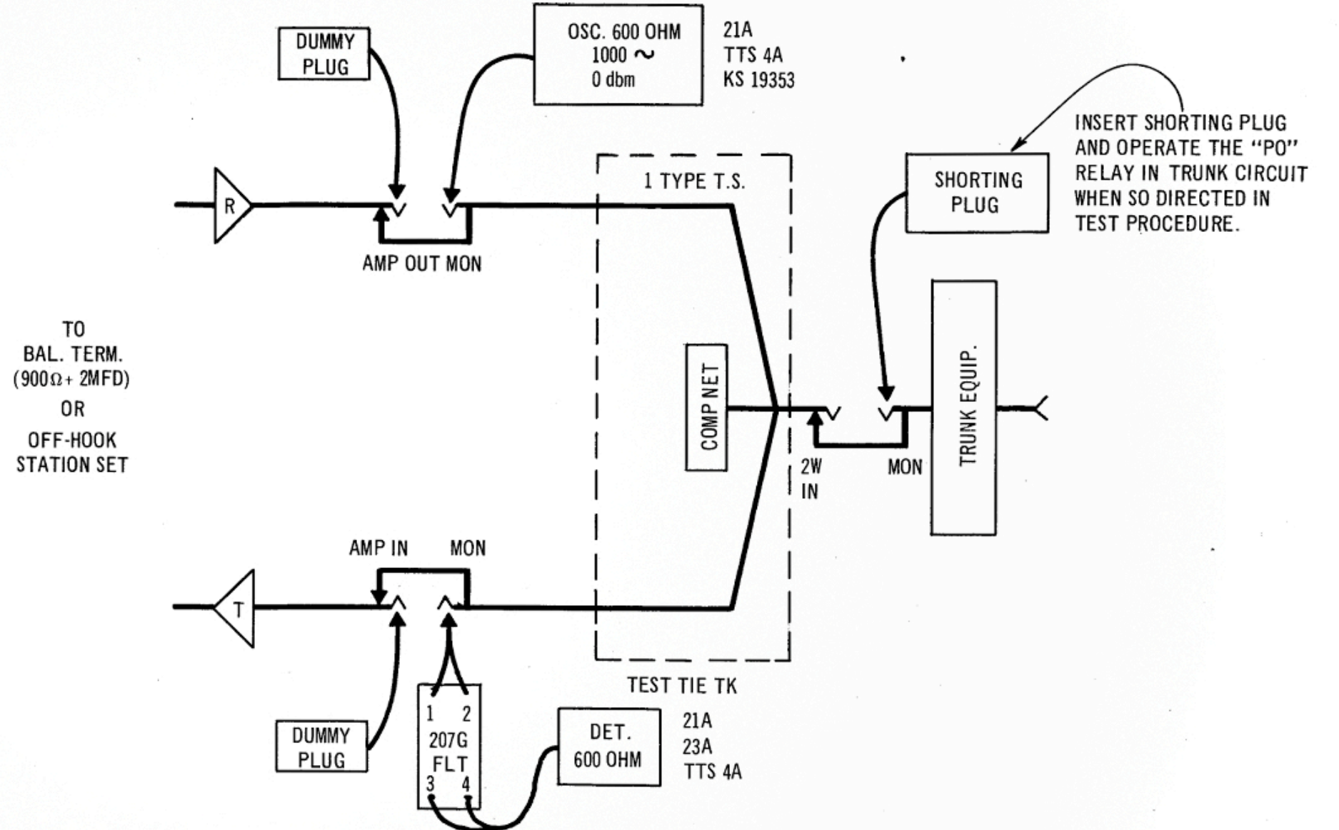
Fig. 8 - Singing Point Tests — Equipment Arrangement to Determine Hybrid Correction Factor
