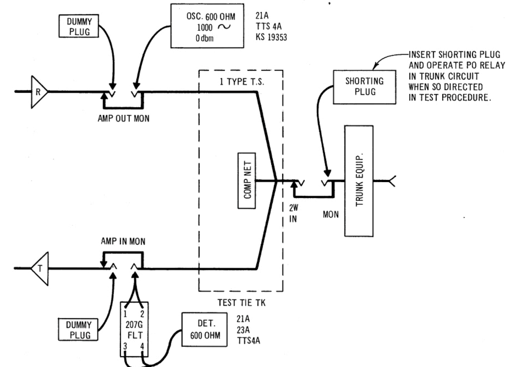
Fig. 5 - Singing Point Tests — Equipment Arrangement to Determine Hybrid Correction Factor
