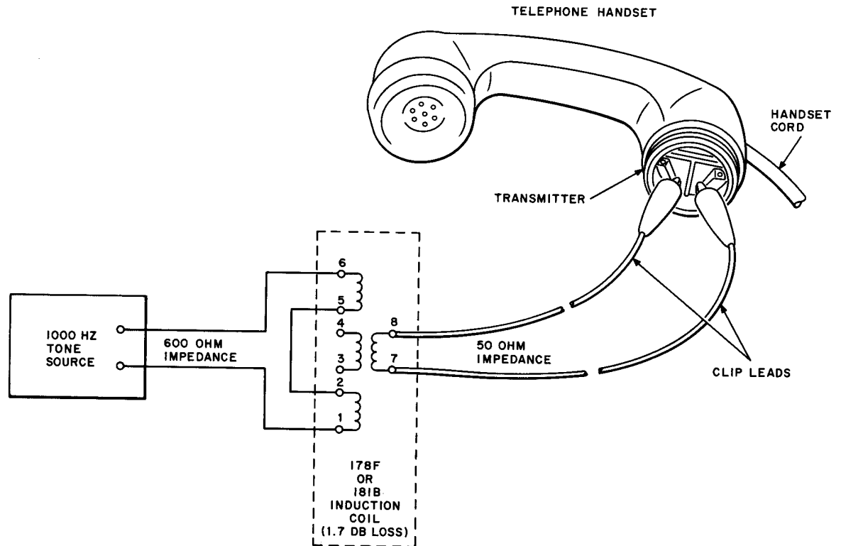
Fig. 1—Connections for Sending Tone of a Telephone Handset Transmitter
