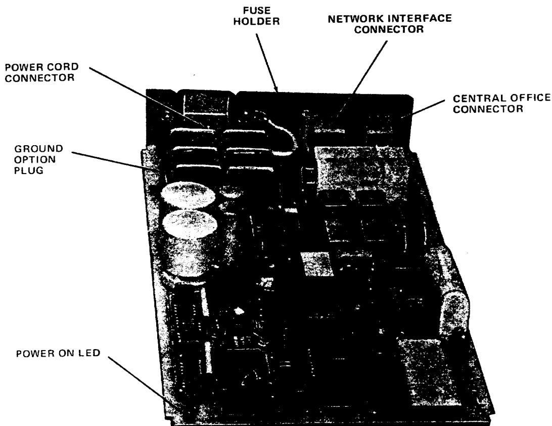
Fig. 1—554A-Type CSU—Cover Removed
