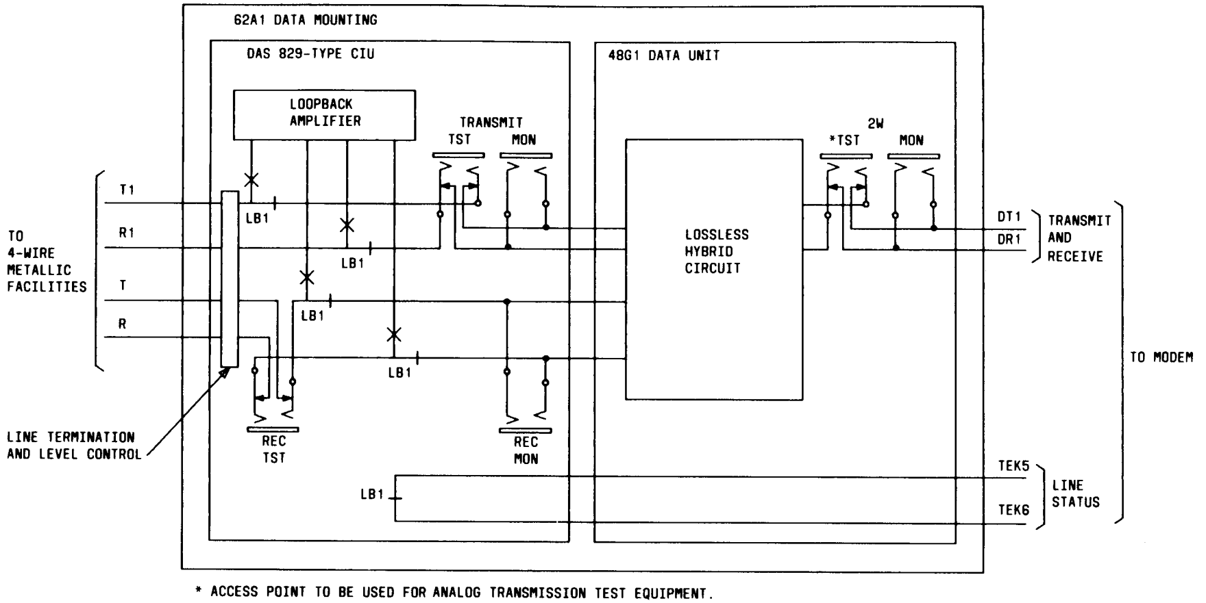
Fig. 2—Standard Circuit Design for Data Only, 2-Wire Data Set
