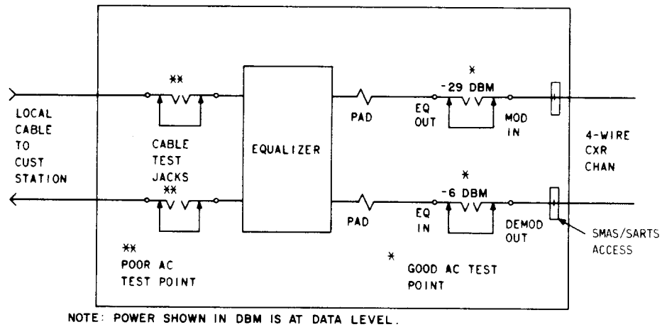
Fig. 3—Test Access Points on 4-Wire Circuit at Typical STC Office
