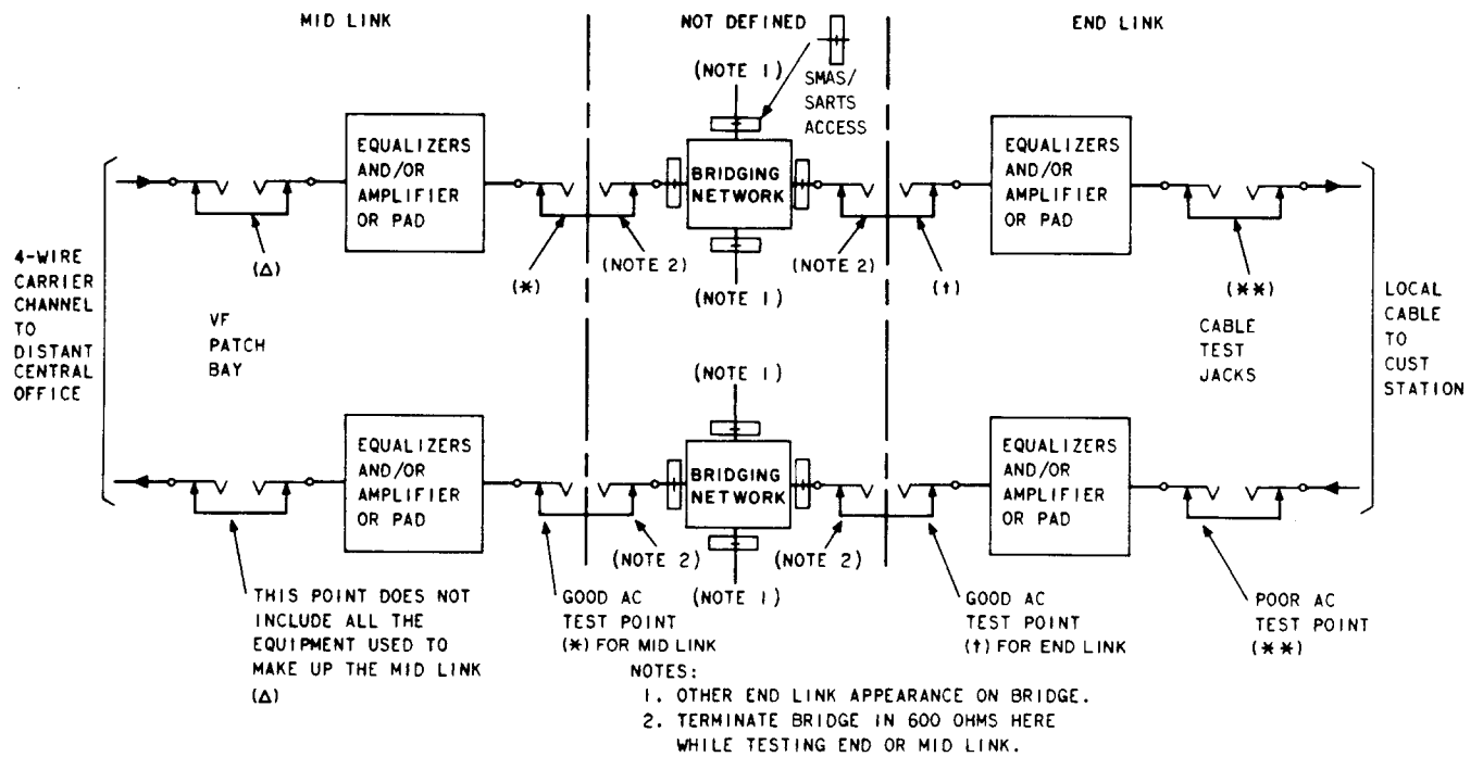
Fig. 4—Test Access Points on 4-Wire Multipoint Circuit at Bridge Location
