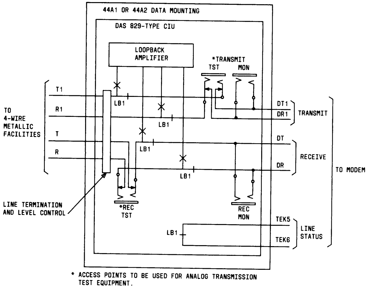
Fig. 1—Standard Circuit Design for Data Only, 4-Wire Data Set
