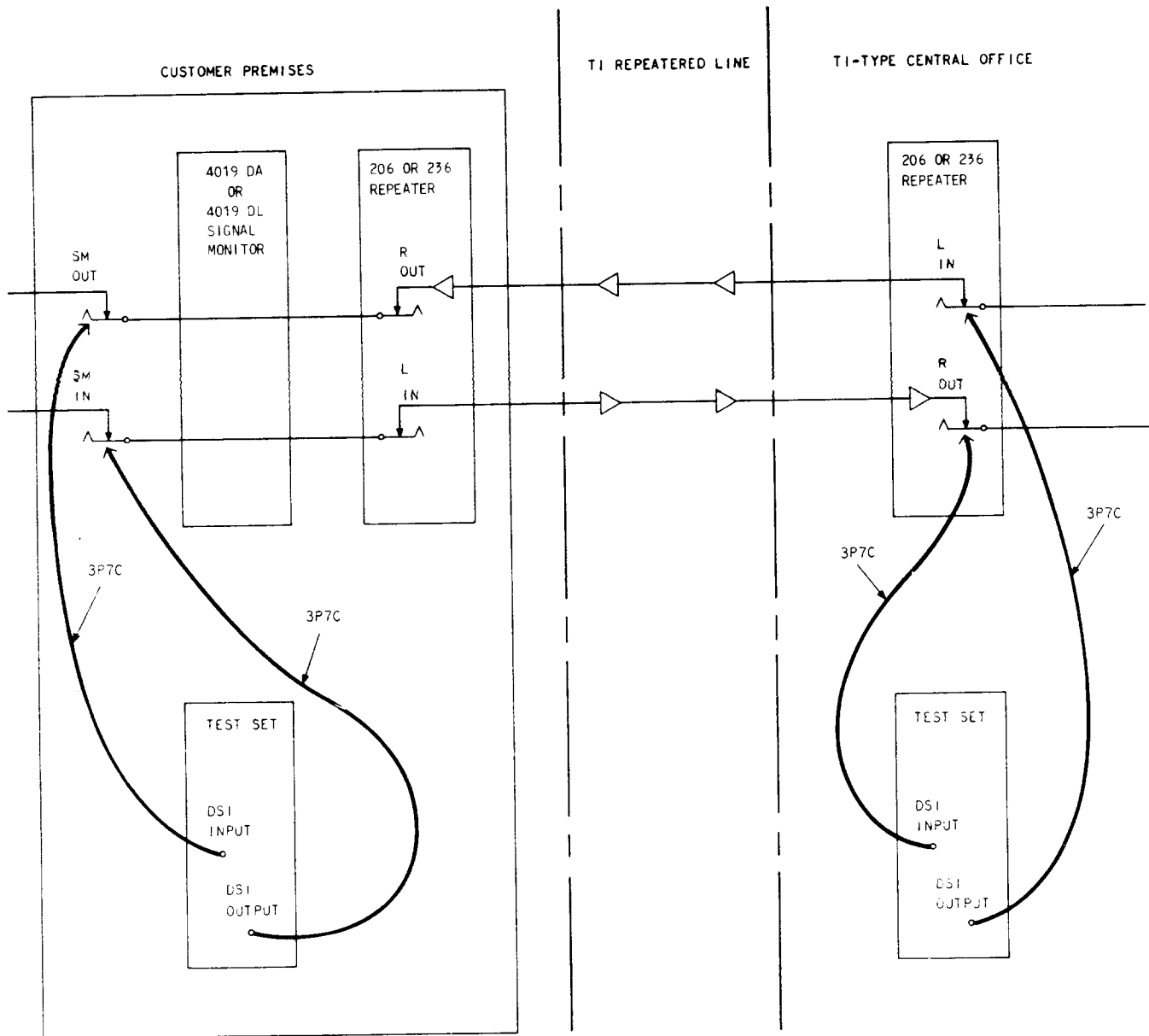
Fig. 2—Station to Central Office Testing
