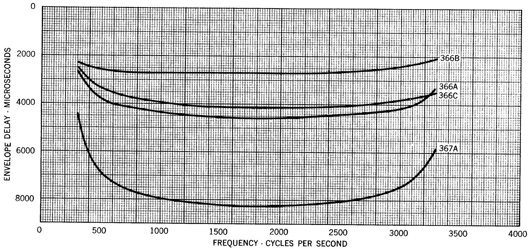
Fig. 3 – Nominal Envelope Delay Characteristics for 366- and 367-type Equalizers
