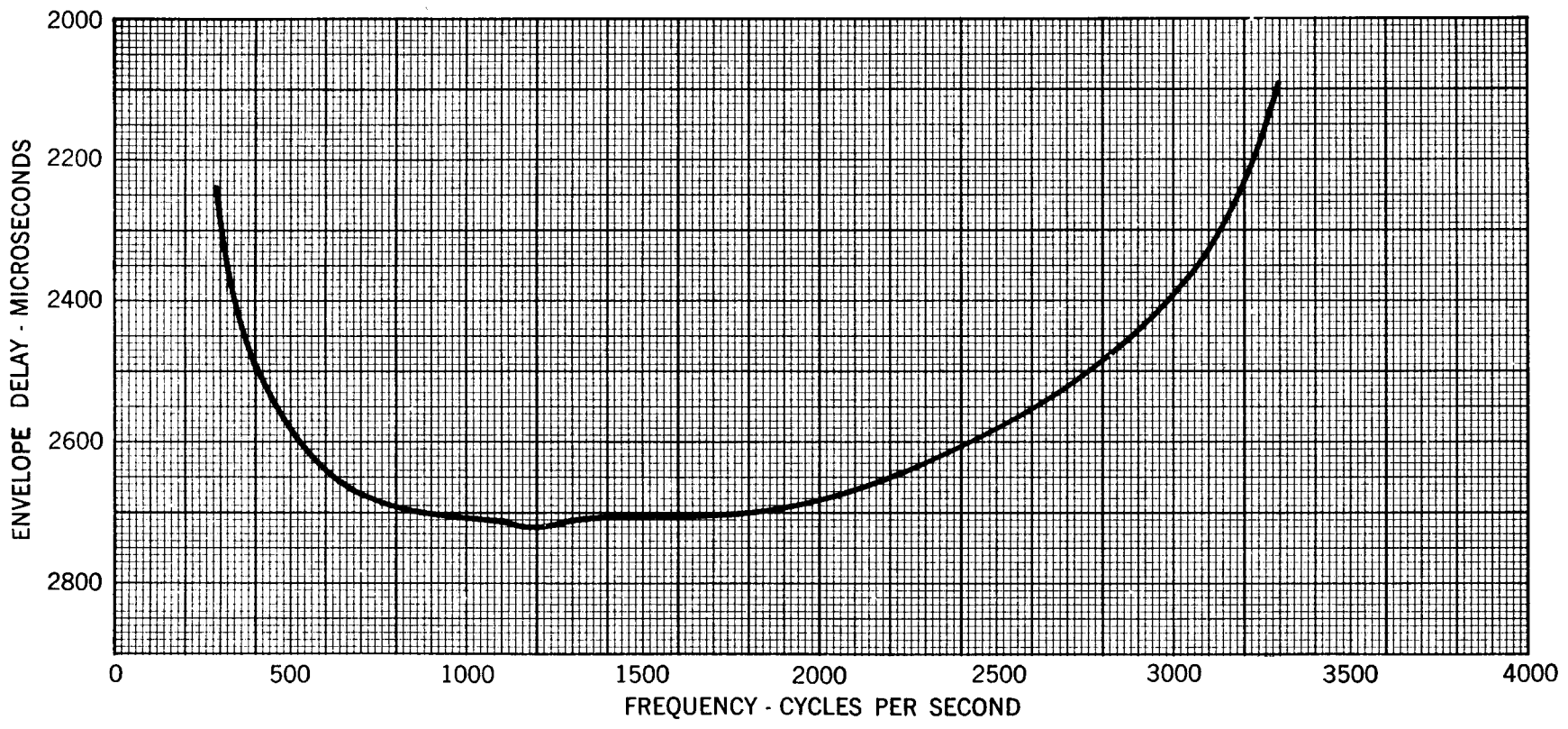
Fig. 5 – Nominal Envelope Delay Characteristic of 366B Equalizer
