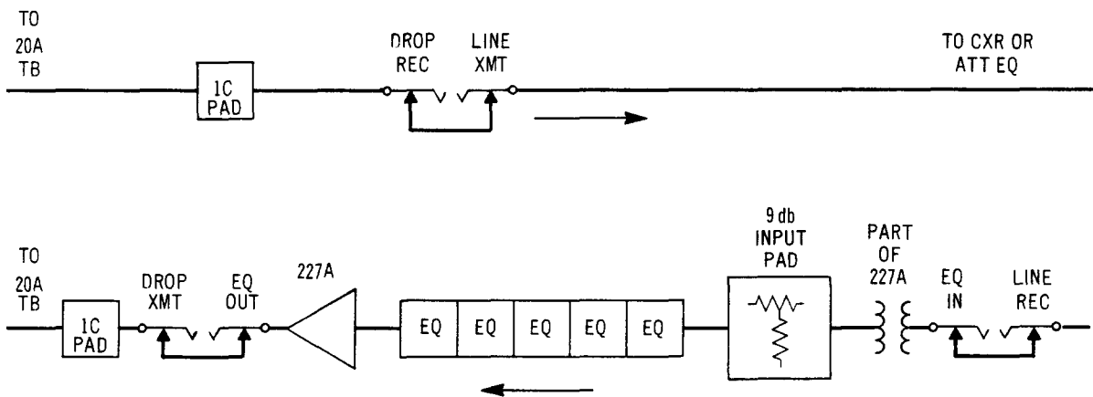
Fig. 2 - Delay Equalization Circuit
