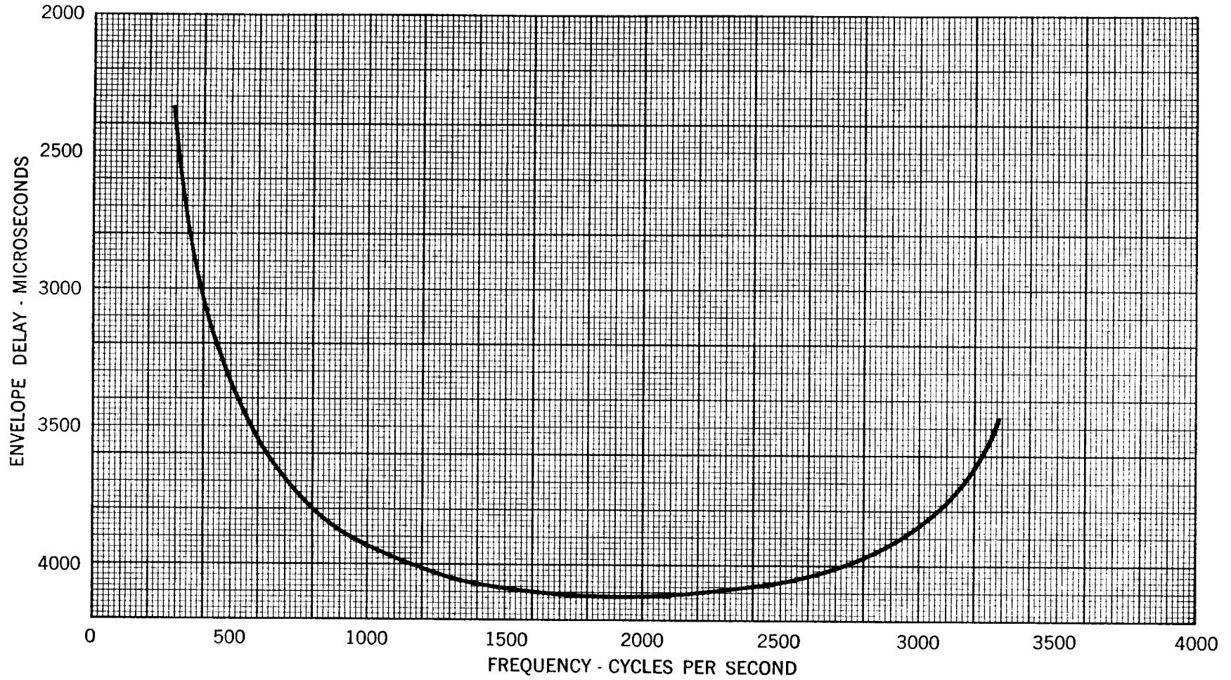
Fig. 6 – Nominal Envelope Delay Characteristic of 366C Equalizer
