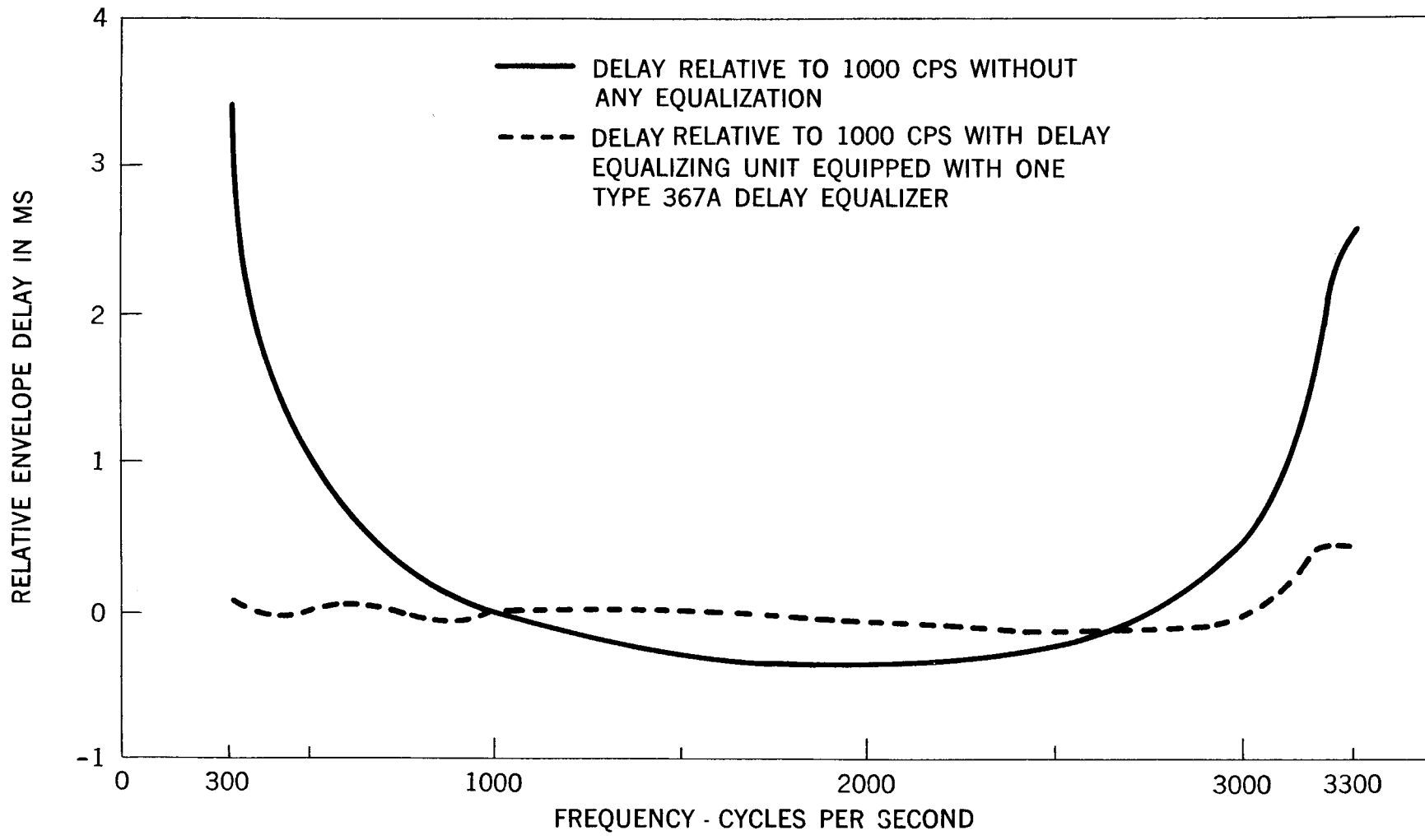
Fig. 9 - Relative Envelope Delay of Typical L Multiplex Circuit
