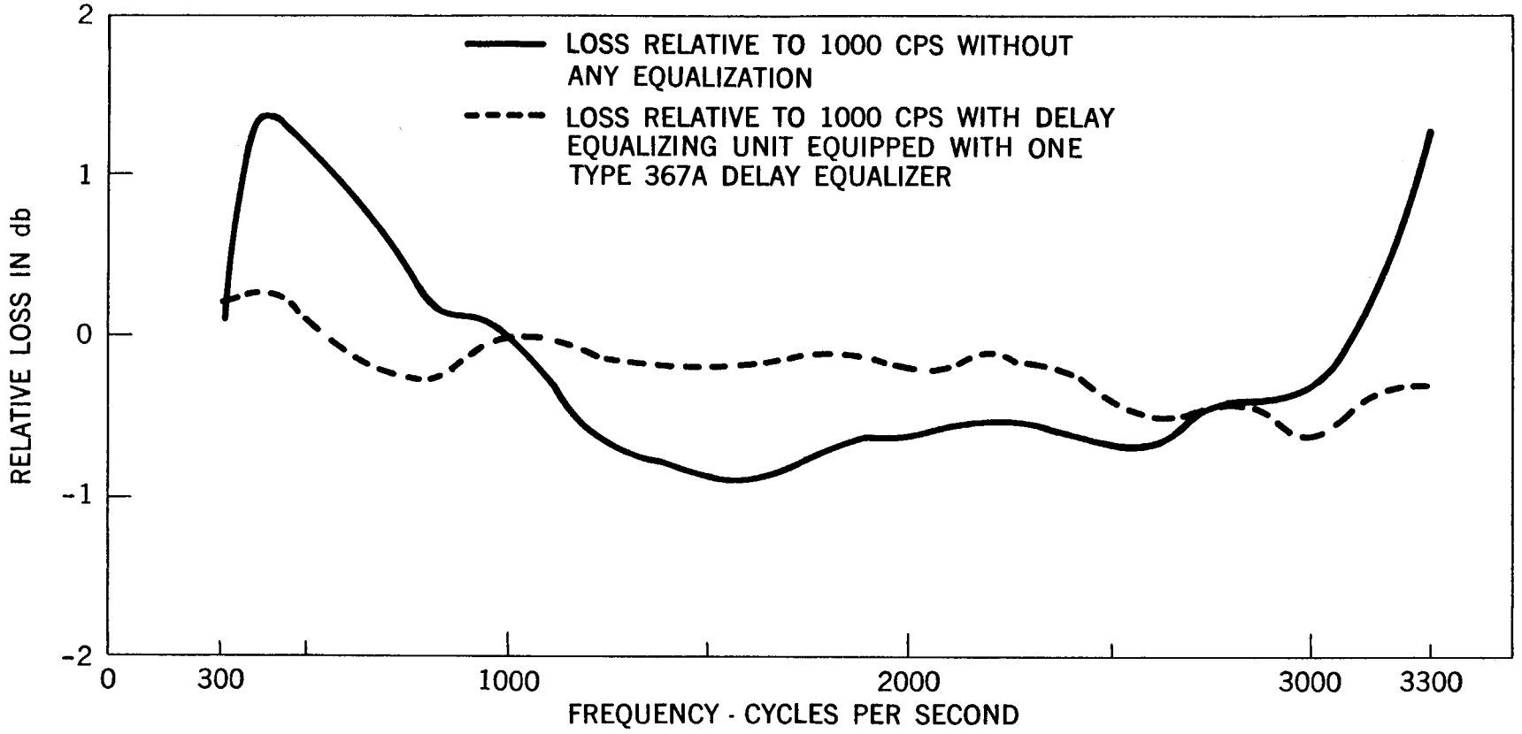
Fig. 8 - Relative Loss of Typical L Multiplex Circuit
