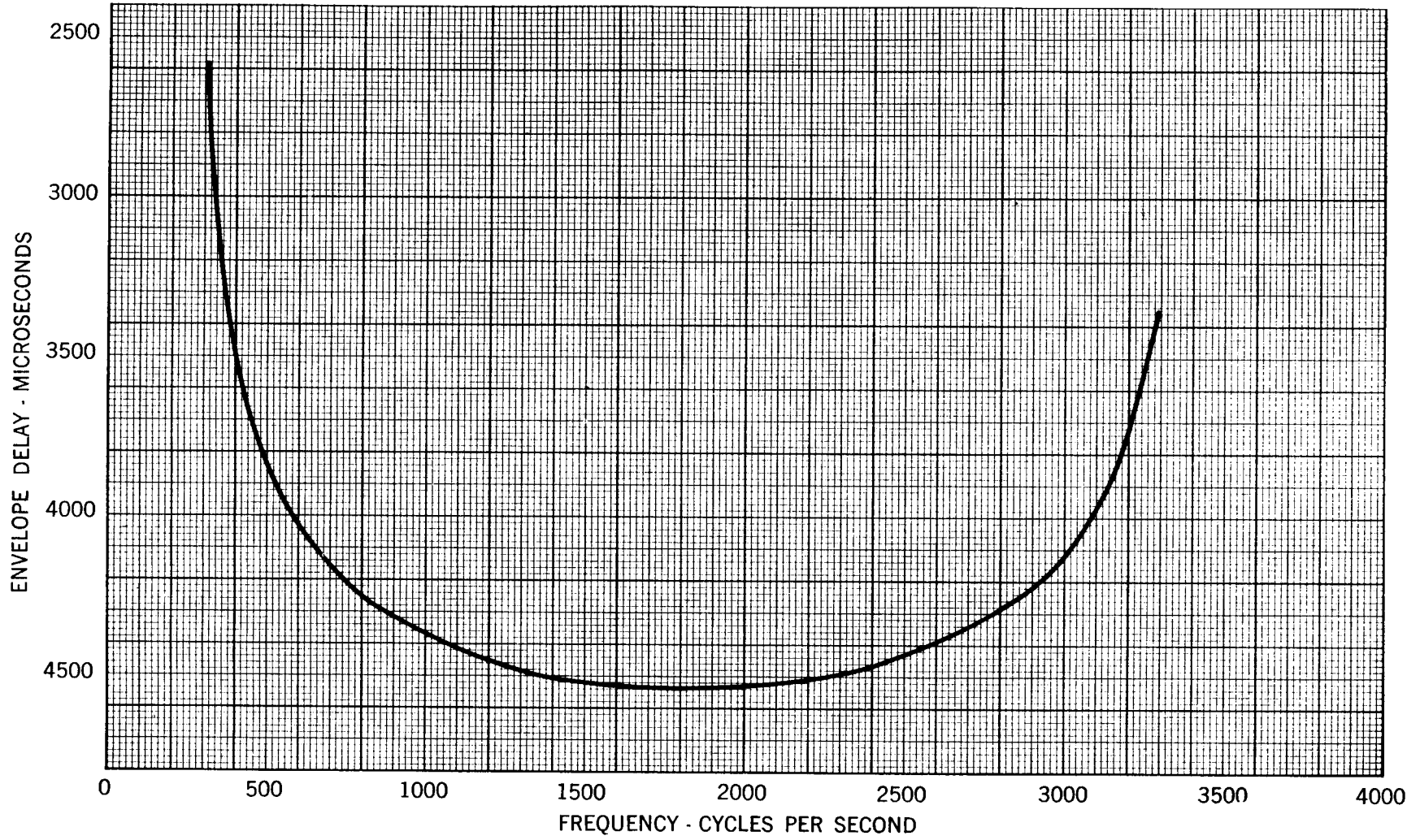
Fig. 4 – Nominal Envelope Delay Characteristic of 366A Equalizer
