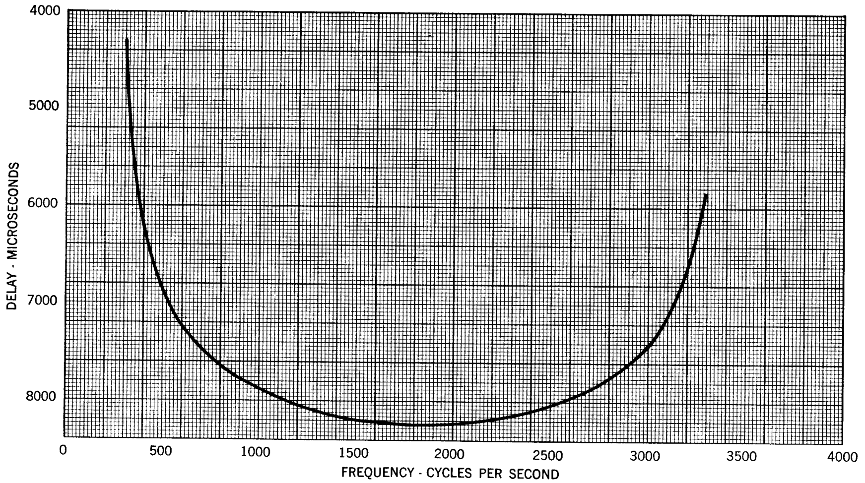
Fig. 7 – Nominal Envelope Delay Characteristic of 367A Equalizer
